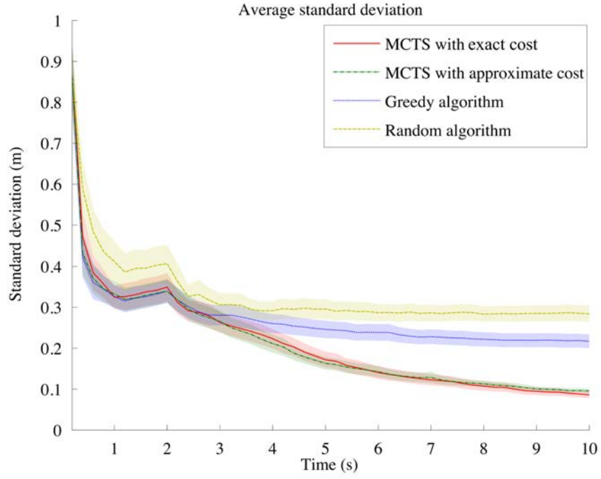
Figure 5.11: Average standard deviation and 95% confidence interval over time with the standard deviation criterion of the 4 algorithms over all 200 experiments.
