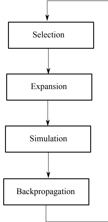
Figure 5.1: The four main steps in an iteration of the MCTS algorithm.
