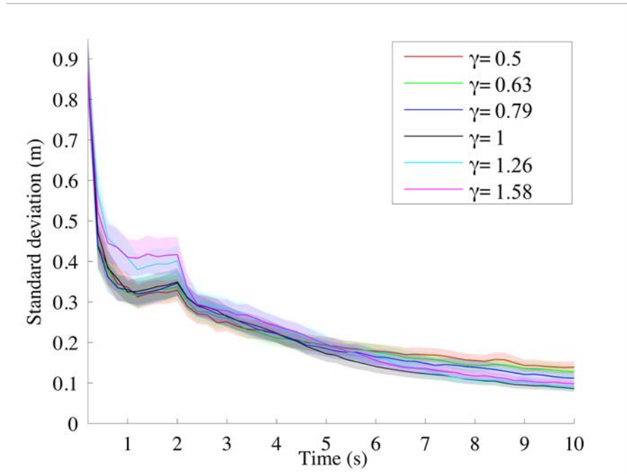
Figure 5.18: Average standard deviation and 95% confidence interval over time with different discount factor values for the standard deviation criterion.
