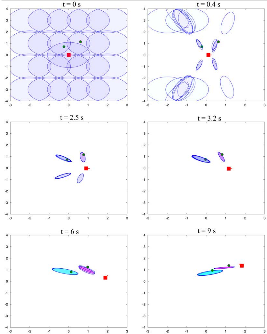
Figure 4.1: Visualization of our extended MKF with the JPDAF in an example of localizing two sources. Robot positions are shown as red squares, and the actual source positions as green circles. Blue and pink ellipses represent 95% confidence regions of source location estimation of various hypotheses in the mixture with a transparency proportional to the weight of the components.
