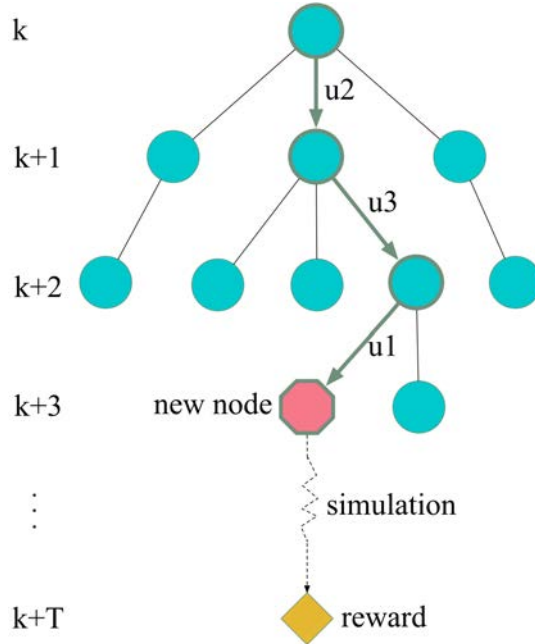
Figure 5.2: An iteration of the MCTS algorithm.
