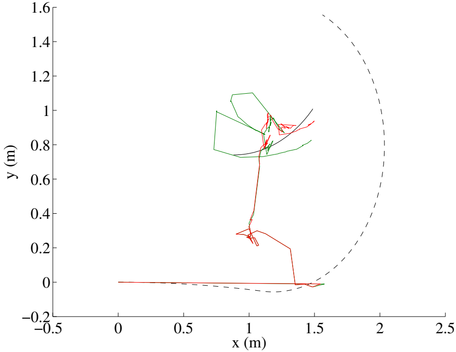
Figure 3.5: Estimated trajectories of the two extended MKF methods in the example run. Dashed black line: trajectory of the robot, Solid black line: ground truth trajectory of the sound source, Green line: estimate of the extended MKF without activity model, Red line: estimate of our extended MKF with activity model.
