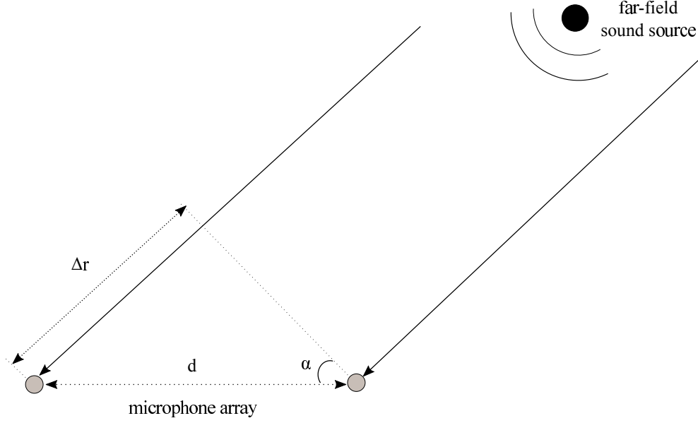
Figure 2.4: AoA computation in the far-field.
