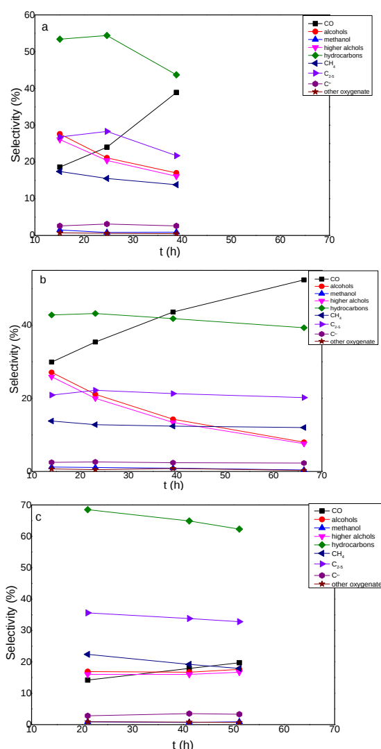
Figure 70 The change of selectivities to products with time with (a) 0.5K30CuFeCNTs, (b) 1.5K30CuFeCNTs, (c) 1Cs30CuFeCNTs
