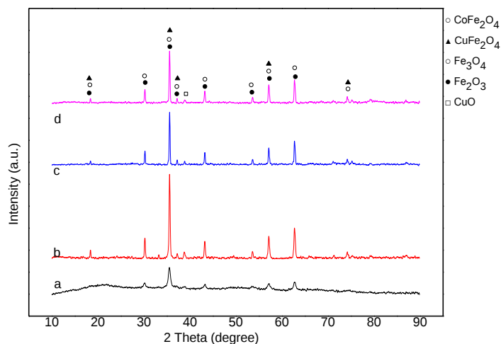
Figure 29 Room temperature XRD patterns of CuCoFe-precursor after calcination at different temperatures: (a) 400 °C, (b) 600 °C, (c) 800 °C, (d) 1000 °C
