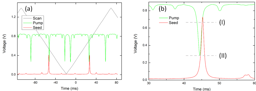
Figure 4.9: (a) Responses of the OPO cavity to the pump and seed when the cavity is scanned with a triangle waveform from a function generator. (b) The peaks for the pump and seed when the phase-matching temperature is optimized. I and II denote the threshold levels for switching to the locking mode.
