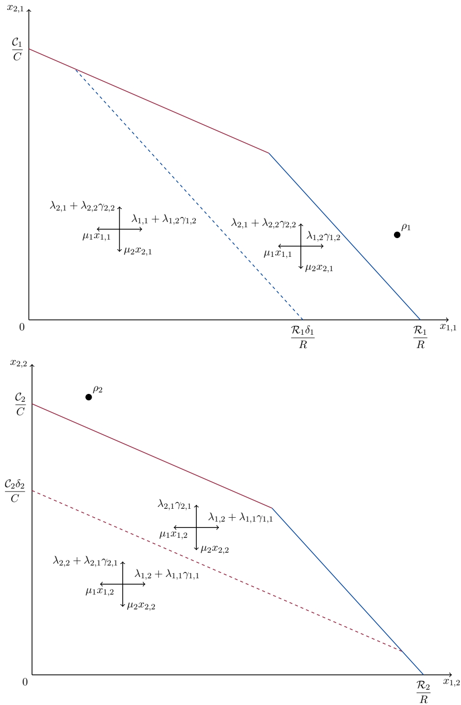
Figure 3.4 – Transitions of threshold forwarding policy
