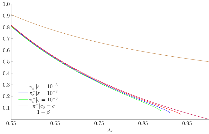
Figure 2.4 – Fraction of jobs served at requested bit-rate at equilibrium for the downgrading policy compared to the fraction of lost jobs in a pure loss system.
