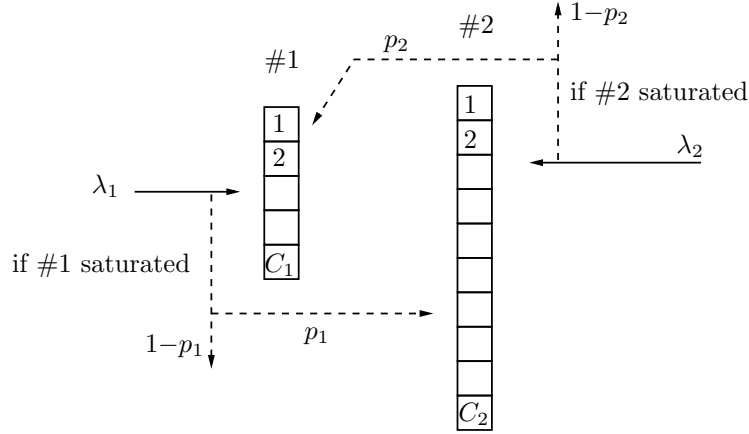
Figure 4.2 – Load Balancing between Two Data Centres
