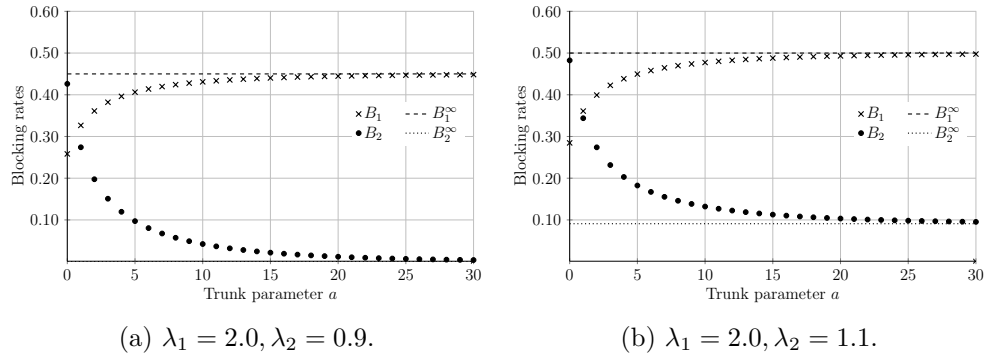
Figure 5.3 – Blocking probabilities in both data centres with same size as a function of a , with c = (1.0, 1.0) and \mu = (1.0, 1.0)
