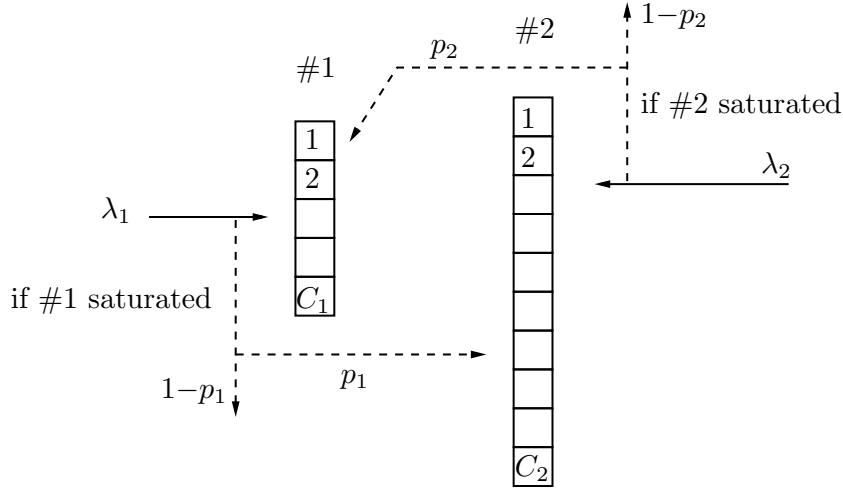
Figure 1.8 – System configuration ("probabilistic" Offloading)
