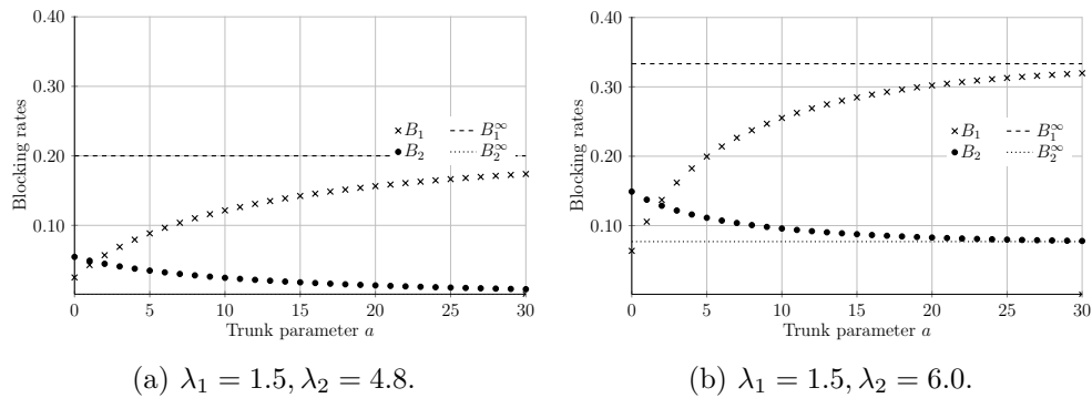
Figure 5.4 – Blocking probabilities in both data centres with different sizes as a function of a , with c = (1.0, 5.0) and \mu = (1.0, 1.0)
