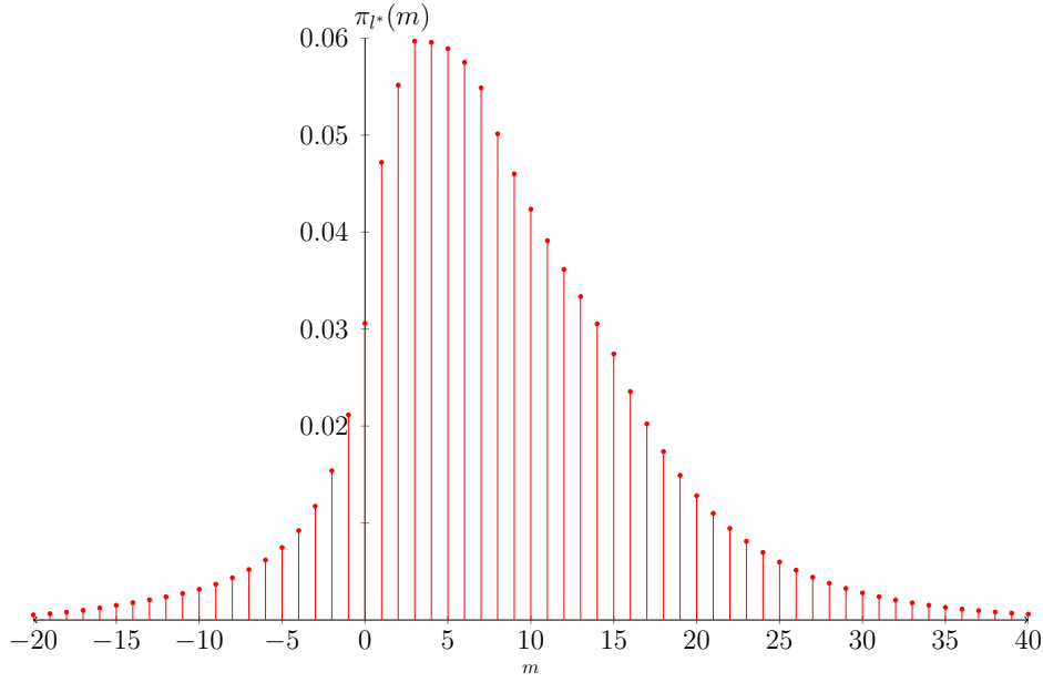
Figure 2.1 – The histogram of Y_{\ell^*} with the parameters J = 5 , A = (1, 2, 4, 8, 16) , \lambda = (0.25, 0.2, 0.15, 0.1, 0.05) , \mu = (1, 1, 1, 1, 1) and c_0 = 0.97 .
