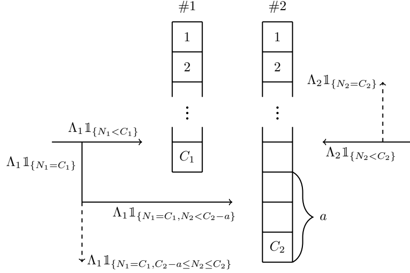
Figure 5.1 – Policy implementation scheme
