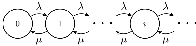
Figure 1.3 – Transition diagram of the M/M/1 Queue
