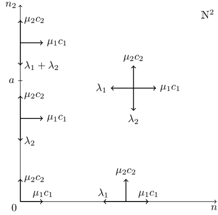
Figure 5.2 – Transitions for (n(t)) .
