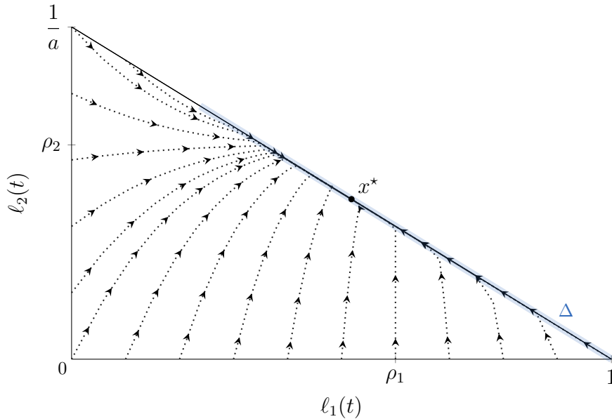
Figure 1.6 – Limiting sample paths of an overloaded loss system The Equilibrium point x^* is determined in Equation (1.5). Note that if l(t_0) \in \Delta , for some t_0 \geq 0 , then l(t) \in \Delta for any t > t_0 .
