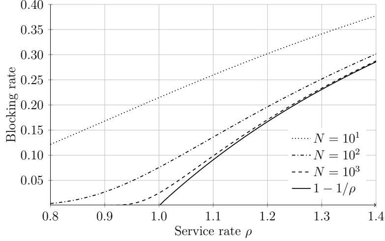
Figure 1.5 – Exact Erlang Formula and Large Scale Approximation
