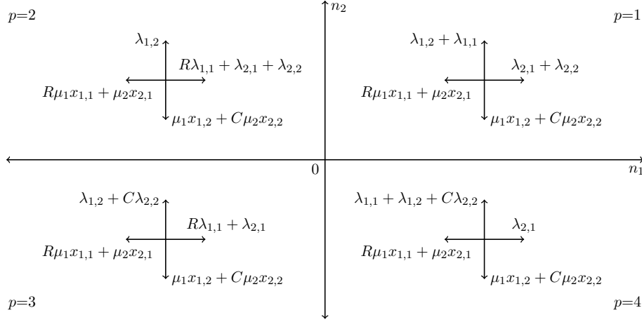
Figure 3.2 – Drifts on the quarter planes of \mathbb{Z}^2
