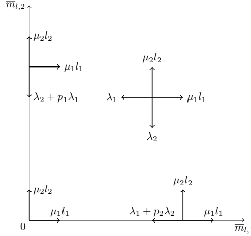
Figure 4.3 – Transitions for \bar{m}_i(t) .
