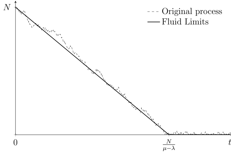
Figure 1.4 – Fluid limits of the M/M/1 queue
