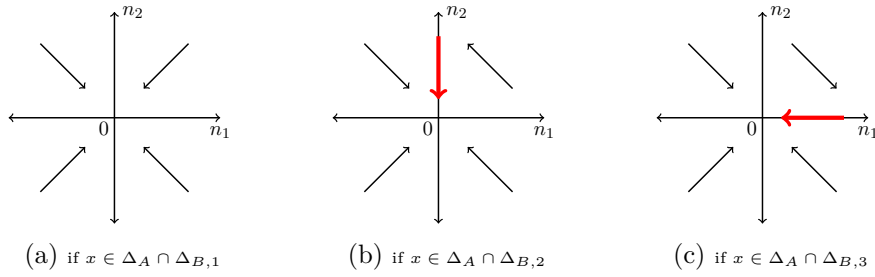
Figure 3.3 – Resulting drifts of the fluids limits associated with (U_x(t)) .
