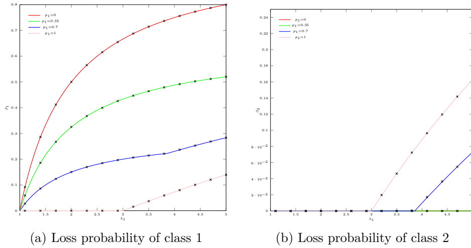
Figure 4.4 – Loss probabilities as a function of \lambda_1 with \lambda_2 = 8 , c_1 = 1 , c_2 = 10 , \mu_1 = 1 , \mu_2 = 1 , p_2 = 0 . The crosses represent simulation points while solid curves are plotted from analytical results.
