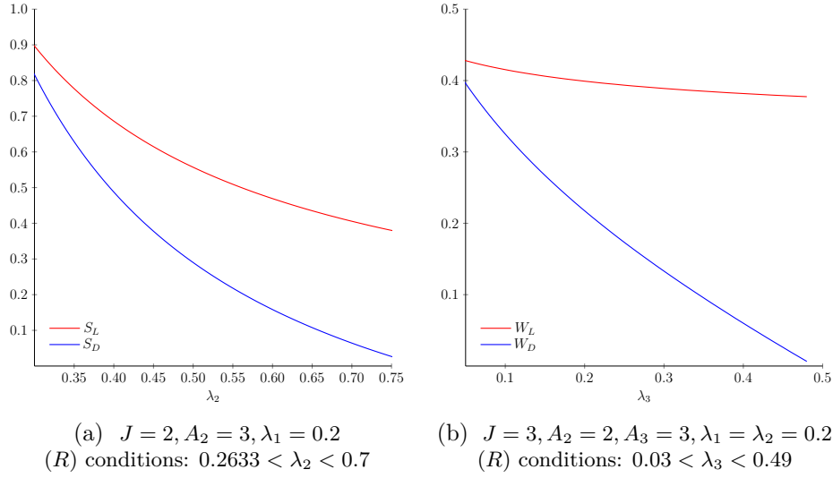
Figure 2.2 – Comparison between policies
