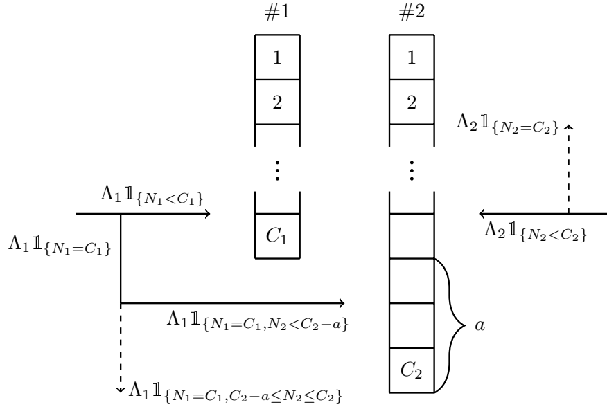
Figure 1.9 – System configuration (“truncated” offloading)
