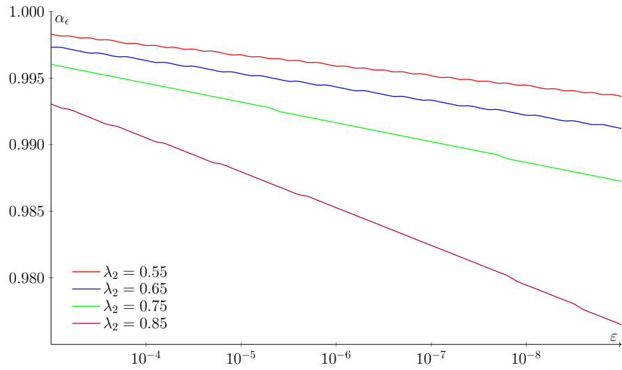
Figure 2.3 – Maximal threshold for a loss probability equal to \epsilon .
