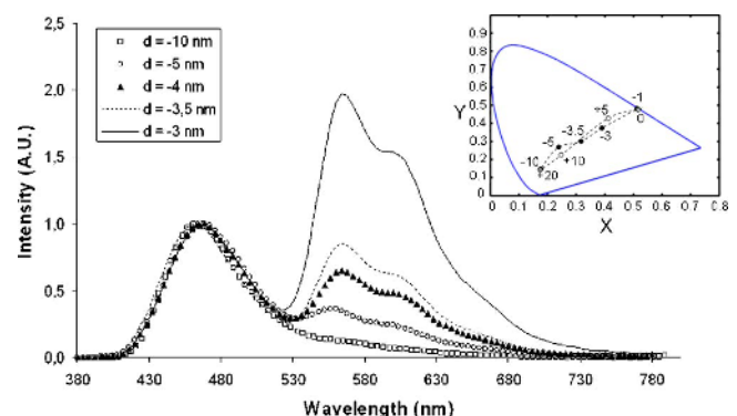
FIG. 3. (Color online) Electroluminescence spectra for different positions of rubrene in the NPB (the DPVBi side is similar but was not plotted for clarity). Inset: corresponding CIE diagram; filled circles stand for DPVBi side (the values of d (in nm) are written near each circle) and open circles stand for NPB side. The dotted line is a guide to the eye.
