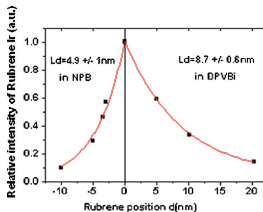
FIG. 4. (Color online) Relative rubrene intensity for different positions in NPB and DPVBi. The dots show the experimental data, and the line fits the exponential decay.
