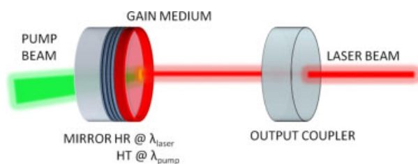
Figure 10. Schematic of a VEC SOL. 121 The left-hand mirror is highly transparent (HT) for the pump wavelength and highly reflective (HR) for the laser radiation. The radius of curvature and reflectivity of the output coupler are optimized to yield the highest output energy in a single transverse mode.
