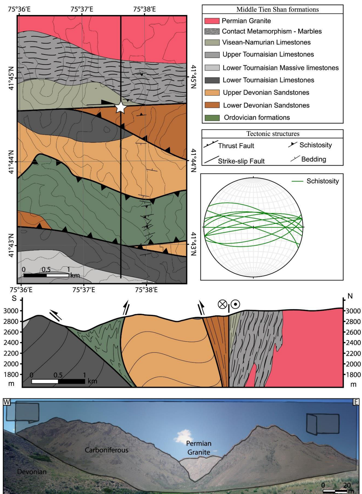
Figure 8 : Geological map and cross-section of the East Son-Kul area. The thick black line indicates the cross-section location. Star indicates the picture location. The stereoplot shows the projection, in Schmidt diagram lower hemisphere, of the schistosity measured in this zone. The picture shows the vertical dextral fault considered as the trace of the Nikolaev Line at the surface.
