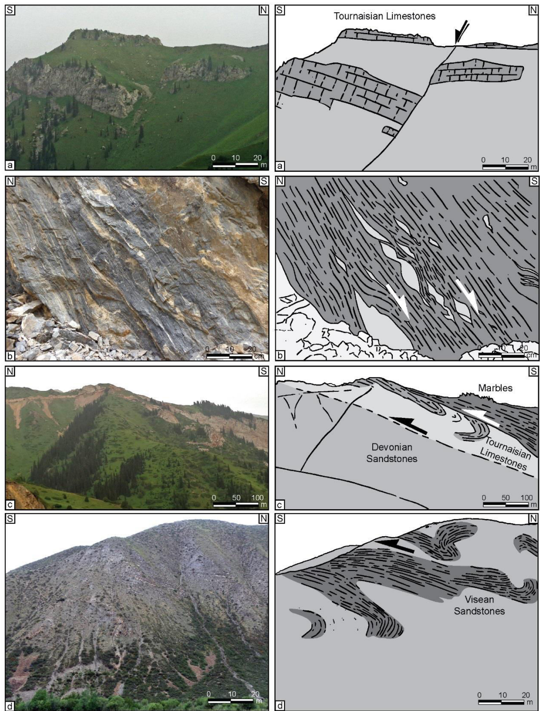
Figure 7 : Field pictures and their interpretations of the Lake Song Kul area. a. Normal fault in Carboniferous platform carbonates (Tournaisian) of the MTS; b. Deformed marbles with asymmetric top to the SW ductile shearing; c. Top to the North thrusting of the marbles on Tournaisian MTS carbonate platform and Devonian sediments; d. Southward overturned folds in Visean pelites and sandstones. Fig. 6 displays the location of pictures.
