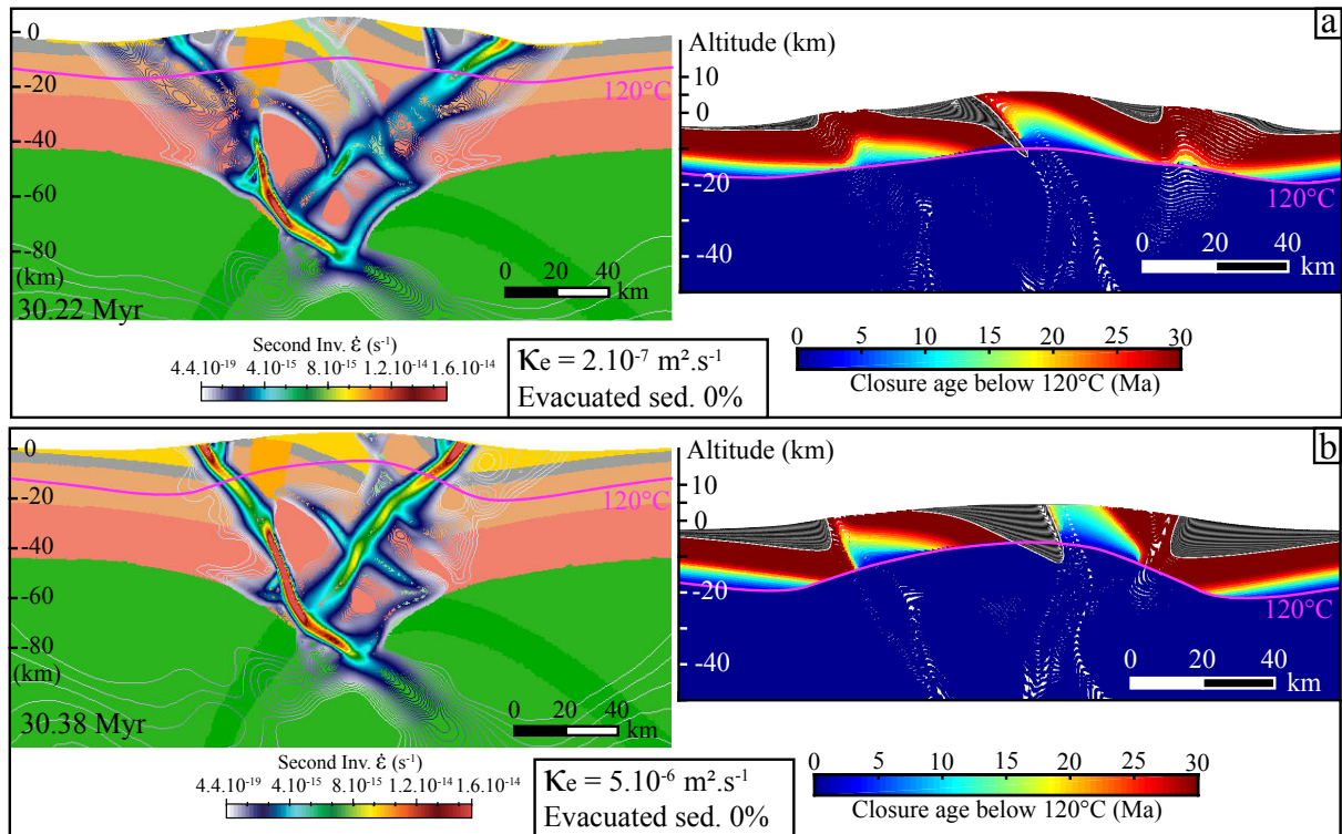
Figure 3: Final time step of two models with diffusion coefficient of a) 2.10^{-7} \text{ m}^2.\text{s}^{-1} and b) 5.10^{-6} \text{ m}^2.\text{s}^{-1} and no outward sediments fluxes. On the left, isolines represent the second invariant of the strain rate tensor. On the right, colours represent the age of exhumation at temperatures lower than the 120°C isotherm (purple line). Sedimentary basins are represented with stratigraphic layering of 1 Ma.
