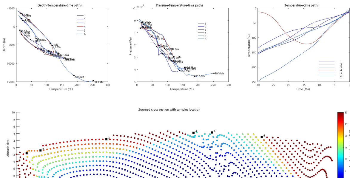
Figure 6: final figure obtained at the end of the P_T_tfromPtatin script. A Depth-Temperature-time path (corner left), a Pressure-Temperature-time path (central), a Temperature-time path (corner right) are obtained as well as a cross section indicating the exhumation age of the points in the simulation on which the clicked points are represented.
