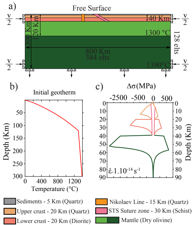
Figure 2: Models setup. a) Rheological phases and boundary conditions, v = 0.5 mm/a. b) Initial geotherm for all models. c) Yield strength envelope of the ductile flow laws of quartz (brown), diorite (salmon pink), schists (pink) and olivine (green) for a strain rate of 1.10^{-14} s^{-1} .
