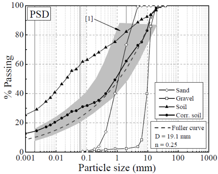
FIGURE 4.1: PSD of soil before and after correction [SOS+14]
