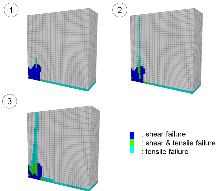
FIGURE 4.13: Evolution of the plasticity states in a simulated pushover tests using CJS-RE1 at different computation stages
