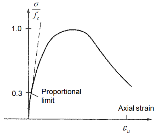
FIGURE 1.9: Typical compressive stress-strain curve for concrete [Che07]
