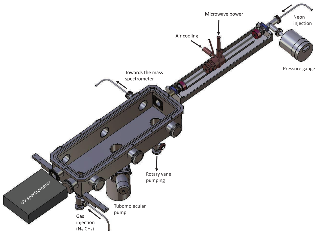
Figure 2. Scheme of the photochemical reactor coupled windowlessly with the VUV source.
