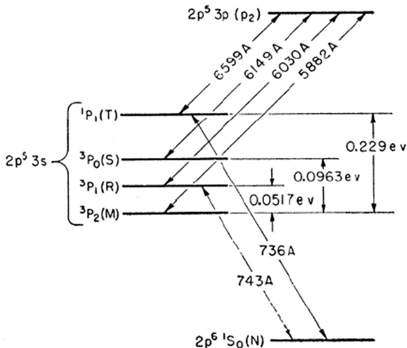
Figure 10. Gotrian diagram of the neon energy levels. Reprinted with permission from (Phelps 1959). Copyright 1959 by the American Physical Society.
