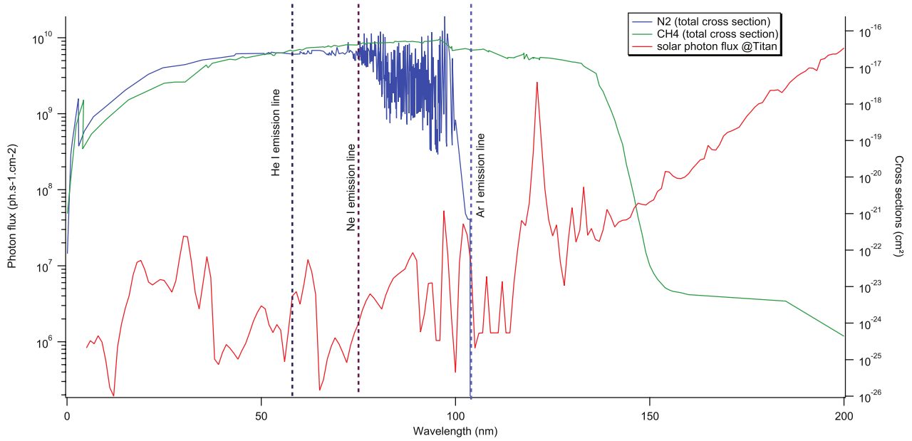
Figure 1. VUV absorption cross sections of N 2 (blue) and CH 4 (green), and the VUV solar spectrum at Titan (red). The dotted vertical lines show the VUV emission lines of the three rare gases He I, Ne I, Ar I.
