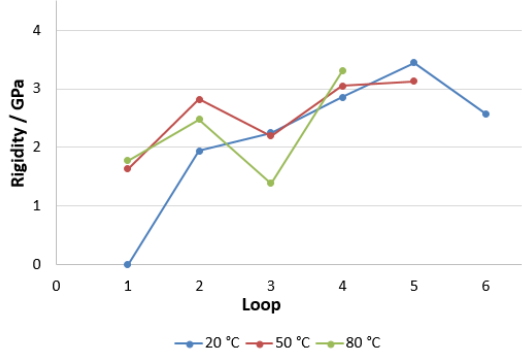
(b) Difference of secant modulus between load and reload at different temperature
