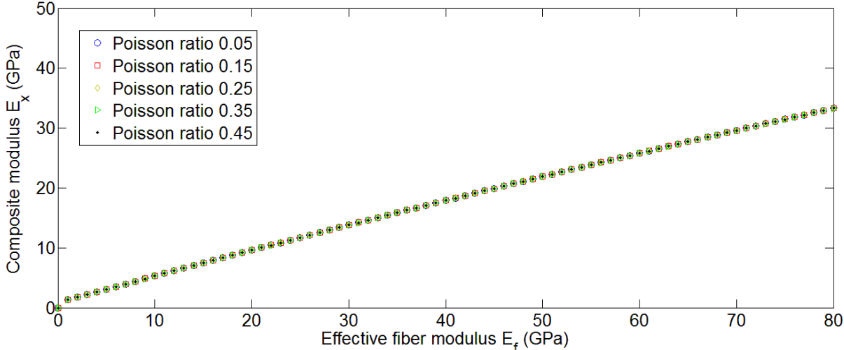
Fig. 3.14 Effect of flax fiber Poisson’s ratio on the computed longitudinal composite modulus
