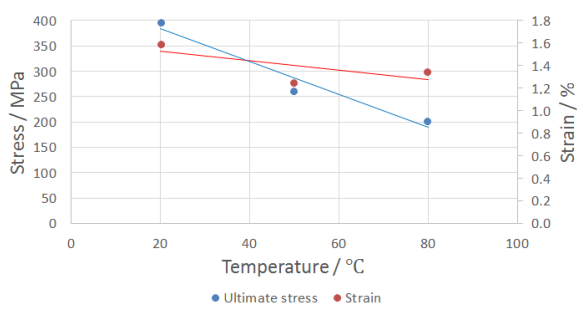
(b) Evolution of ultimate stress and strain
