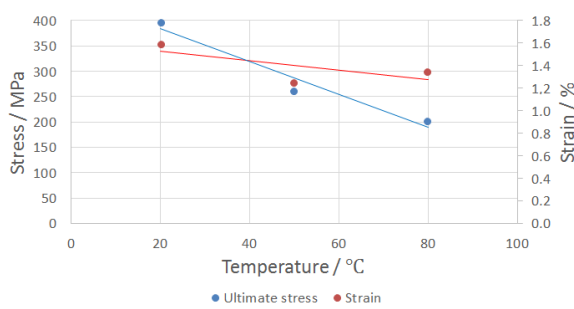
(b) Evolution of ultimate stress and strain
