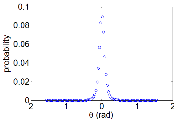
Fig. 3.18 Best orientation distribution function of UD flax ply with a surface density of 78 \text{ g m}^{-2}
