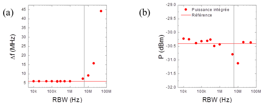
Fig. 2.7-Signal characteristic of a Lorentzian signal of \Delta f=6\text{ MHz} and P=-30.5\text{ dBm} generated by signal generator with different RBW used for the measurement with the SA: (a) \Delta f versus RBW and (b) power versus RBW. Adapted from [76].
