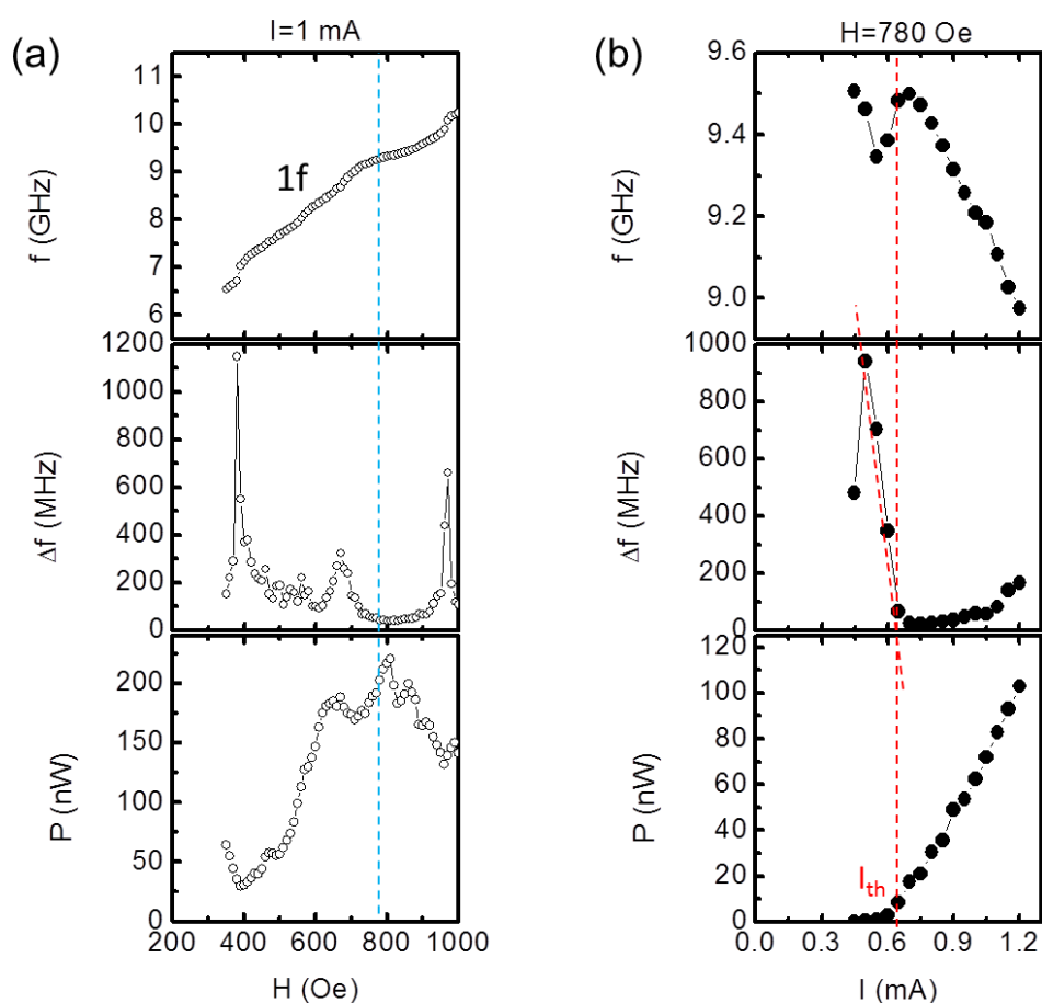
Fig. 4.48-(a) The frequency, linewidth, and the output power of the first harmonic excitation as a function of applied magnetic field for a fixed applied DC current I_{\text{DC}}=1 mA. (b) The frequency, linewidth, and the output power of the first harmonic excitation as a function of applied DC current for a fixed applied magnetic field H_{\text{DC}}=780 Oe.
