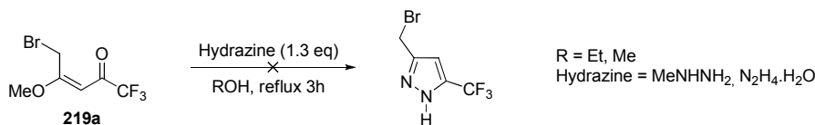
Scheme 4.50 : Attempts of cyclisation of the brominated fluoroenone 219a
