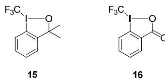
Figure 2.5: Togni's trifluoromethyl transfer reagents
