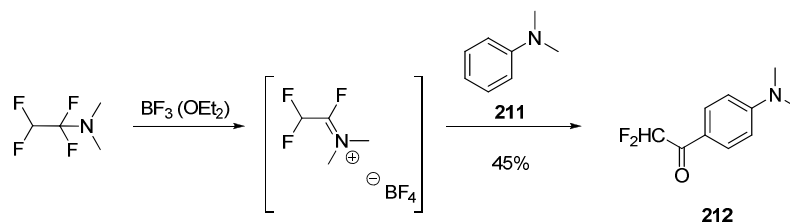
Scheme 4.43 : Acylation of aromatic substrates
