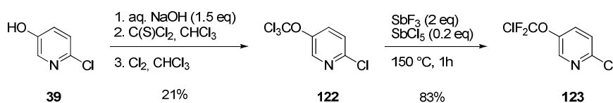
Scheme 3.12: Fluorination of the trichloromethoxy pyridine 122 with SbF 3
