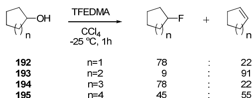
Scheme 4.33 : Fluorination of cyclic alcohols
