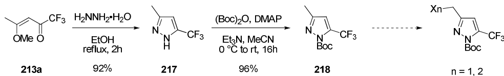
Scheme 4.47 : Synthesis of N -Boc pyrazole 218 from 213a
