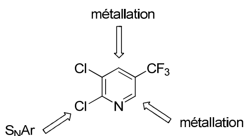
Figure 6: "Magic Pyridine" 12
