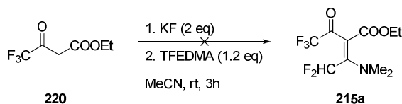
Scheme 4.51 : Reaction of ethyl trifluoroacetoacetate 220 with TFEDMA
