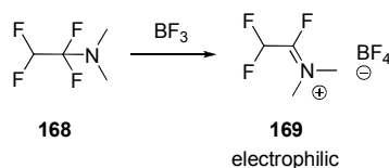
Scheme 4.22: Activation of TFEDMA
