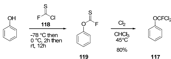
Scheme 3.9: Chlorination of fluorothionoformate 119
