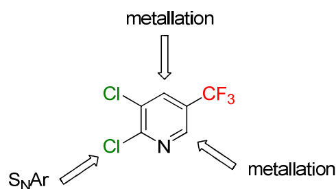
Figure 2.8: Magic Pyridine 61
