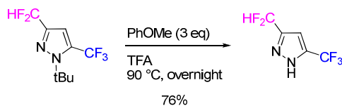
Scheme 5.5: Deprotection of N - tert -butyl 3-CHF 2 -5-CF 3 pyrazole
