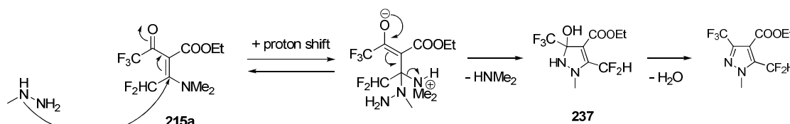
Figure 4.12: Mechanism of the Michael-addition of \text{-NHMe} onto the adduct
