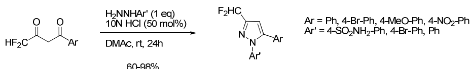
Scheme 4.4 : Influence of acidic medium on the regiochemistry
