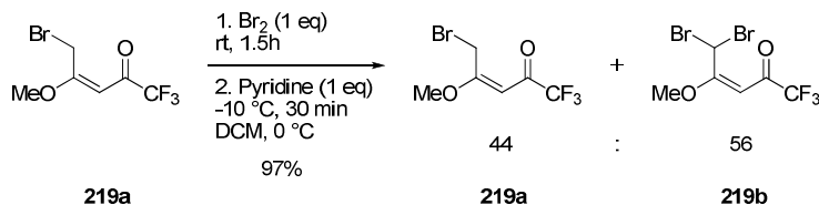
Scheme 4.49 : Attempt of bromination of the brominated fluoroenone 219a
