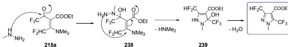
Figure 4.13: Mechanism of the attack of \text{-NHMe} onto the trifluoromethyl carbonyl
