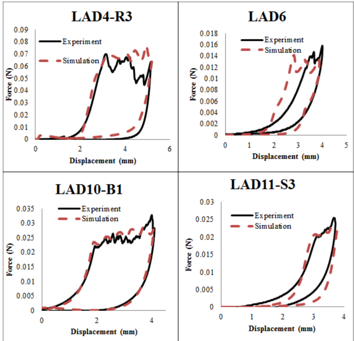
Figure 2.8: Experimental versus simulation curves obtained with the minimum cost value, for samples dissected through the intima
