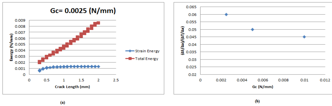
Figure 5.1: (a) Example of the strain energy and the total energy curves vs crack length, for G_c = 0.0025\text{ N/mm} (b) the average ratio of (\Delta S/\Delta a) / (\Delta T/\Delta a) vs. G_c values
