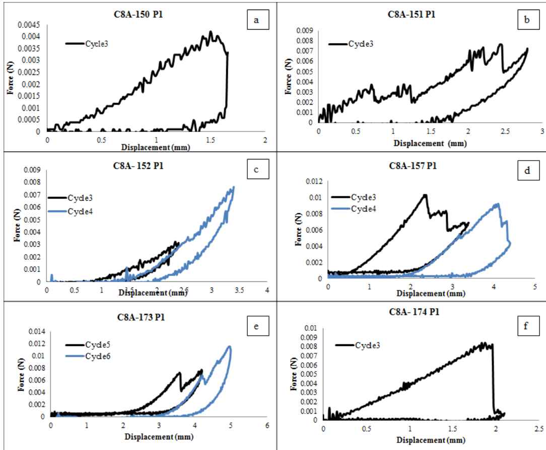
Figure 5.3: Force vs Displacement curves obtained experimentally for 6 plaques tested from the ApoE -/- Col8 -/- mouse group
