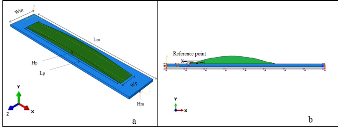
Figure 3.4 : Schematic representation of the plaque model and the underlying aorta. (a): L_m represents the aortic media length, L_p the plaque length, W_m the medial width, W_p the plaque width, H_m the medial height and H_p the maximum plaque height ( L_m not shown to scale); (b): 2D representation of the atherosclerotic plaque (green) attached by cohesive elements to the underlying aorta (blue), lying on the gray rigid surface (S). The bottom edge of S, the left & right edges of (A+S), and the top left edge of A were clamped to simulate experimental testing conditions. The reference point represents the master node where displacement boundary conditions were applied.
