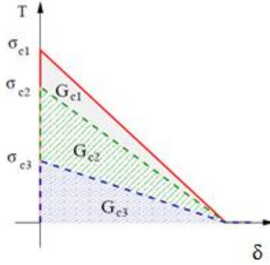
Figure 1.6: Set of cohesive laws considered in the model used in Ferrara et al. 2010
