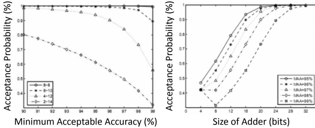
Figure 1.32 – ETAI accuracy simulation results [35]
