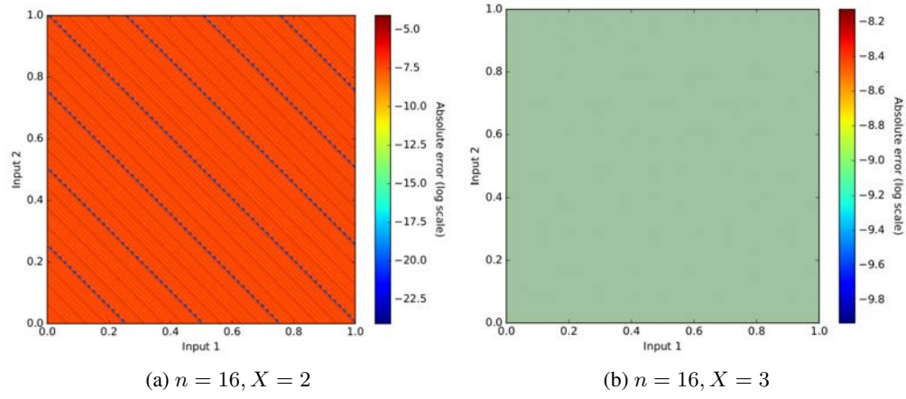
Figure 1.36 – Error maps of 16-bit ETAIV for different values of X
