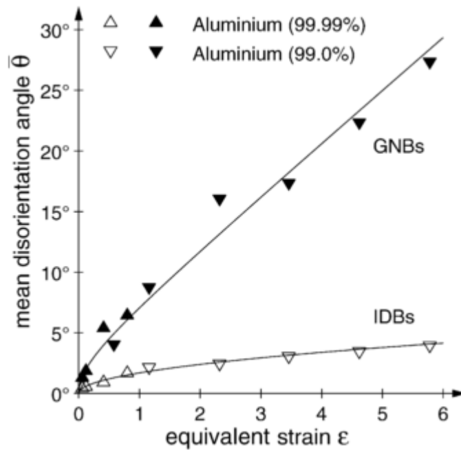
Figure 1.10 – Evolution of the mean disorientation angle across the boundaries (both GNB and IDB) during cold-rolling, for two different Aluminium alloys (99.99% and 99%) [15].
