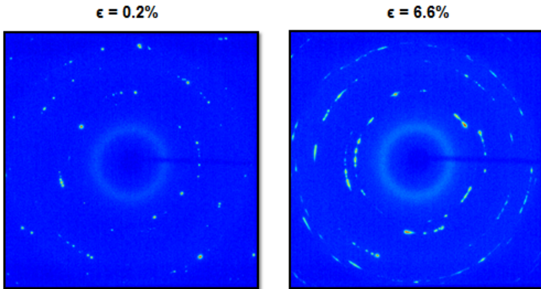
Figure 3.1 – Comparison between two diffraction frames recorded at the strain levels of \epsilon = 0.2\% and \epsilon = 6.6\% and at the same rocking angle \omega = 0^\circ . Diffraction spots are very narrow at \epsilon = 0.2\% and broaden along the \eta direction when increasing the strain.
