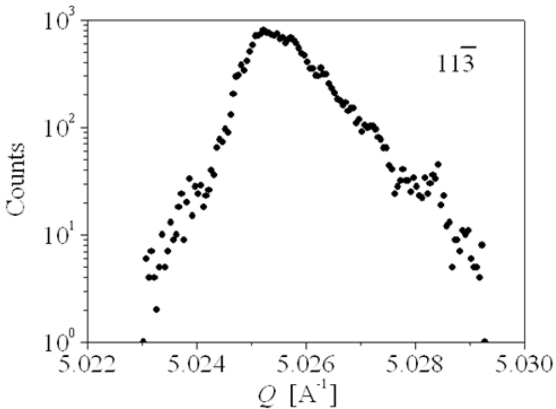
Figure 5.5 – Distribution of diffraction vector lengths |\vec{Q}_{113}| (line profile).
