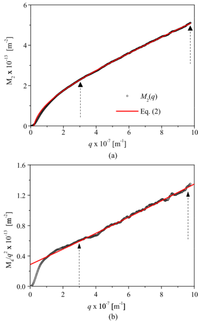
Figure 1.19 – Plots of (a) second order moment and (b) fourth order moment of a X-Ray diffraction peak for a deformed copper ( \epsilon = 0.15 ). Arrows indicate the considered q interval for the fit. [31].
