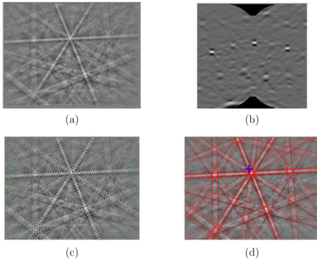
Figure 2.11 – Determination of an orientation. (a) Kikuchi diagram, (b) Hough transform, (c) Kikuchi bands detection, (d) orientation indexation [57].
