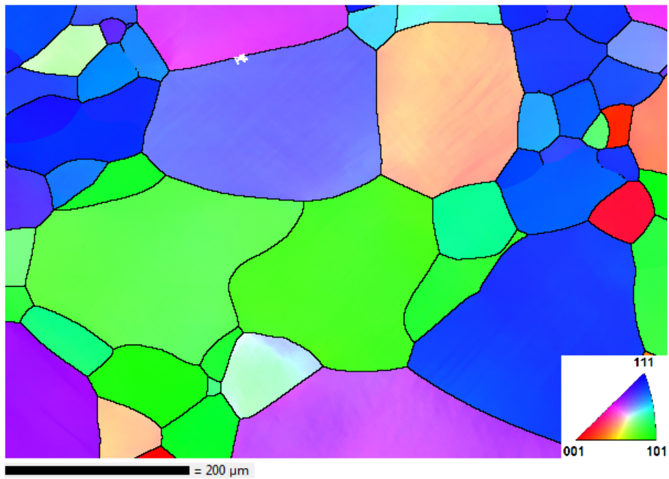
Figure 6.2 – IPF colour map of Specimen B deformed at \varepsilon = 5\% .
