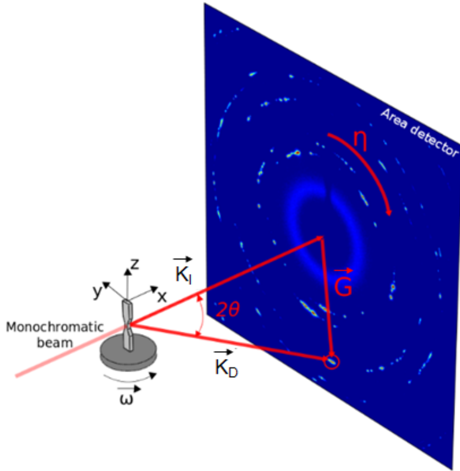
Figure 2.2 – Sketch of the 3DXRD setup for the case of an incoming monochromatic X-Ray beam. The Bragg angle 2\theta , the rotation angle \omega and the azimuthal angle \eta are indicated, as well as the laboratory coordinate system centred on the sample. Diffraction spots coming from different grains of the polycrystalline sample appear onto the 2D detector, arranged along the Debye-Scherrer rings.
