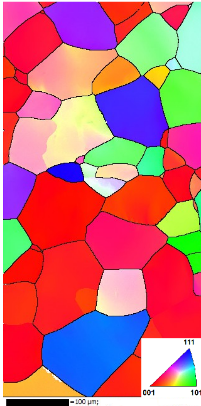
Figure 6.1 – IPF colour map of Specimen A deformed at \varepsilon = 5\% .
