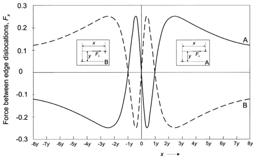
Figure 1.6 – Variation of F_x with dislocation relative position. The full curve A is relative to dislocations of the same type, the broken curve B to unlike dislocations [6].
