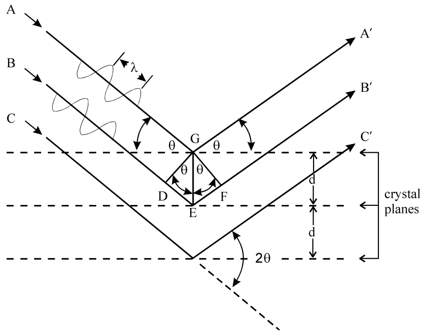
Figure 2.5 – Schematic representation of the Bragg law. The line DEF indicates the difference between the optical paths of the waves A and B: if this quantity equals the wavelength of the monochromatic beam, the interference is constructive with the rise of the diffraction phenomenon.
