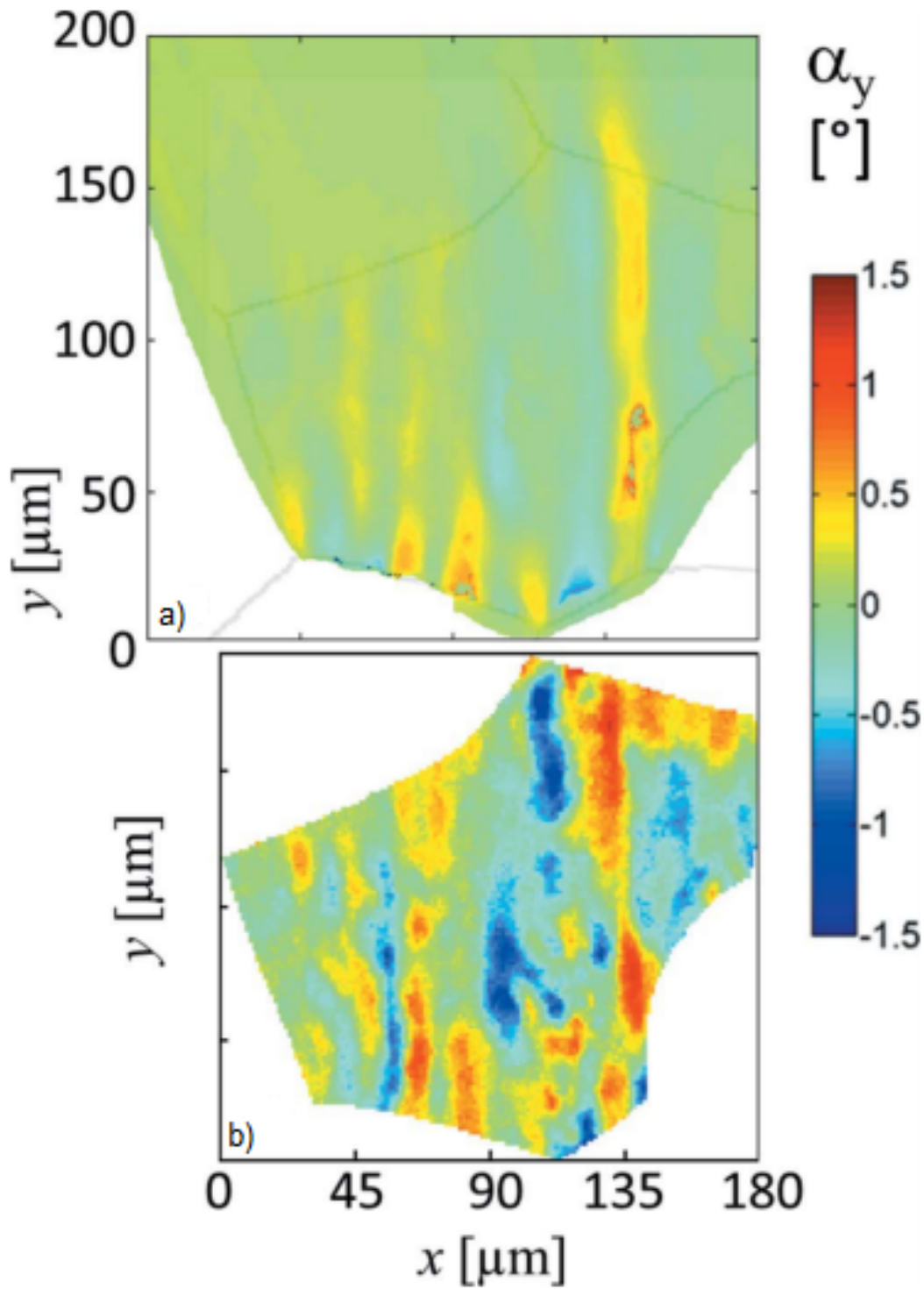
Figure 5.1 – Distribution of the O_y component of lattice tilt \alpha_y (the angle between the local Q_y component and the average value of \vec{Q}_{11\bar{3}} over all pixels) calculated from a) K-map rocking curves and b) EBSD.
