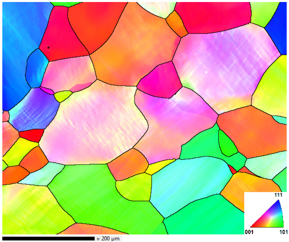
Figure 6.3 – IPF colour map of Specimen C deformed at \varepsilon = 10\% .
