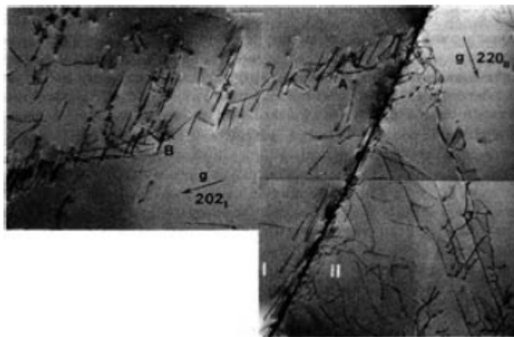
Figure 1.22 – Transmission Electron Microscope image of a dislocation pile-up in the vicinity of a grain boundary [37].
