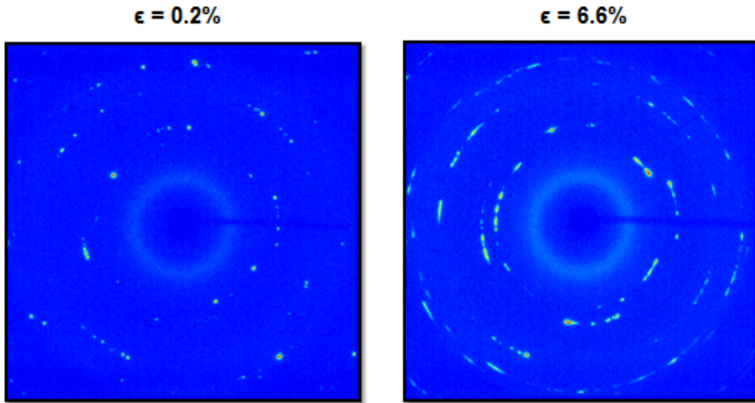
Figure 3.1 – Comparison between two diffraction frames recorded at the strain levels of \varepsilon = 0.2\% and \varepsilon = 6.6\% and at the same rocking angle \omega = 0^\circ . Diffraction spots are very narrow at \varepsilon = 0.2\% and broaden along the \eta direction when increasing the strain.
