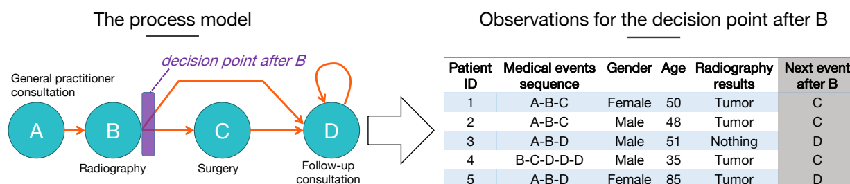
Figure 4.5: Example of a ready-for-classification log for a single decision point
