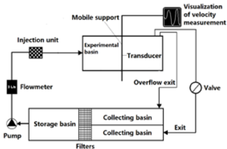
Figure 4.1 Experimental tank
