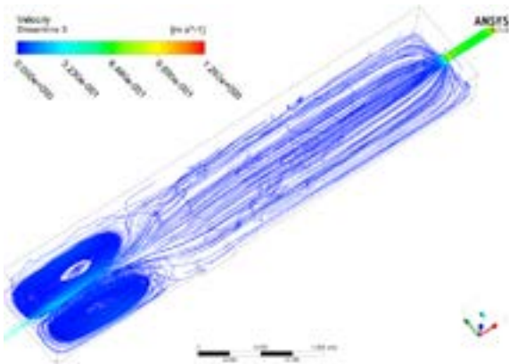
Figure 2.100 3D streamlines at volume flow rate 2 L/s
