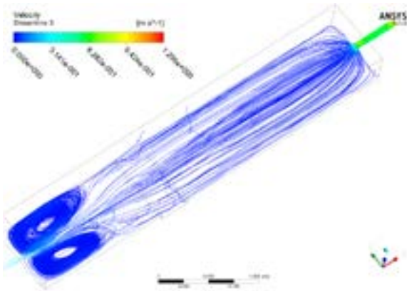
Figure 2.98 3D streamlines at volume flow rate 2.5 L/s
