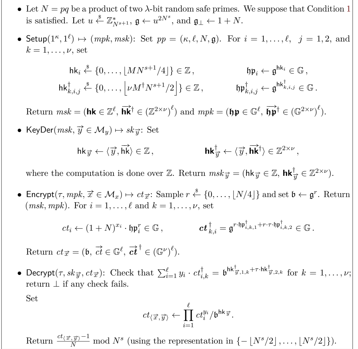
Figure 7.2: DCR-based tag-based inner-product functional encryption secure against chosen-ciphertext attacks
