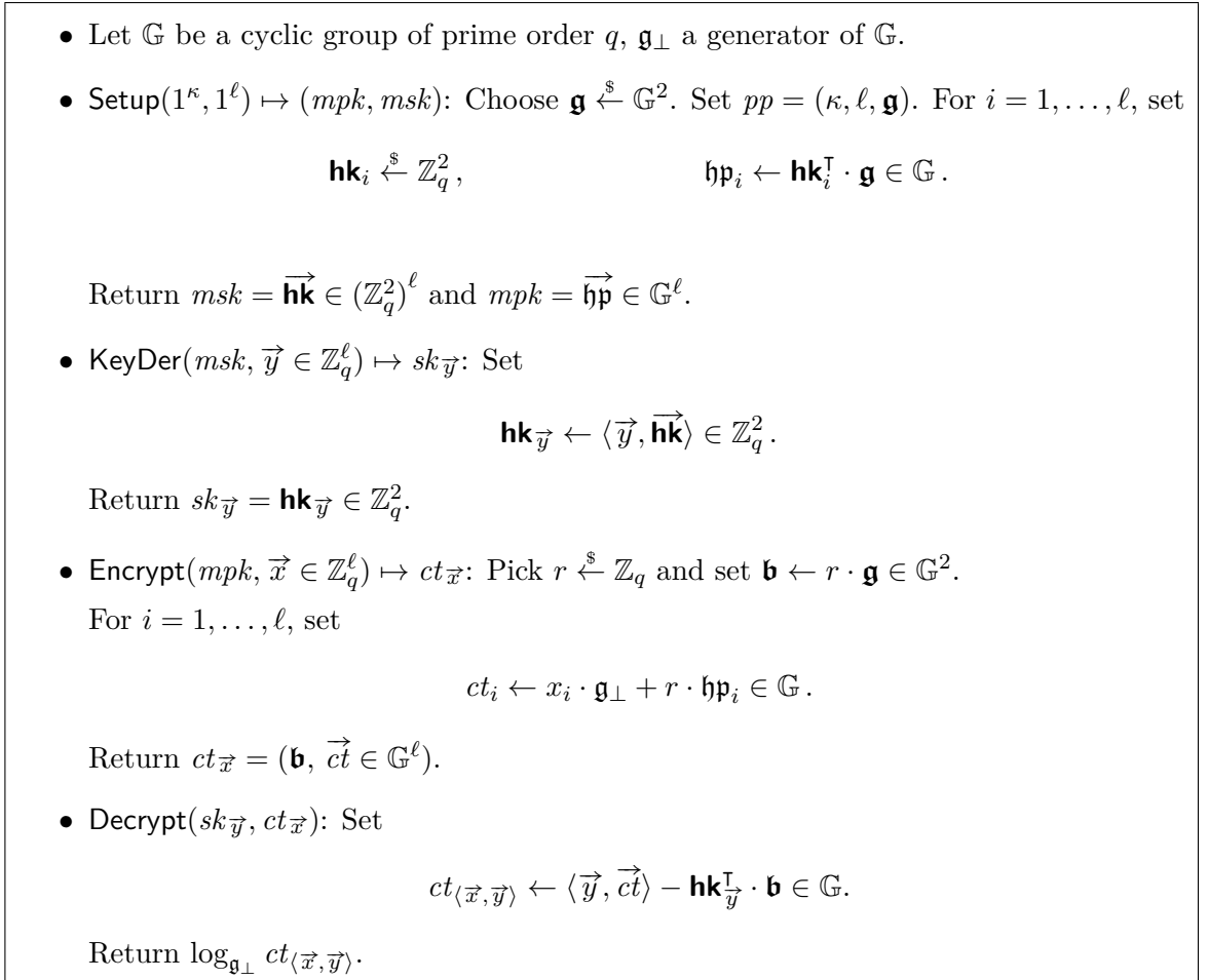
Figure 6.2: DDH-based inner-product functional encryption secure against chosen-plaintext attacks
