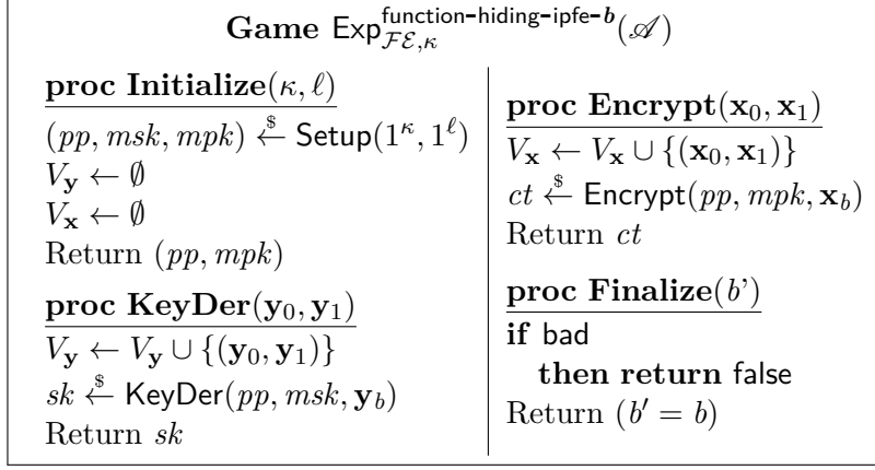
Figure 3.9: Game \text{Exp}_{\mathcal{FE}, \kappa}^{\text{function-hiding-ipfe-}b}(\mathcal{A}) defines function hiding of \mathcal{FE} . The event bad corresponds to \exists(y_0, y_1) \in V_y, \exists(x_0, x_1) \in V_x, \langle x_0, y_0 \rangle \neq \langle x_1, y_1 \rangle .
