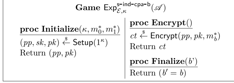
Figure 2.1: Game \text{Exp}_{\mathcal{E}, \kappa}^{\text{s-ind-cpa-b}}(\mathcal{A}) defines s-IND-CPA security of \mathcal{E} .
