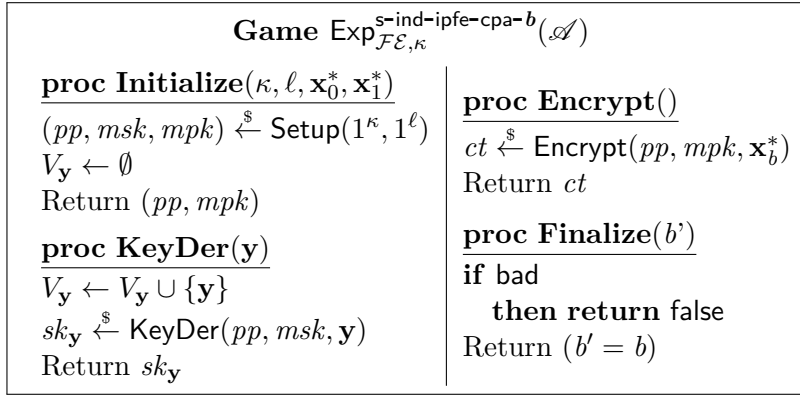
Figure 3.4: Game \text{Exp}_{\mathcal{FE}, \kappa}^{\text{s-ind-ipfe-cpa-}b}(\mathcal{A}) defines s-IND-IPFE-CPA security of \mathcal{FE} . The event bad corresponds to \exists \mathbf{y} \in V_y, \langle \mathbf{x}_0^*, \mathbf{y} \rangle \neq \langle \mathbf{x}_1^*, \mathbf{y} \rangle .
