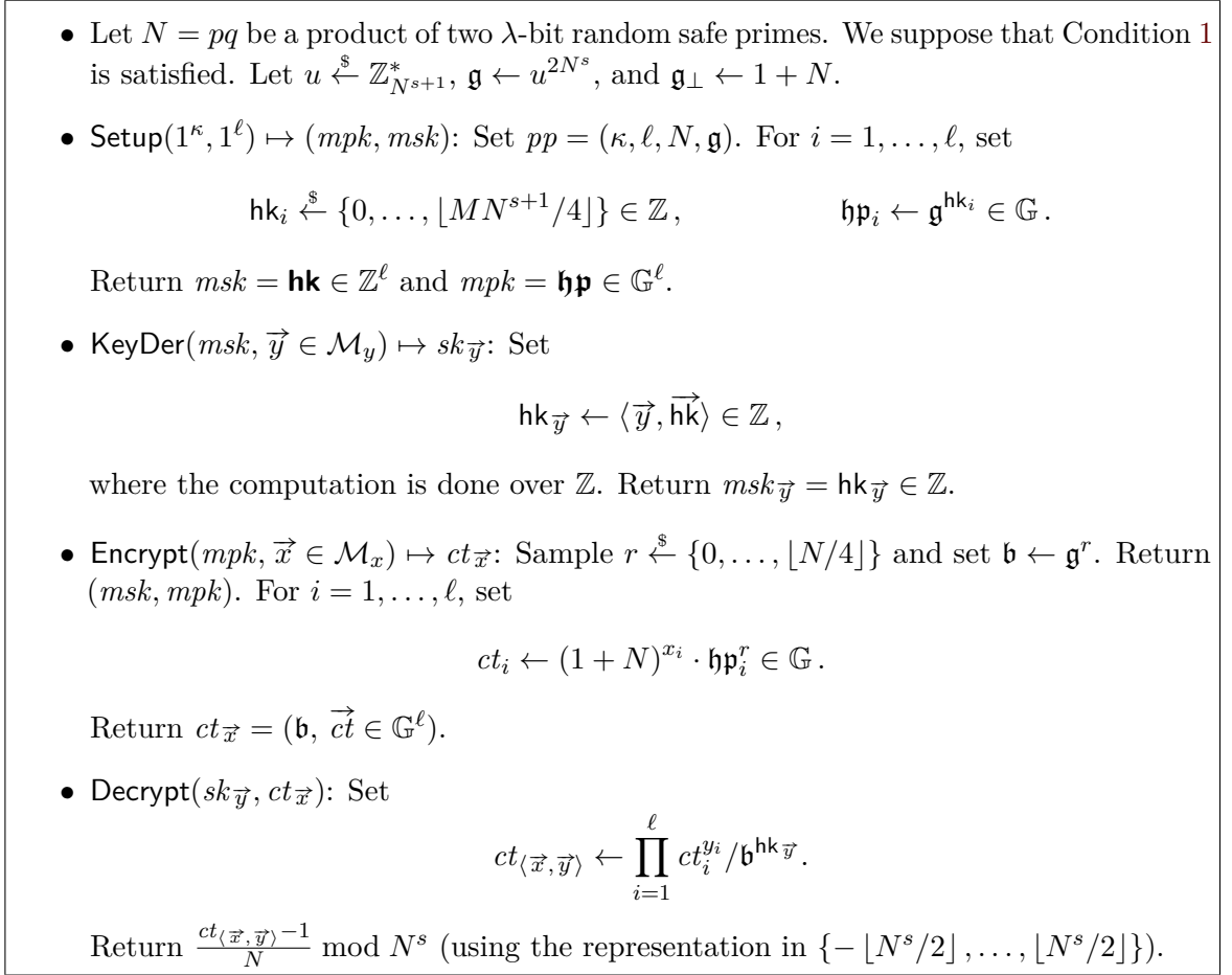
Figure 7.1: DCR-based inner-product functional encryption secure against chosen-plaintext attacks
