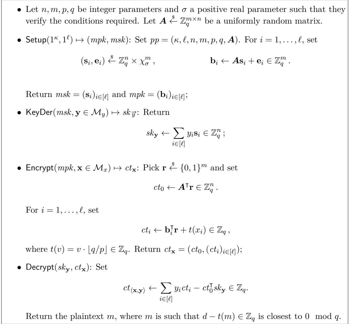
Figure 8.1: LWE-based inner-product functional encryption secure against selective chosen-plaintext attacks
