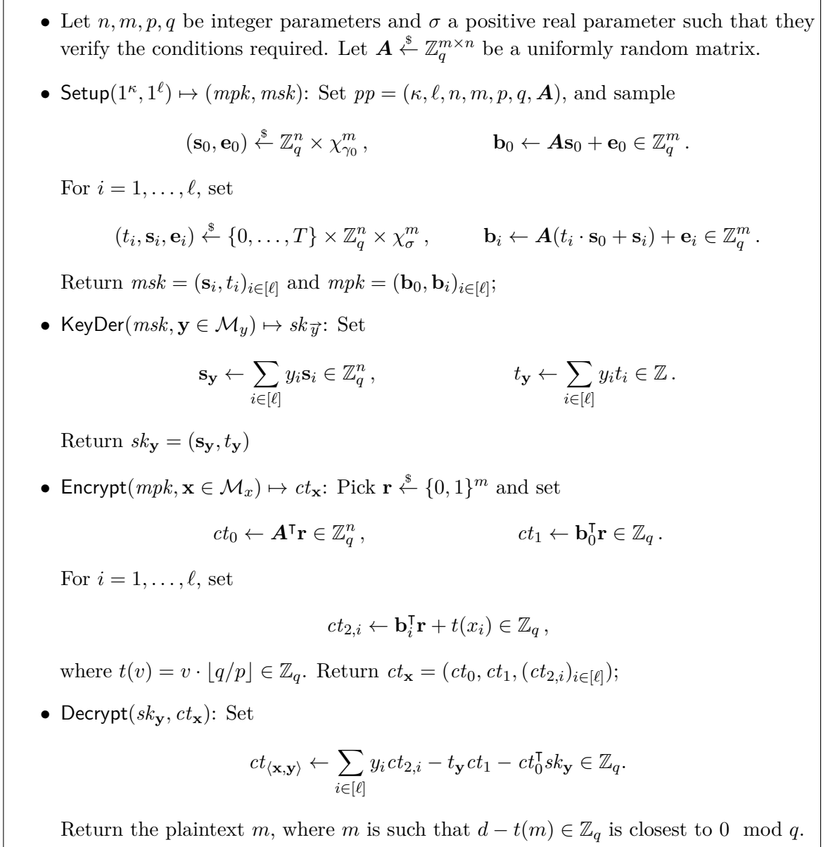
Figure 8.2: LWE-based inner-product functional encryption secure against adaptive chosen-plaintext attacks
