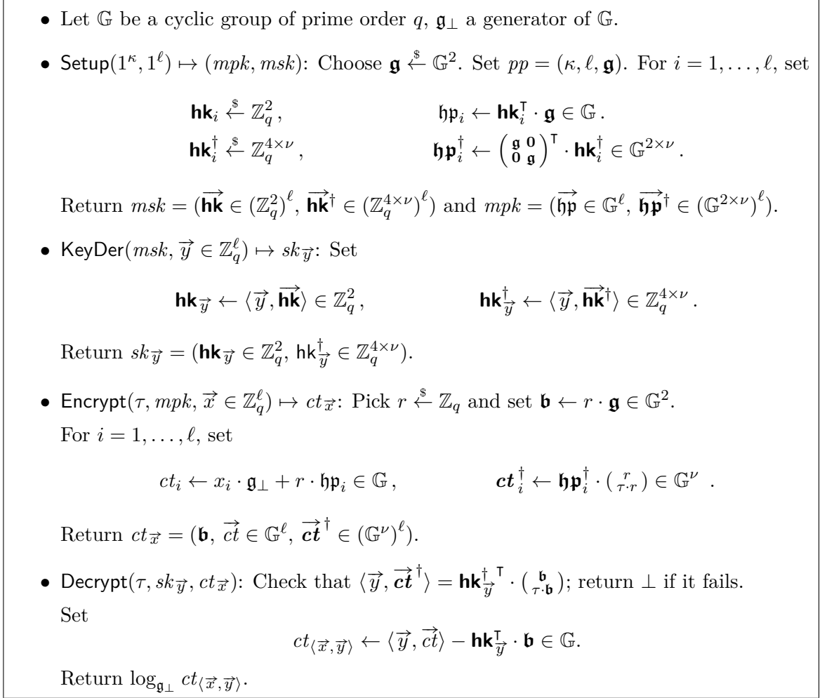
Figure 6.3: DDH-based tag-based inner-product functional encryption secure against chosen-ciphertext attacks
