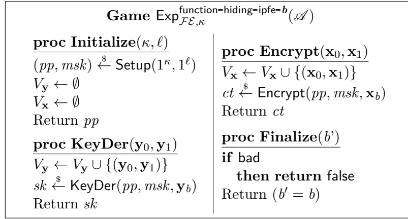
Figure 3.10: Game \text{Exp}_{\mathcal{FE}, \kappa}^{\text{function-hiding-ipfe-b}}(\mathcal{A}) defines function hiding of \mathcal{FE} . The event bad corresponds to \exists(\mathbf{y}_0, \mathbf{y}_1) \in V_y, \exists(\mathbf{x}_0, \mathbf{x}_1) \in V_x, \langle \mathbf{x}_0, \mathbf{y}_0 \rangle \neq \langle \mathbf{x}_1, \mathbf{y}_1 \rangle .
