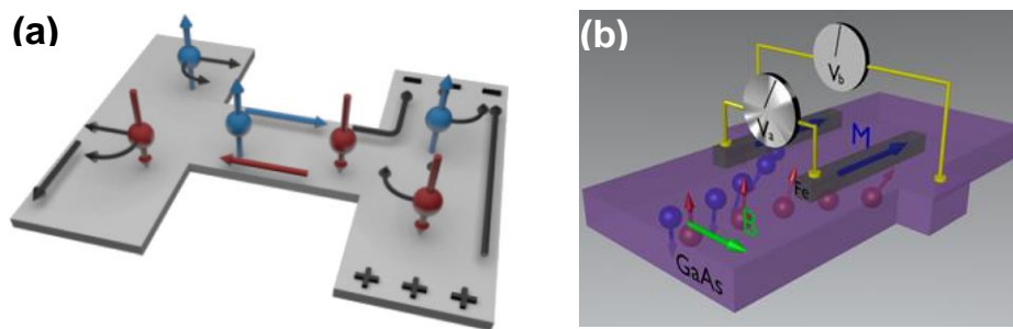
Fig. I. 14: (a) Principle of the H -based device (from ref. 84): A charge current is applied in the left hand wire (the black arrow), creating a spin current in the bridge. This spin current is then converted into a charge current by ISHE which can be measured by a voltmeter along the right hand wire (black arrow). (b) Principle of the SHE detection device proposed by Garlid et al. in ref. 127: Two thin Fe electrodes are laid along the (In)GaAs Hall cross. Firstly, the magnetizations in the Fe-electrodes is initialized in the anti-parallel or in the parallel states. The charge current is applied along the semiconductor wire to create the spin accumulations of the perpendicular-polarization by SHE in (In)GaAs. An in-plane field B is applied perpendicularly to the Fe-electrodes to induce the precession of the spin accumulation. The spin signal is the measured voltage V_a - V_b . V_b is used as a reference, to eliminate parasitic effects such as the normal Hall contribution due to the stray-field.
