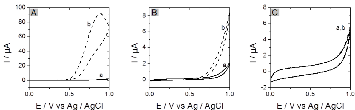
Figure 2.8. (A) Cyclic voltammograms recorded at a potential scan rate of 20 \text{ mV s}^{-1} using a bare GC electrode in 0.1 \text{ M} Tris-HCl buffer (pH 9.0) (a) in the absence and (b) in the presence of 1 \text{ mM} NADH. (B) Cyclic voltammograms recorded in the same conditions as in A but using this time a vinylphenyl functionalized GC electrode (a) in the absence and (b) in the presence of 1 \text{ mM} NADH. (C) Cyclic voltammograms recorded at a potential scan rate of 100 \text{ mV s}^{-1} using CysI-DSDH functionalized GC electrode in 0.1 \text{ M} Tris-HCl buffer (pH 9.0) containing 1.8 \text{ mM} \text{NAD}^+ (a) in the absence and (b) in the presence of 1 \text{ mM} D-sorbitol. The geometric surface area of the electrode was 0.28 \text{ cm}^2 .
