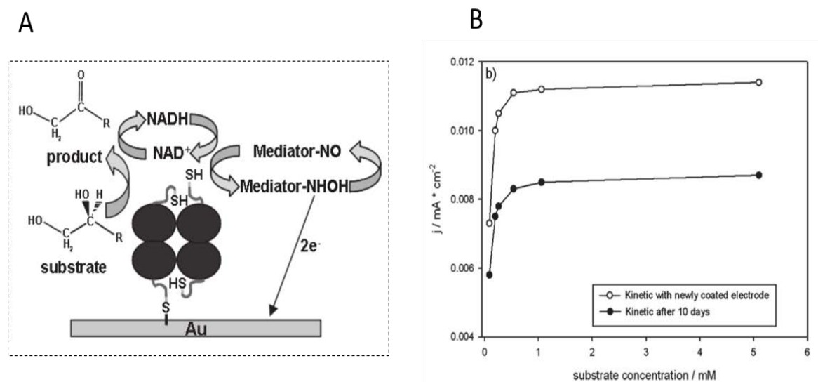
Figure 1.7. (A) Schematic principle of the immobilization of the cysteine-modified GatDH with electrochemical NAD + regeneration for enzymatic synthesis of hydroxyacetone; (B) Michaelis-Menten plots of the current at +500 mV vs the substrate concentrations for GatDH-immobilized electrode before and after 10 days [77].
