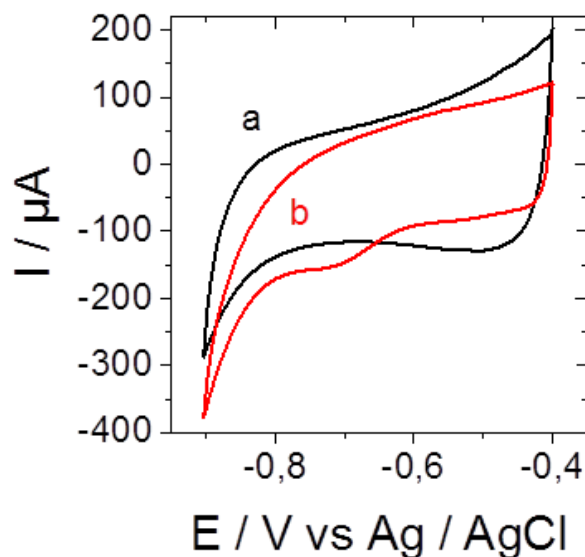
Figure 3.7. Cyclic voltammograms of the bipyridine immobilized electrode (CF-CNT-4'4-Bpy) (a) before and (b) after complexation with ((\text{RhCp}^*\text{Cl}_2)_2) . Experiment was carried out in 50mM PBS (pH6.5) under nitrogen. Scanning rate is 5 \text{ mV s}^{-1} . The geometric surface area of the electrode was 0.25 \text{ cm}^2 .
