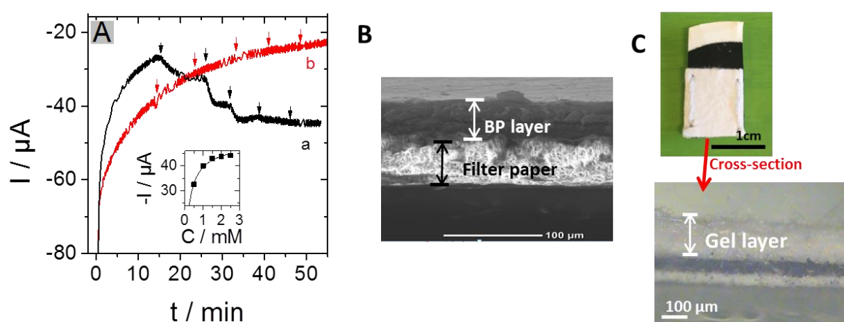
Figure 5.9. (A) Amperometric response to gradual addition of 0.5 mM D-fructose recorded using a combined electrode (1 cm * 1 cm) of (a) separate BP-Bpy-Rh and DSDH gel layer (b) separate BP-Bpy-Rh and blank gel layer in 50 mM PBS (pH 6.5) with the presence of 1 mM NADH at an applied potential of -0.72 V under nitrogen. (B) SEM picture for the cross-section of the buckypaper layer on filter paper electrode. (C) Optical image illustrating the assembly of the packing electrode, as well as its cross-section under optical microscopy.
