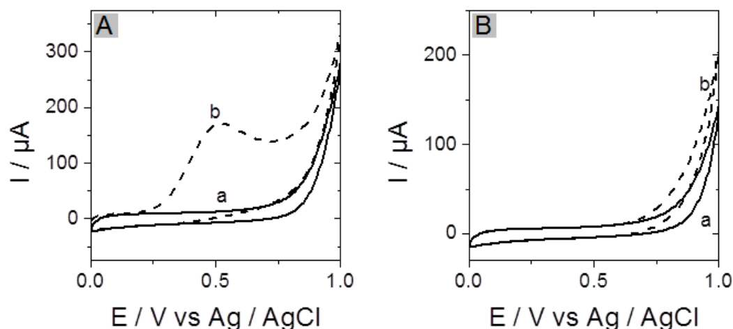
Figure 2.11. Cyclic voltammograms recorded using (A) an activated bare carbon felt or (B) a vinylphenyl functionalized carbon felt electrode in 0.1 M Tris-HCl buffer (pH 9.0) (a) in the absence and (b) in the presence of 1 mM NADH. All curves have been recorded at a potential scan rate of 20 \text{mV s}^{-1} . The surface area of the carbon felt electrode was 95 \text{cm}^2 .
