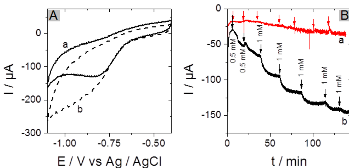
Figure 2.17. (A) Cyclic voltammograms recorded at a potential scan rate of 20 \text{ mV s}^{-1} using a Cys1-DSDH functionalized carbon felt electrode (a) in the absence and (b) in the presence of 1 mM D-
