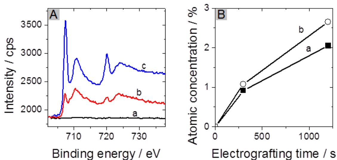
Figure 2.5. (A) XPS spectra of the narrow Fe2p region, as obtained for ferrocene functionalized electrodes via click chemistry for GC supports electrografted with 4-vinylaniline diazonium cations at -0.6 V for (a) 2 s, (b) 300 s, and (c) 1200 s. (B) Variation of (a) iron (■) and (b) sulfur (○) atomic concentrations measured from XPS data as a function of the electrografting time.
