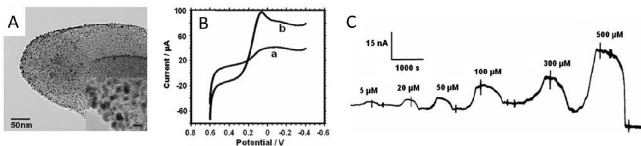
Fig. 5. (A) TEM micrograph of a Pt/PDDA-CMM nanocomposite loaded with 30% Pt (PDDA = poly(diallyldimethylammonium chloride); CMM = carbon mesoporous material). (B) Linear sweep voltammetric responses of the 30% Pt/PDDA-CMM electrodes to (a) 1 mM \text{H}_2\text{O}_2 in artificial cerebrospinal fluid (pH 7.4) and (b) 1 mM \text{H}_2\text{O}_2 solution (potential scan rate = 100 \text{ mV s}^{-1} ). (C) Amperometric response for different standard solutions of glucose obtained at 30% Pt/PDDA-CMM/GOx/Nafion modified electrode in the on-line microdialysis system (flow rate = 2.0 \text{ mL min}^{-1} ; applied potential = -200 \text{ mV} ). Reprinted from [172]. Cathodic current was defined by convention positively in this work.
