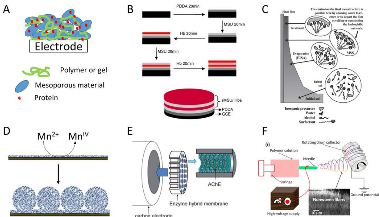
Fig. 6. Illustration of various approaches for preparing electrodes modified with mesoporous materials (used for biosensing purposes): (A) film of mesoporous particles deposited on an electrode surface by drop-casting suspension containing the mesoporous material and the protein (along with a polymeric binder); (B) layer-by-layer deposition of a mesoporous material [109]; (C) Mesostructured thin film prepared by evaporation induced self-assembly (EISA) [221]; (D) Anodic deposition of MnO 2 hierarchical spheres on ITO substrate [197]; (E) AChE-(F127-MST) enzyme hybrid membrane on nylon mesh [135]; (F) synthesis of aligned TiO 2 nanofibers by electrospinning [200].
