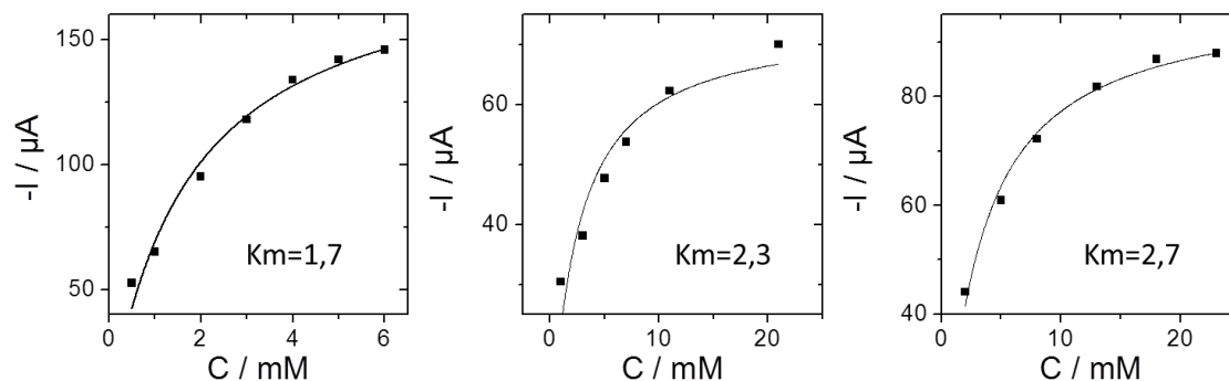
Figure 2.19. Amperometric responses to increasing concentration of D-fructose recorded using the same Cys1-DSDH functionalized CF electrode at an applied potential of -0.85\text{ V} , experiments were performed under nitrogen in 20\text{ mL } 0.1\text{ M} PBS buffer ( \text{pH } 6.5 ) containing 1.8\text{ mM} NADH and 0.1\text{ mM} [\text{Cp}^*\text{Rh}(\text{bpy})\text{Cl}]^+ . The surface area of the carbon felt electrode was 95\text{ cm}^2 .
