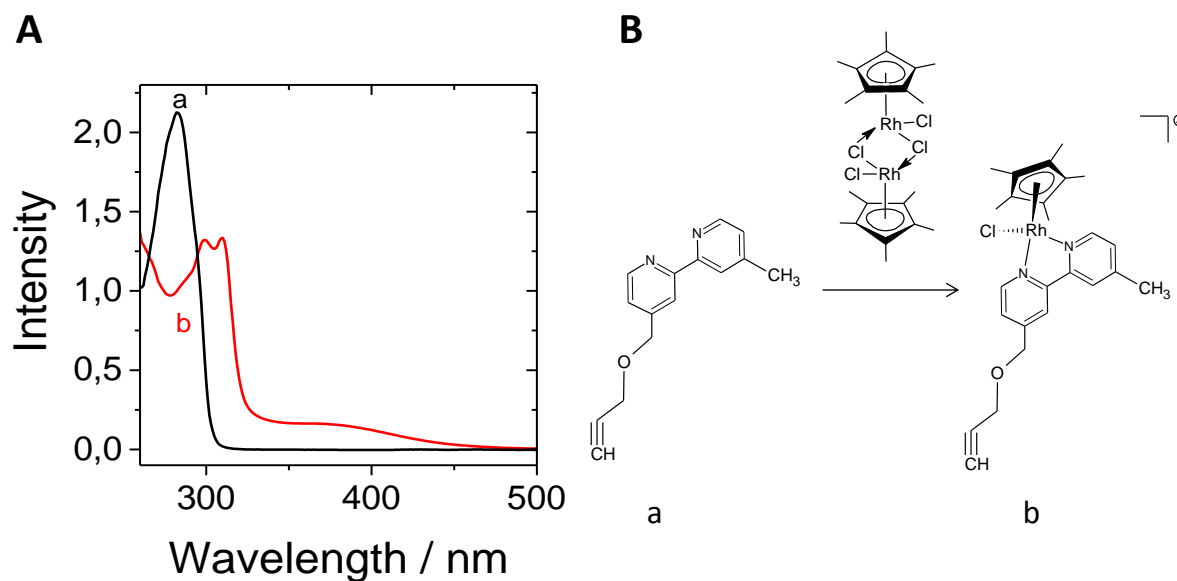
Figure 3.2. (A) UV-vis spectra recorded for 4-[(2-propyn-1-yloxy)methyl]-4'-methyl-2,2'-bipyridine in DMF/H 2 O (7/3) solution (a) before and (b) after complexation in the presence of a molar excess of (RhCp*Cl 2 ) 2 . (B) Corresponding illustration of the complexation process.
