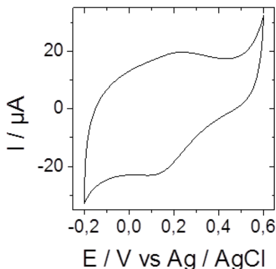
Figure 2.13. Cyclic voltammogram recorded in 0.1 M Tris-HCl buffer at pH 9.0 for ferrocene functionalized carbon felt electrode. Electrode potential scan rate was 20 \text{ mV s}^{-1} . The surface area of the carbon felt electrode was 95 \text{ cm}^2 .
