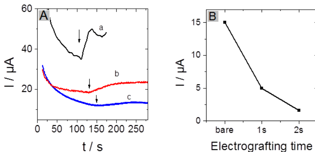
Figure 2.12. (A) Amperometric response to the addition of 0.1 mM NADH at an applied potential of 0.8 V in 0.1 M Tris-HCl buffer at pH 9.0 for activated carbon felt electro-grafted with 4-vinylaniline diazonium cations at -0.6 V for (a) 0 s; (b) 1 s and (c) 2 s. (B) Plot of the oxidation current to 0.1 mM NADH for these different electrodes. The surface area of the carbon felt electrode was 95 \text{cm}^2 .
