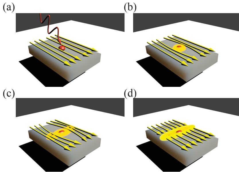
Figure III.1: (a) A single photon is absorbed by the nanowire. (b) Creation of a hotspot making the material locally resistive. (c) The density of current increases as the current tries to bypass the resistance. (d) Complete phase transition. The material becomes locally resistive and a voltage pulse is detected.
