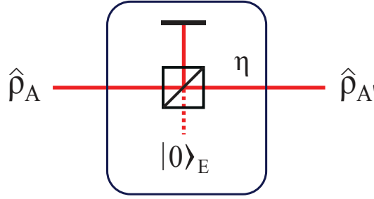
Figure I.2: Losses modeled by a damping channel
