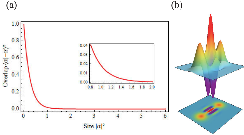
Figure V.8: (a) Overlap of two coherent states |\alpha\rangle and |- \alpha\rangle for several mean photon number |\alpha|^2 . The inset gives a zoom on the 1 to 2 range. (b) Wigner representation of an even cat state of size |\alpha|^2 = 3 .
