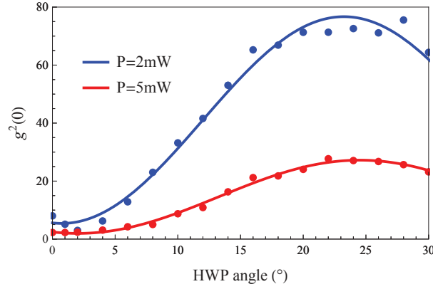
Figure V.3: Evolution of the g^{(2)}(0) as a function of the angle of the wave plate, for two different input pump powers, 2 mW and 5mW, corresponding respectively to 0.7 and 1.6 dB of squeezing.
