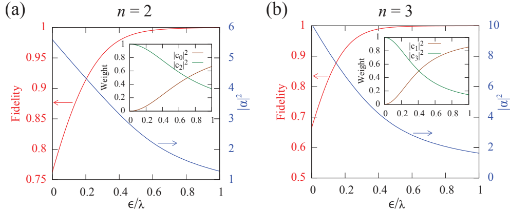
Figure V.13: (a) Two-photon detection: fidelity with a squeezed even cat state as a function of the ratio \epsilon/\lambda . The fidelity is optimized by the size |\alpha|^2 and the squeezing of the target state. The inset gives the weights of the vacuum and two-photon components. (b) Three-photon detection state and fidelity with a squeezed odd cat state.
