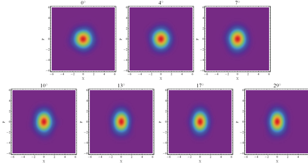
Figure V.4: Wigner functions for several HWP angles showing the transition from a thermal state corresponding to the angle 0^\circ to a squeezed vacuum state.
