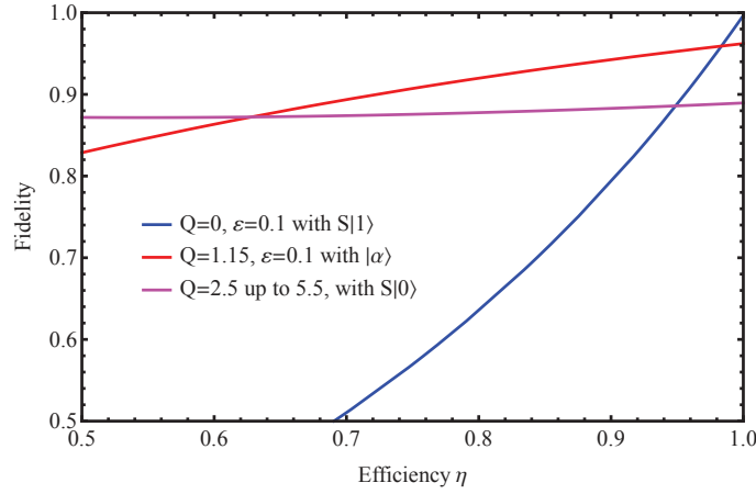
Figure VI.17: Theoretical plot of the fidelity depending on the efficiency of the system \eta = \eta_{Alice} = \eta_{Bob} for different remotely prepared states on Bob's side.
