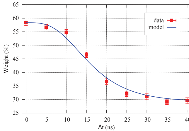
Figure IV.9: Weight of two-photon component for the optimal temporal mode f_s(t) as a function of the delay between the two triggers. The blue line corresponds to the model taking into account the overall loss and the OPO bandwidth.
