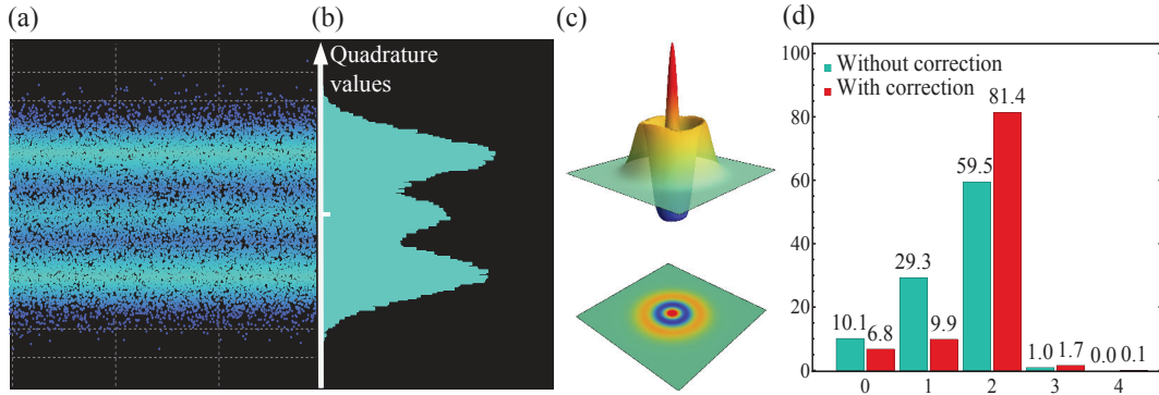
Figure IV.5: (a) Quadrature values and (b) distribution measured via the homodyne detection for the heralded state. (c) Wigner function of the generated two-photon Fock state with correction from detection losses (15%). (d) Photon number probabilities of the generated two-photon Fock state, with and without correction from detection losses (15%).
