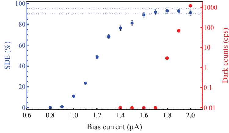
Figure III.7: System detection efficiency (SDE) at 1064 nm (blue) and dark counts (red) as a function of the bias current. For a bias current of 1.8\mu A , a value equal to 0.9 times the switching current, a SDE of 93 \pm 3\% is obtained with a dark noise of 3 cps. These measurements are obtained at an operating temperature of 1.8 K.
