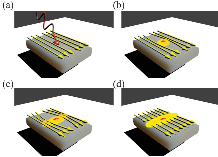
Figure III.1: (a) A single photon is absorbed by the nanowire. (b) Creation of a hotspot making the material locally resistant. (c) The density of current increases as the current tries to bypass the resistance. (d) Complete phase transition. The material becomes locally resistant and a voltage pulse is detected.
