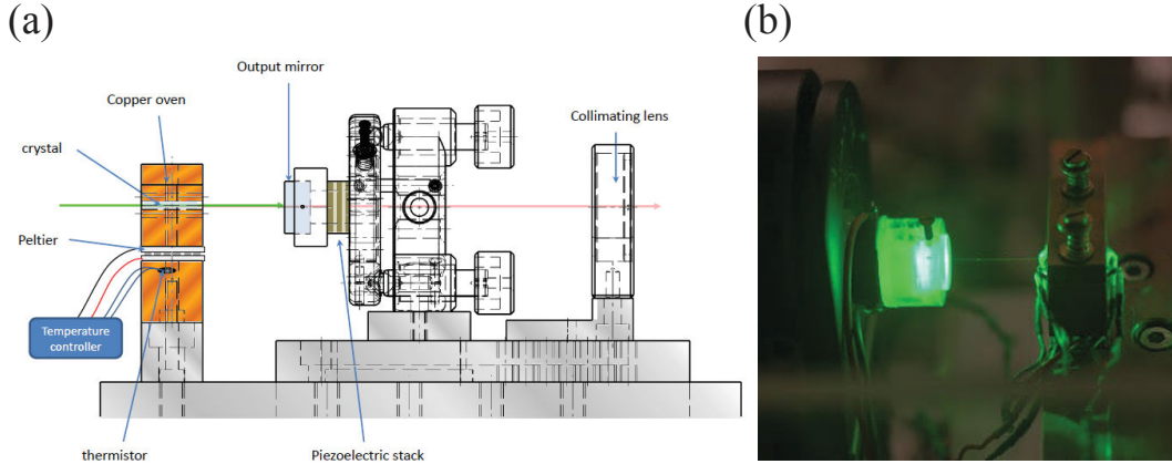
Figure II.3: (a) Scheme of the mount of the type-I OPO. (b) Picture of the similar type-II OPO mount.
