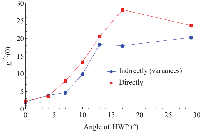
Figure V.7: Evolution of the g^{(2)}(0) of the one output of the PBS as a function of the angle of the wave plate. The indirect method of evaluating the g^{(2)}(0) using homodyne detection and Wigner function reconstruction is given in blue, while the direct method, using two single-photon detectors and coincidence counts is given in red.
