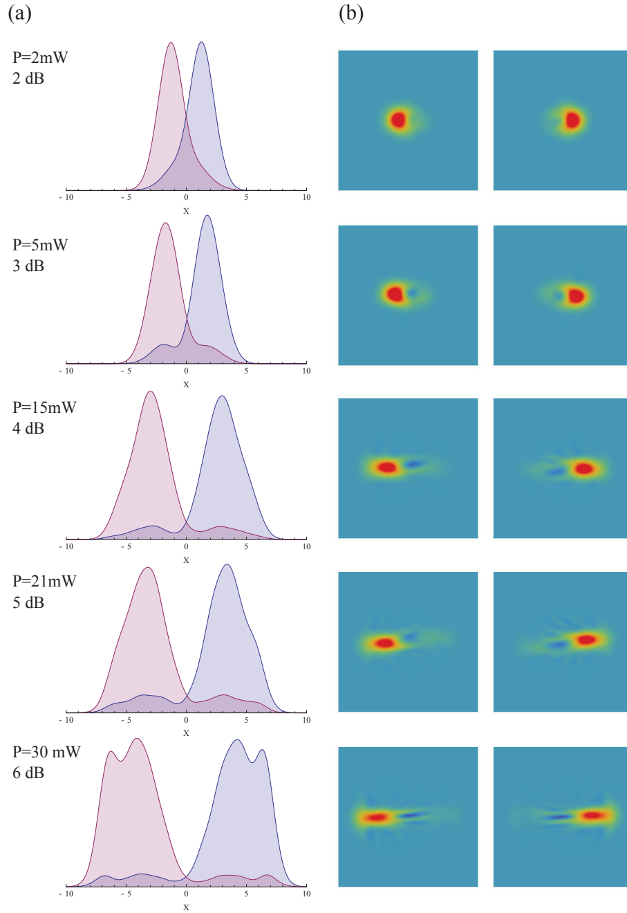
Figure VII.7: Experimental results for the 2-click state. (a) Marginal distributions and (b) Wigner functions of the two reduced density matrices \rho_{\Psi_{\pm}} = \langle \pm |_A \hat{\rho}_{AB} | \pm \rangle_A , for different input pump powers for the type I-OPO, i.e. for different amounts of squeezing on Bob's mode. These results are corrected from detection losses (15%). |\Psi_{-}\rangle marginal distribution is plotted in purple and the corresponding Wigner function is on the left side.
