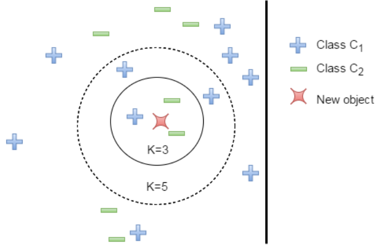
Figure 5.5: k -NN algorithm example
