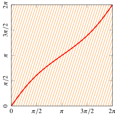
FIGURE 2.8 – Density of \mathbf{O} \cap \mathbf{H} in \mathbf{H}
