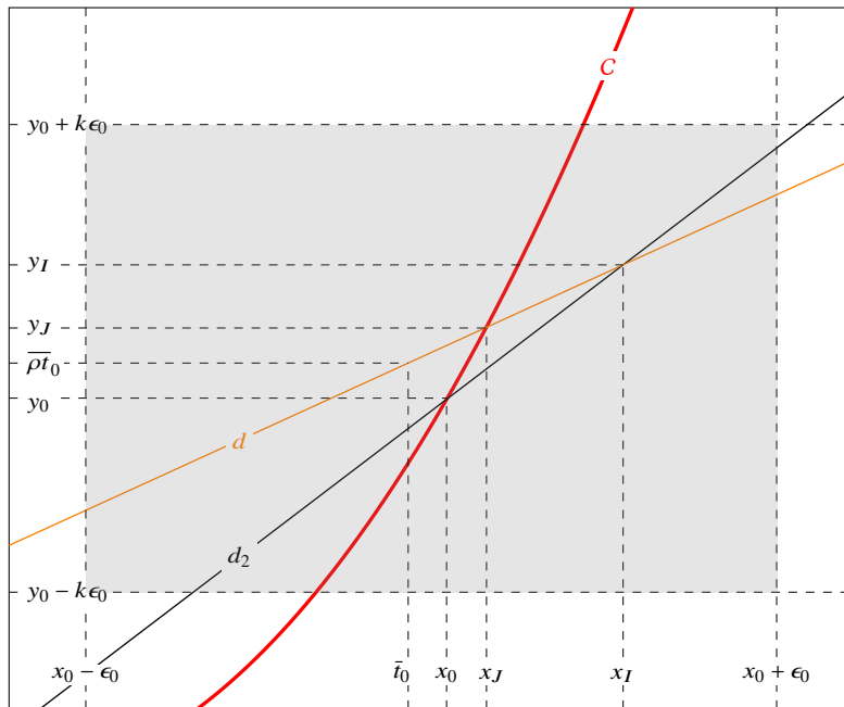
FIGURE 2.9 – Zoom in the box ]x_0 - \varepsilon_0; x_0 + \varepsilon_0[ \times ]y_0 - k\varepsilon_0; y_0 + k\varepsilon_0[ when \dot{\psi}(x_0) > \rho
