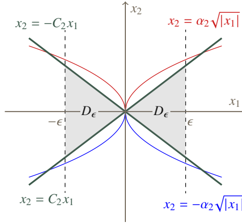
FIGURE 3.5 – Neighborhood D_\epsilon
