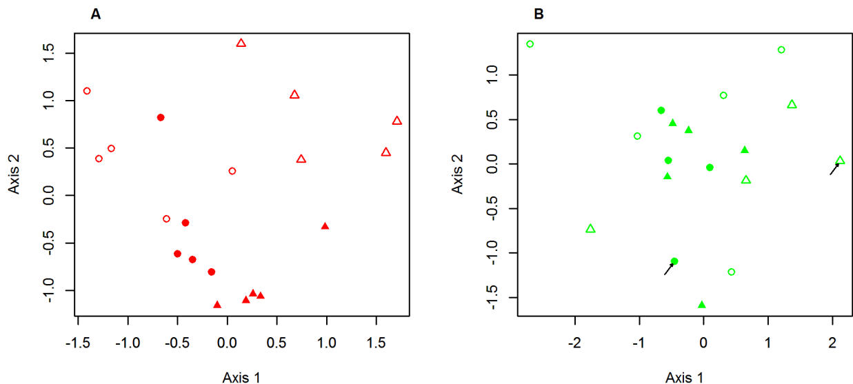
Figure 5. Variation in the composition of the scents emitted by figs (A) and leaves (B). Two-dimensional NMS ordinations on relative scent composition (% each VOC) computed separately on (A) fig scents (stress-value = 14%) and (B) leaf scents (stress-value = 11%). Circles represent Ficus nota and triangles Ficus septica samples, open symbols are sunrise samples and closed symbols are noon samples. Black arrows indicate places where two samples of the same category share the same locus.
