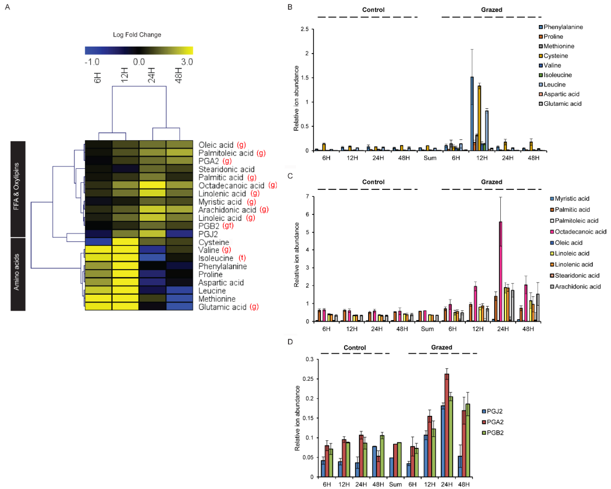
Fig 2. Metabolic profiling in grazed L. spicata highlighted distinctive accumulation dynamics of Amino Acids and Free Fatty Acids. (A) Heat map of the amino acids, free fatty acids and oxylipins detected in L. spicata in laboratory controlled conditions. Values represent the log fold-change of control conditions (n = 3). Time points and compounds were clustered according the Pearson Correlation. The letter (g) indicates a significant difference according to grazed condition, and (t) indicate significant differences for time ( P < 0.05 , Kruskal-Wallis test). (B-D) Time course of relative abundances of free amino acid (B), free fatty acids (C) and oxylipin contents (D) in control and grazed L. spicata (mean of three replicates \pm SE).
