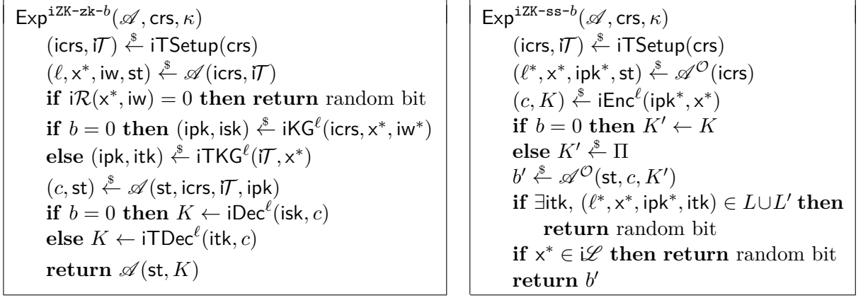
Figure 4.2: Experiments \text{Exp}^{\text{iZK-zk-b}} for zero-knowledge of iZK, and \text{Exp}^{\text{iZK-ss-b}} for simulation-soundness of SSiZK
