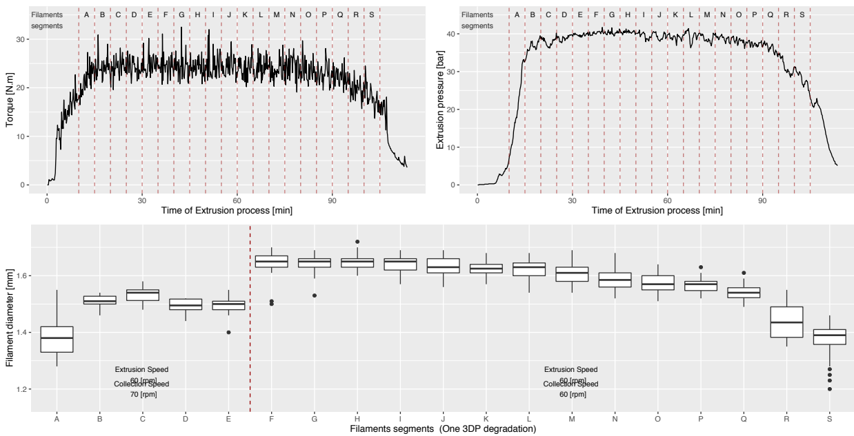
Characteristical curves for filament of 'One 3DP'
