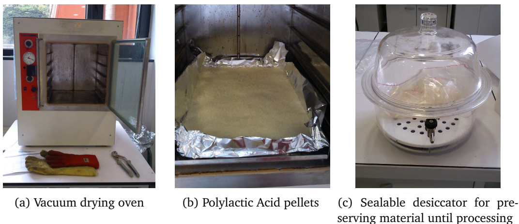
Figure 4.9: Material preparation before extrusion
