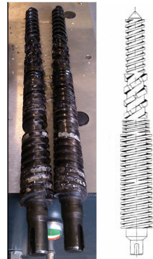
(b) Intensive mixing screw of the extruder machine
