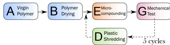
Figure 5.1: Experimental strategy for Reference process chain used for PLA degradation.
