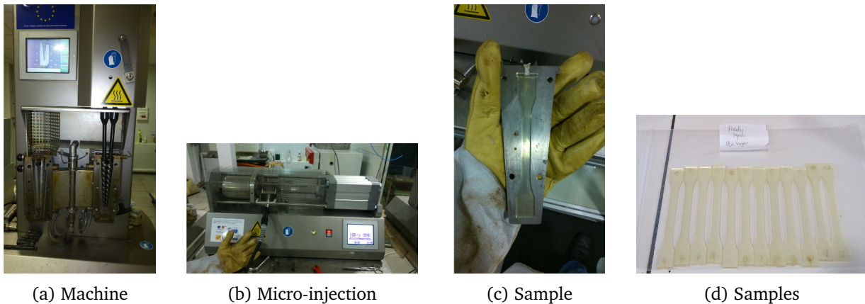
Figure 4.16: Micro-compounding machine used for fabrication of the mechanical samples
