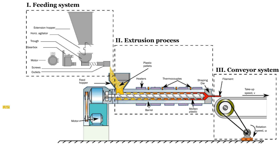
Figure 4.11: Schematical extrusion process for fabrication of feedstock 3D printing material
