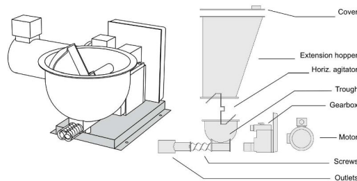
Figure 4.12: Schematical view of the feeding system
