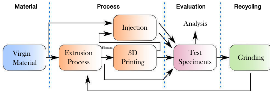
Figure 4.10: Mechanical recycling steps for the case of fabrication of recycled filament.
