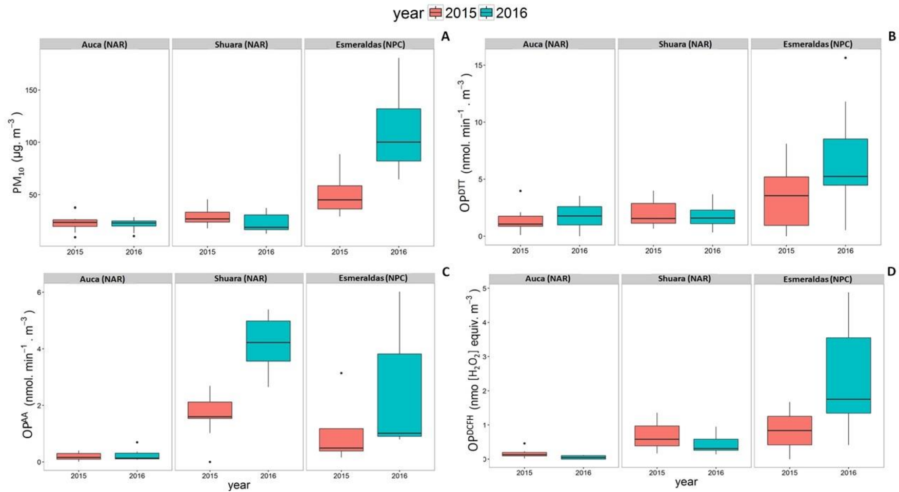
Fig. 3. A. PM_{10} mass concentration ( \mu\text{g} \cdot \text{m}^{-3} ) and Oxidative Potential ( OP \cdot \text{m}^{-3} ) measured by B. Dithiothreitol (DTT), C. Ascorbic acid (AA) and D. Dichlorofluoresceine (DCFH) assays in Auca, Shuara and Esmeraldas, for the 2015 and 2016 years.
