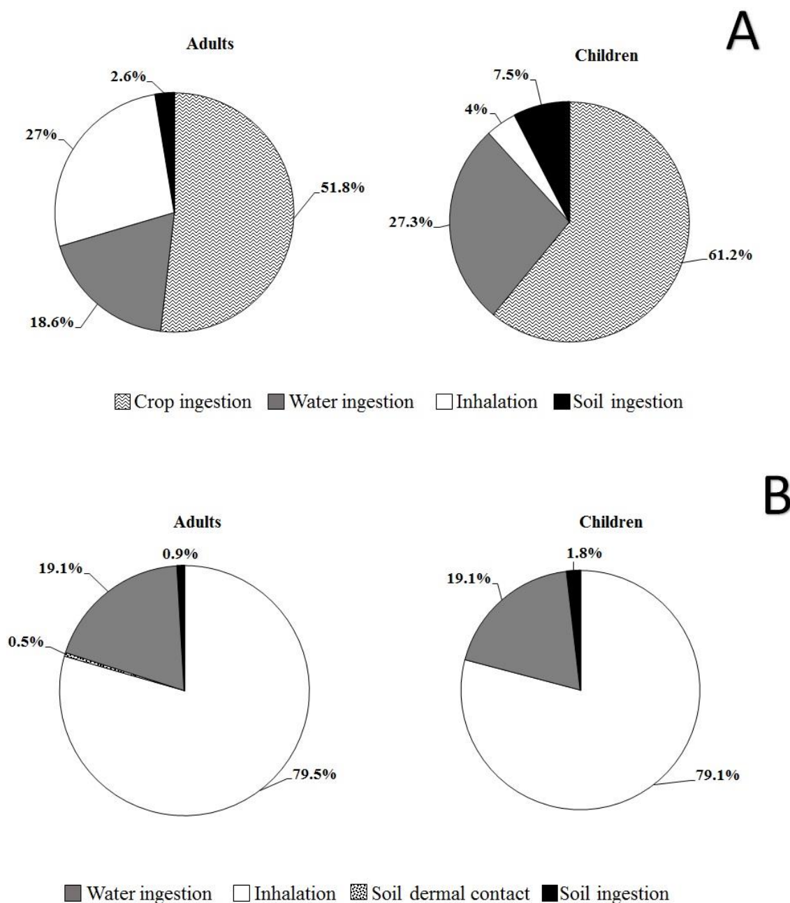
Fig. 3. Hazard Index (HI) for non-carcinogenic health effects of metal(loid)s ( A ) and Total Cancer Risk (TCR) ( B ) considering all exposure routes for adults and children living in the Northern Amazon Region of Ecuador.
