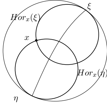
FIGURE 2.1 – Cocycle de Busemann
