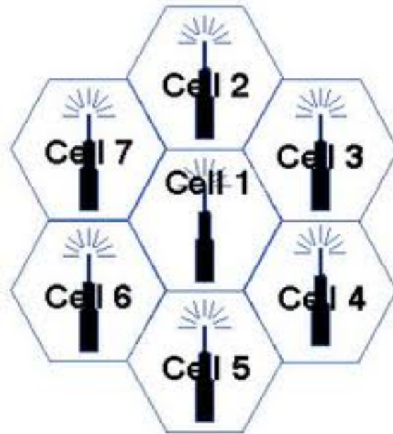
Figure 1.3 – Divide the coverage area using Voronoi.
