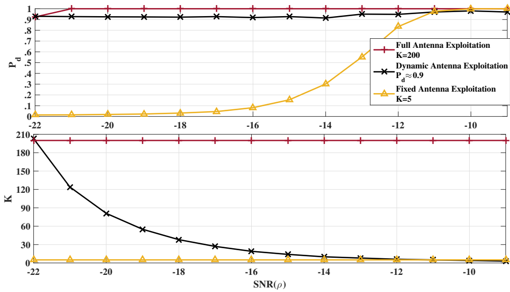
Figure 5.7: Empirical P_d of the SCN detector and the corresponding number of antennas, K , used for sensing in Full, Dynamic and Fixed methods w.r.t \rho and fixing N = 500 .
