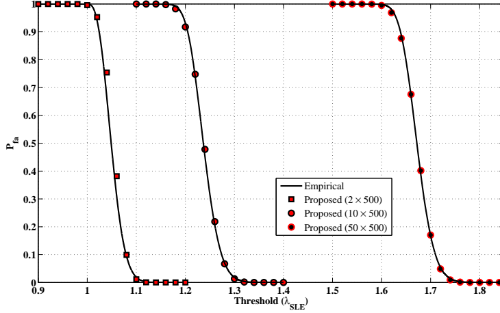
Figure 4.4: Empirical P_{fa} for the SLE detector and its corresponding proposed form in (4.22) for different values of K with N = 500 samples.
