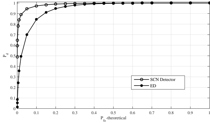
Figure 3.16: ROC of the SCN Detector vs. ROC of the ED for K = 3 , N = 500 , SNR = -10dB and 0.1dB noise uncertainty.
