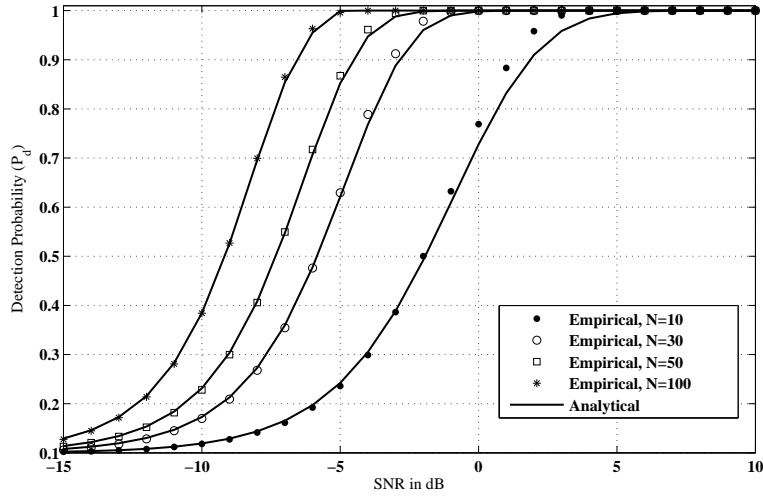
Figure 3.4: Empirical P_d of the SCN metric and its corresponding analytical P_d using normalized non-central/central approximation as a function of SNR for K = 3 and \hat{P}_{fa} = 0.1 .
