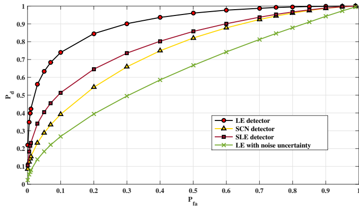
Figure 5.10: ROC of the LE, SCN and SLE detectors when k = 5 , N = 500 and \rho = -15dB .
