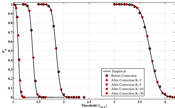
Figure 4.5: Empirical P_d for the SLE detector and its corresponding proposed form for different values of K with N = 500 samples and \rho = -10dB before and after mean error correction.
