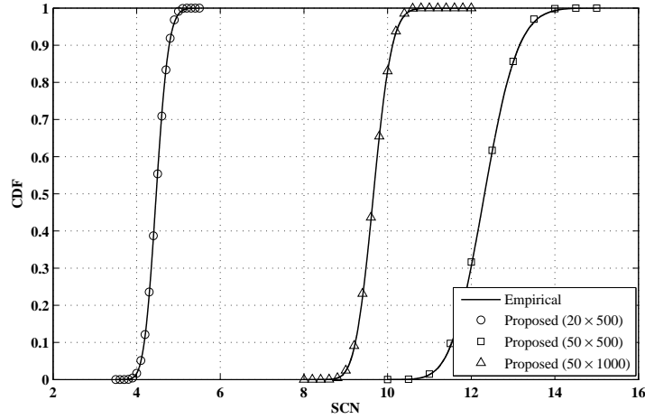
Figure 3.12: Empirical CDF of the SCN and its corresponding proposed GEV approximation for different values of K and N under \mathcal{H}_1 hypothesis with \rho = -10dB .
