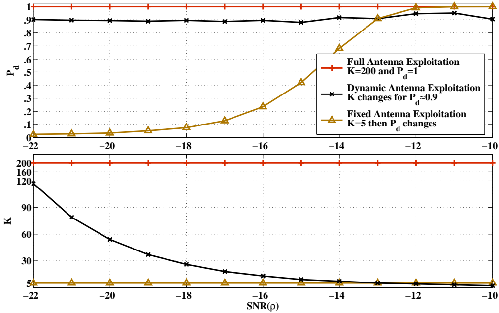
Figure 5.5: Empirical P_d of the LE detector and the corresponding number of antennas, K , used for sensing in Full, Dynamic and Fixed methods w.r.t \rho and fixing N = 500 .
