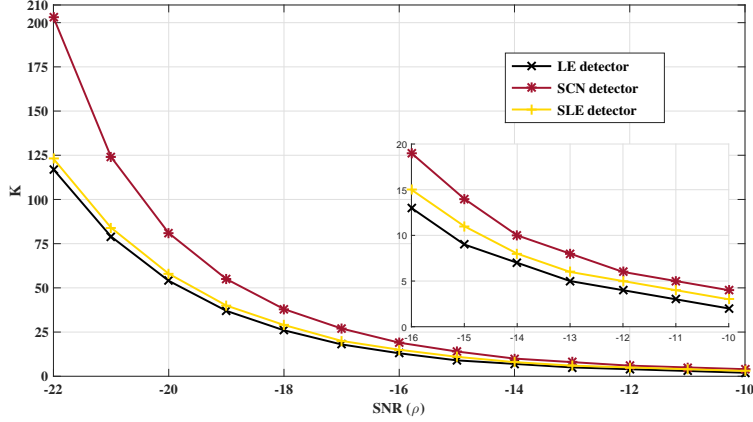
Figure 5.11: Required K of the LE, SCN and SLE detectors for dynamic antenna exploitation w.r.t \rho and fixing N = 500 , P_d = 0.9 and P_{fa} = 0.01 .
