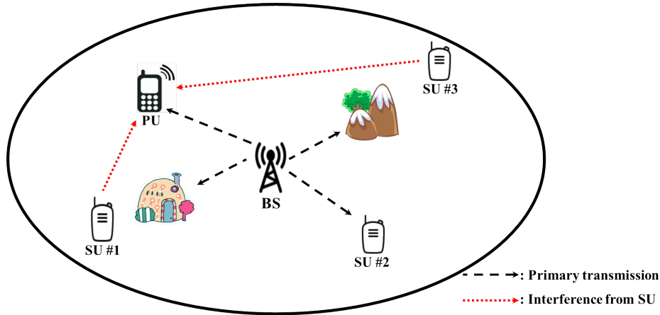
Figure 2.7: Shadowing Effect and Hidden Node problem.
