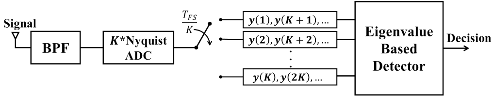
Figure 2.8: Eigenvalue based detector using fractional sampling.
