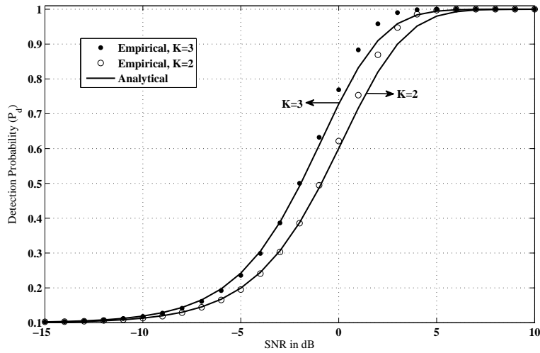
Figure 3.5: Empirical P_d of the SCN metric and its corresponding analytical P_d using normalized non-central/central approximation as a function of SNR for N = 10 and \hat{P}_{fa} = 0.1 .
