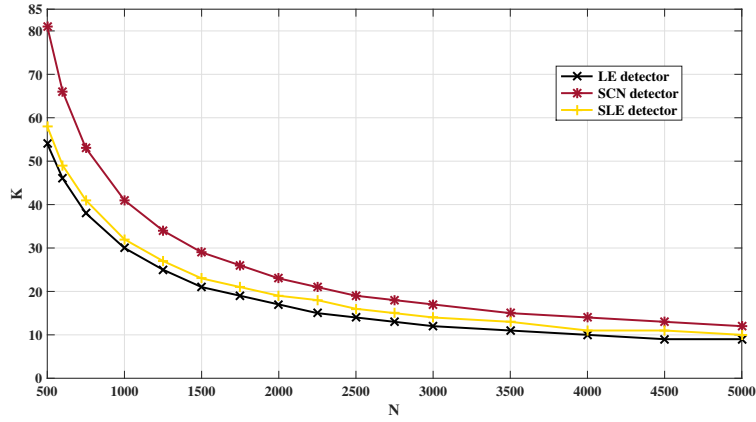
Figure 5.12: Required K of the LE, SCN and SLE detectors for dynamic antenna exploitation w.r.t N and fixing \rho = -20dB , P_d = 0.9 and P_{fa} = 0.01 .
