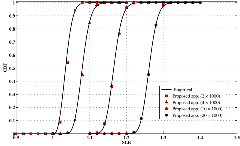
Figure 4.2: Empirical CDF of the SLE under \mathcal{H}_0 hypothesis and its corresponding Gaussian approximation for different values of K with N = 1000 .
