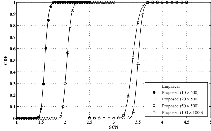
Figure 3.11: Empirical CDF of the SCN and its corresponding proposed GEV approximation for different values of K and N under \mathcal{H}_0 hypothesis.
