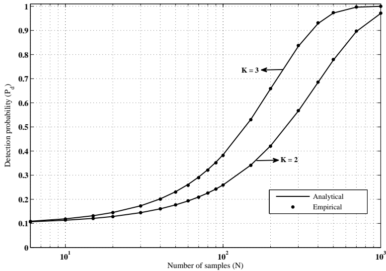
Figure 3.6: Empirical P_d of the SCN metric and its corresponding analytical P_d using normalized non-central/central approximation as a function of the number of received samples for \rho = -10dB , and \hat{P}_{fa} = 0.1 .
