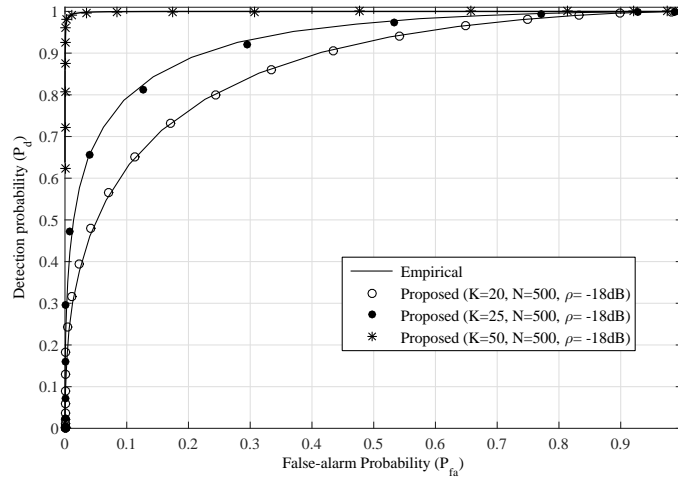
Figure 3.13: Empirical ROC of the SCN detector and its corresponding proposed approximation for different values of K with N = 500 and \rho = -18dB .
