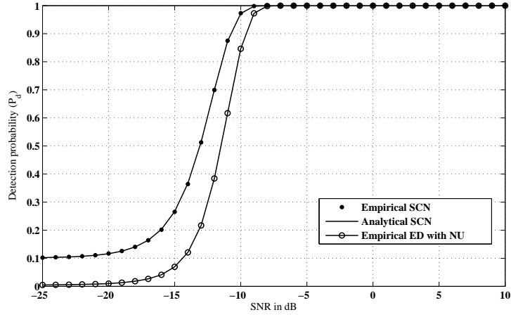
Figure 3.15: P_d of the SCN detector and the ED with 0.1dB noise uncertainty as a function of SNR for K = 3 , N = 500 , and P_{fa} = 0.1 .
