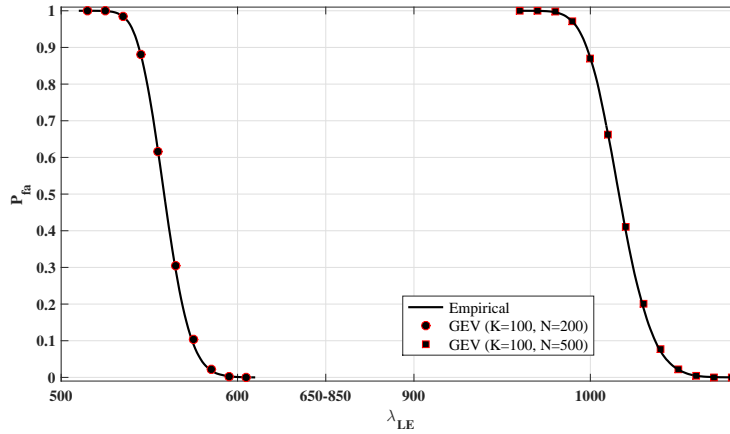
Figure 5.3: Empirical P_{fa} of the LE detector in the asymptotic case and its corresponding GEV approximation for K = 100 and different values of N .
