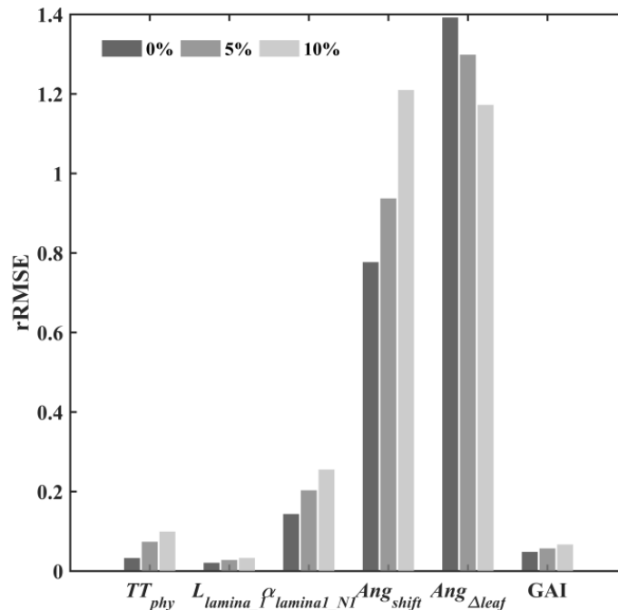
Fig. 5 Accuracy of 5 the estimation of the 5 parameters and GAI during P_{bf\_tiller} stage using the GF contaminated with different levels of noise and using the 5 directions concurrently.
