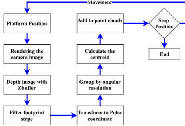
Fig. 7 Schematic diagram of the LiDAR simulator
