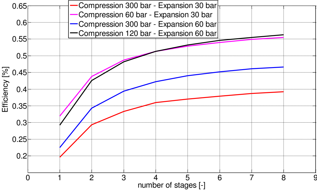
Figure 104 – System primary efficiency
