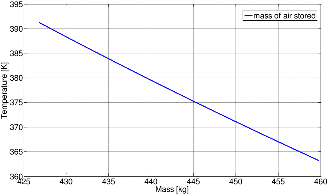
Figure 90 – The mass of air required to be stored function of air engine inlet temperature
