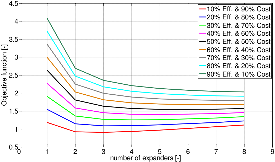
Figure 117 – Objective function determination to obtain 30 kWh energy with air stored a 300 bar and expanded from 60 bar function of number of stages
