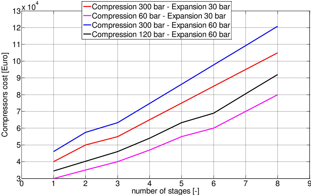
Figure 111 – Compressors cost
