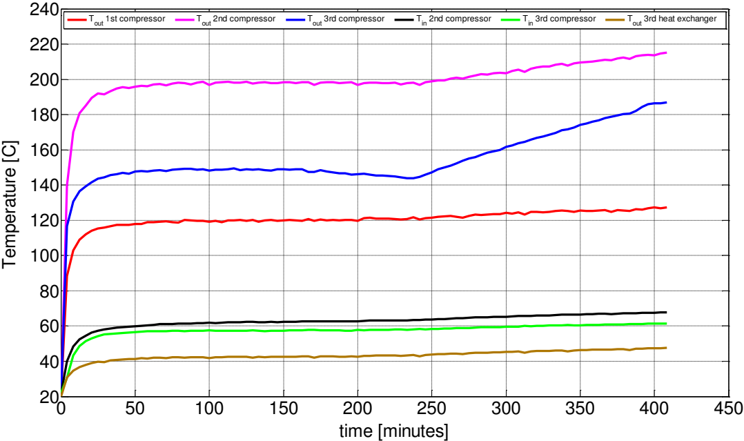
Figure 67 – Experimental measurements of temperature before and after each stage of compression
