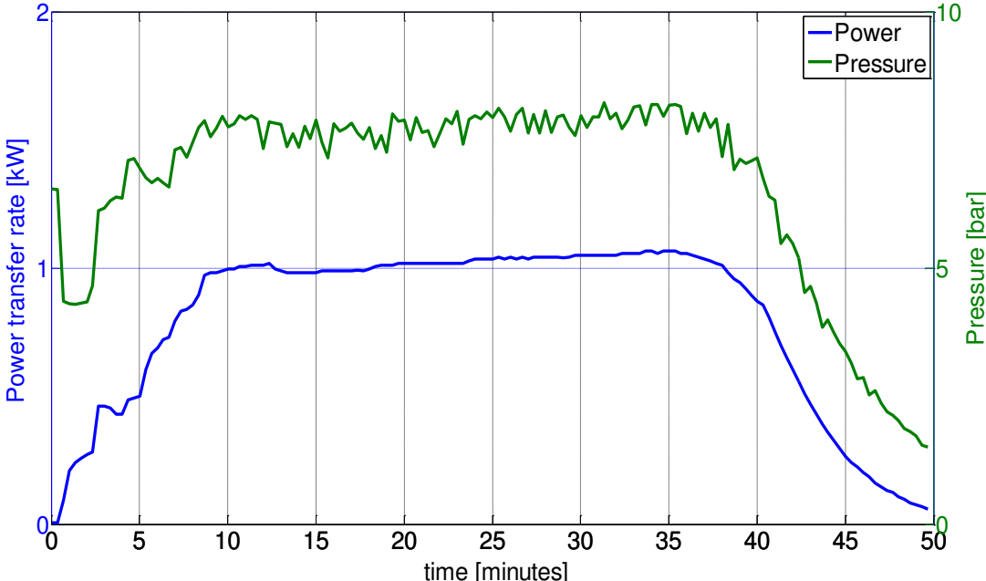
Figure 79 – Power and pressure evolution in time during discharging process
