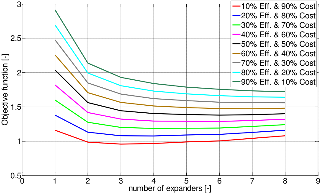
Figure 118 – Objective function determination to obtain 30 kWh energy with air stored a 60 bar and expanded from 30 bar function of number of stages
