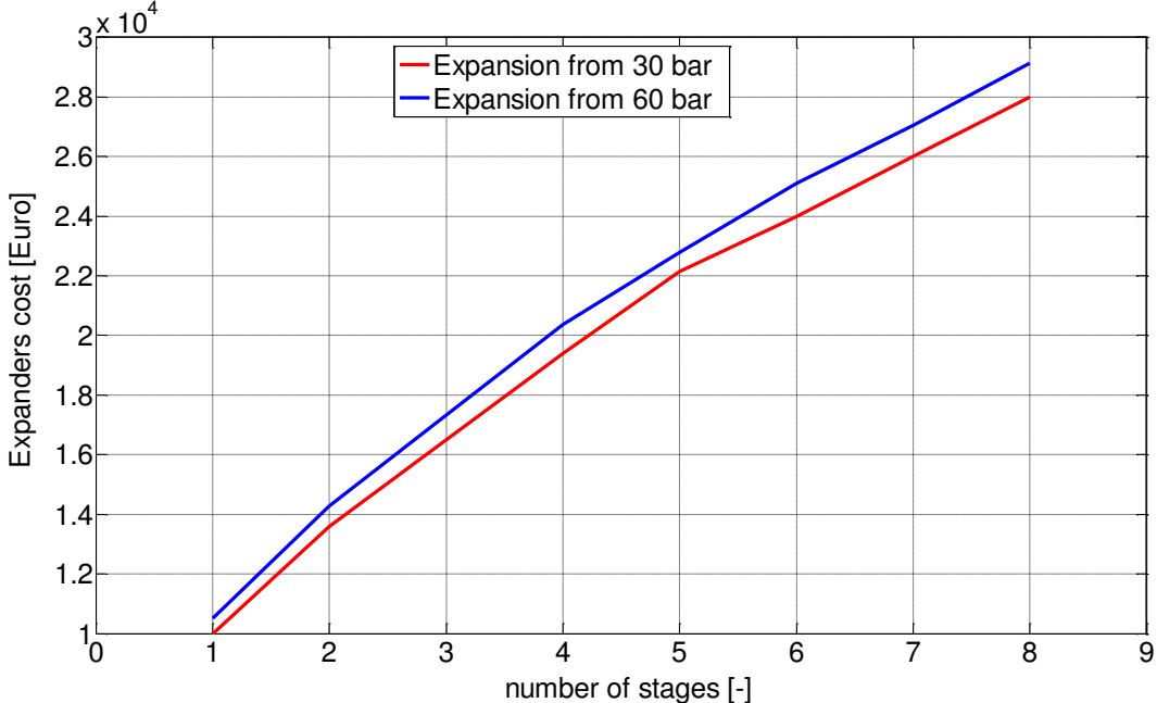
Figure 114 – Expanders cost
