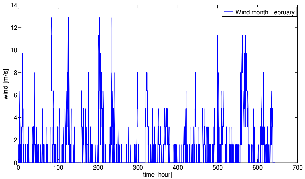
Figure 12 – Wind speed illustration during the month of February 2015
