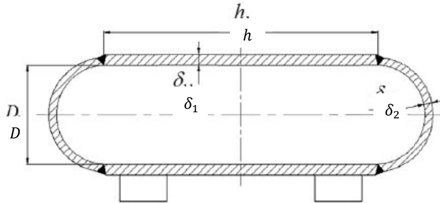
Figure 21 – Storage tank pre-dimensioning [42]
