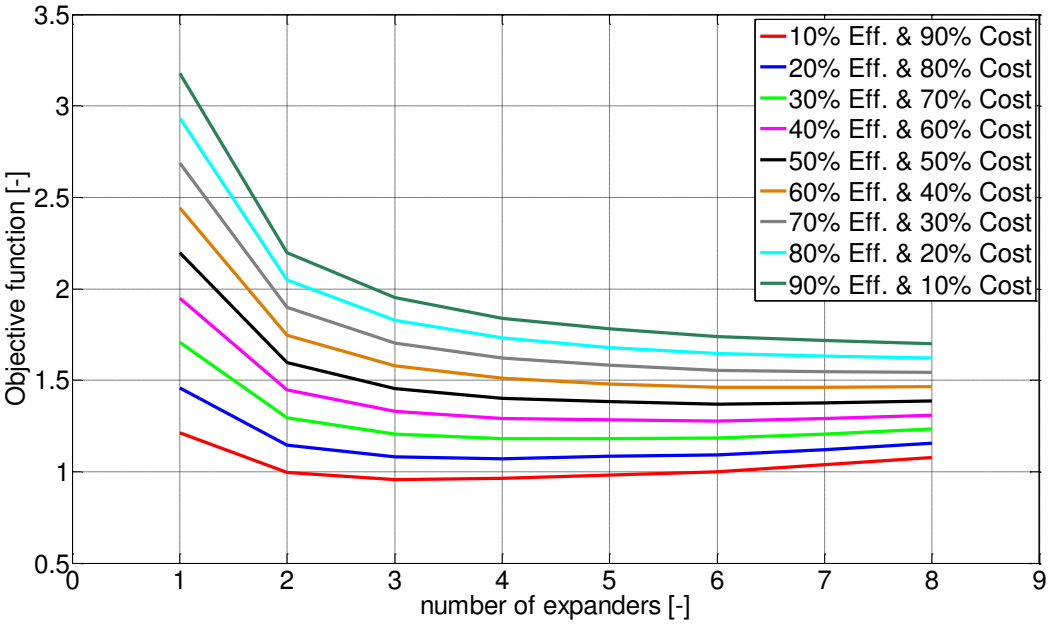
Figure 119 – Objective function determination to obtain 30 kWh energy with air stored a 120 bar and expanded from 60 bar function of number of stages
