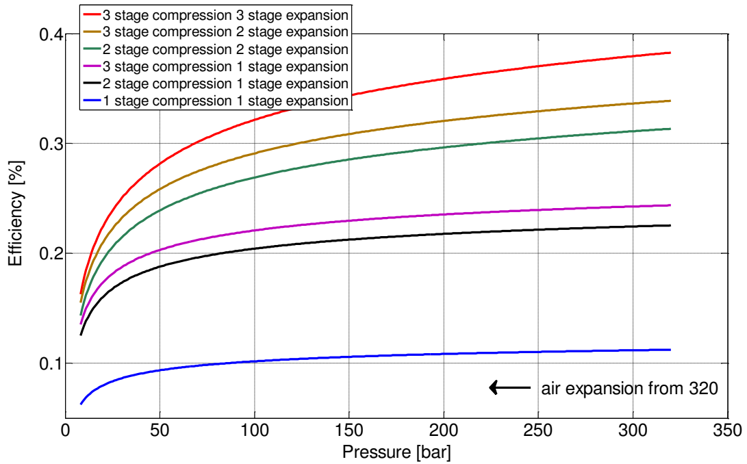
Figure 47 – Graphical representation of efficiency function of input expander pressure - adiabatic process
