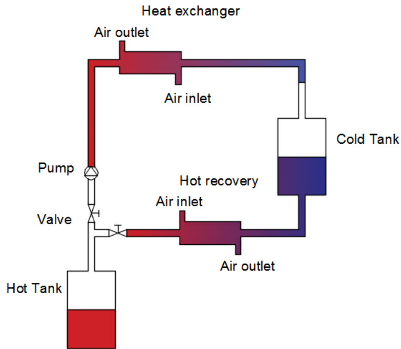
Figure 49 – Thermal energy storage system
