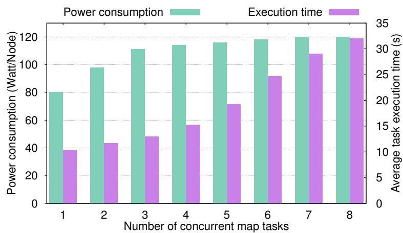
(a) Map tasks in the WordCount application.
