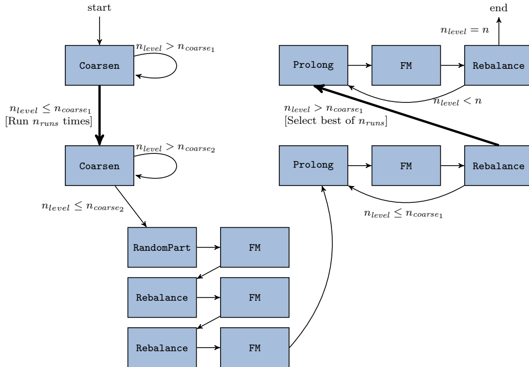
Figure A.1.1 – The default multilevel algorithm used by MeTiS
