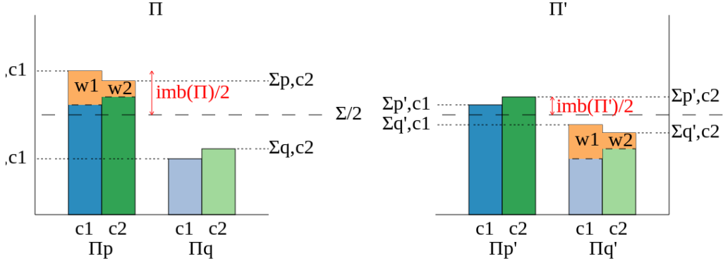
Figure 7.4.1 – Example of how the imbalance changes when a vertex (in orange) moves (left: before move, right: after move)
