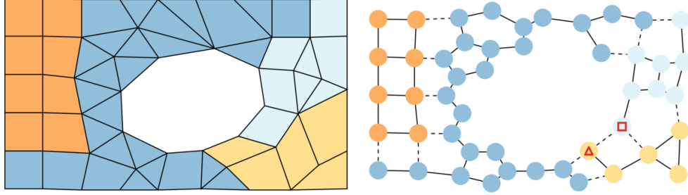
Figure 2.4.2 – 4-partition of a mesh and of its corresponding graph
