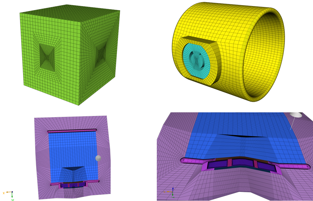
Figure 9.1.1 – The mesh LMJ , which is our industrial test case. Top left: the whole domain, which is in a cube. Top right: the capsule that is inside the cube. Bottom left: upper view of the interior of the capsule. The interior is colored in blue, cells containing gold are in pink, cells containing foam are in purple. Bottom right: side view of the capsule. Red cells are the slits in the foam.
