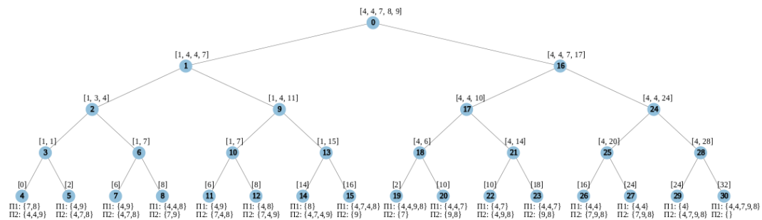
Figure 3.2.3 – The complete Karmarkar-Karp bipartitioning algorithm tree applied to S_e : the two largest numbers of a node are replaced in the left branch by their difference, and in the right branch by their sum. The nodes are numbered according to their visited order. The leaves are the partitions, with their absolute differences indicated above. They are computed a posteriori, using the method explained in Section 3.2.2. In this example, the optimal (and perfect) partition is the first computed one (obtained at node 4).
