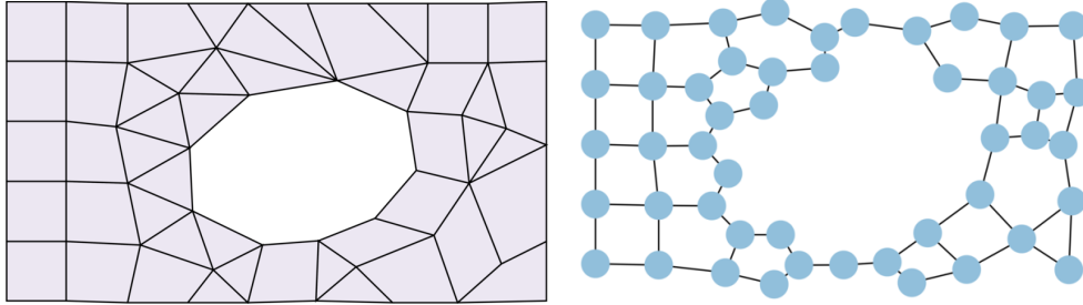
Figure 2.4.1 – Example of a mesh and its corresponding dual graph
