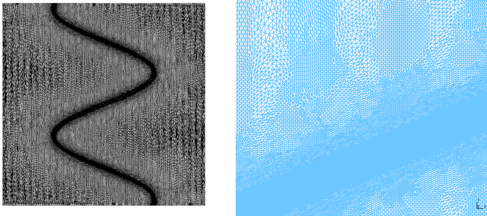
Figure 9.1.4 – The biggest mesh, Shock , of 1 196 352 cells. On the left: the whole mesh. On the right: a zoom on the center of the picture.
