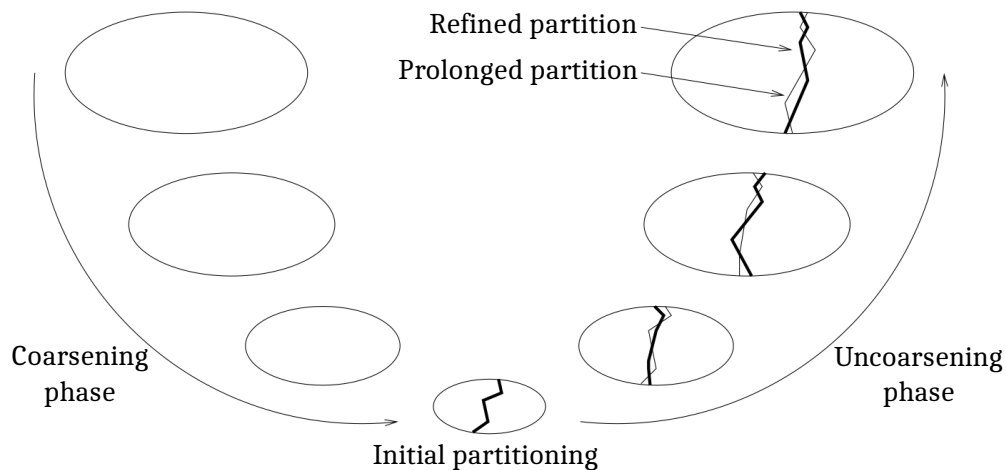
Figure 4.5.1 – The Three Phases of the Multilevel Algorithm (image from the Scotch-6.0.4manual of Pellegrini [2008])
