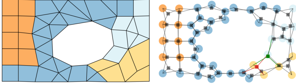
Figure 2.3.2 – Example of a 4-partition of a mesh and of its corresponding hypergraph
