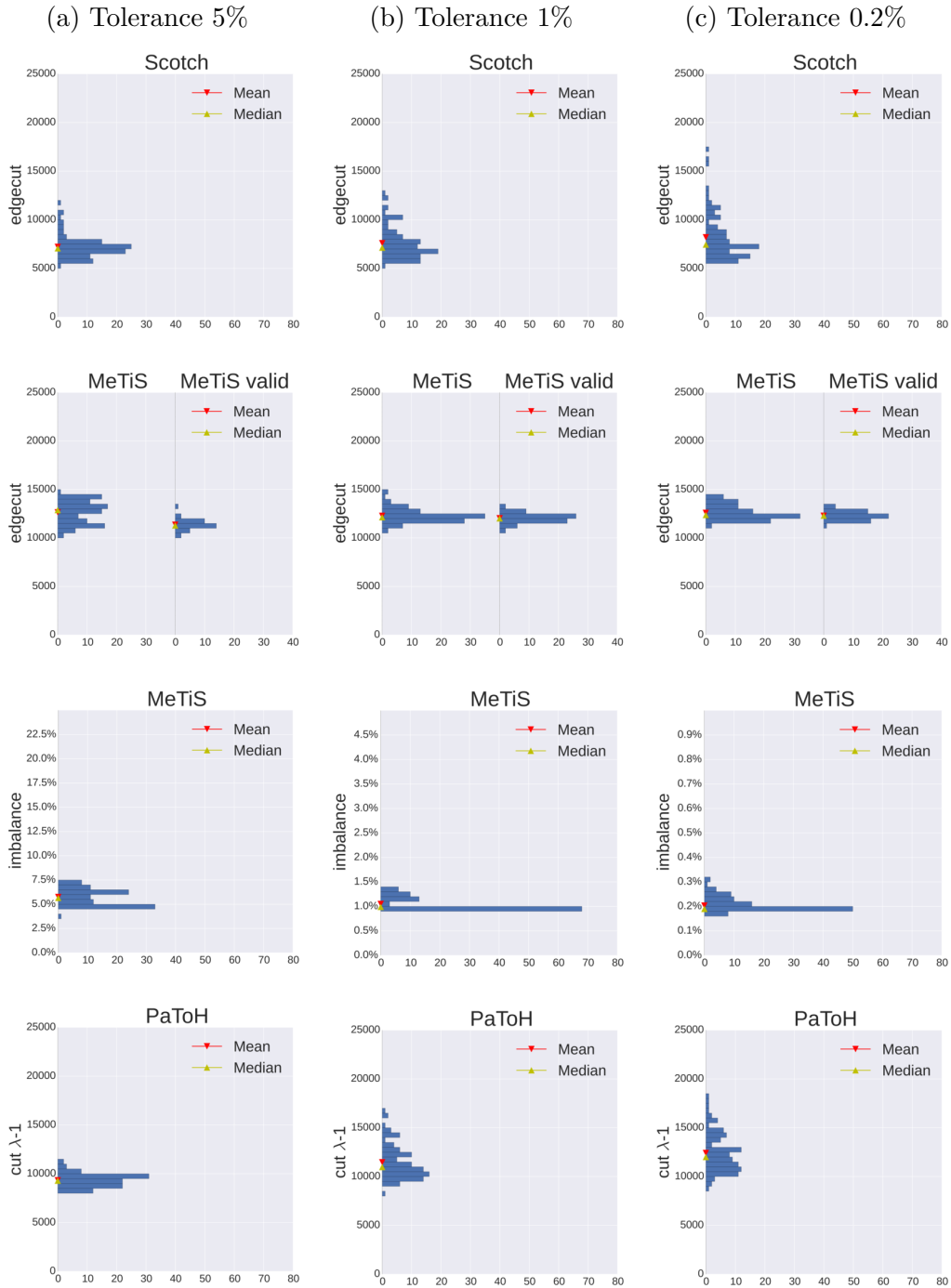
Figure 9.2.1 – Bar plots of the edgecut , cut_{\lambda-1} and imbalance of the partitions returned by Scotch, MeTiS and PaToH over 100 runs on the mesh Mushroom
