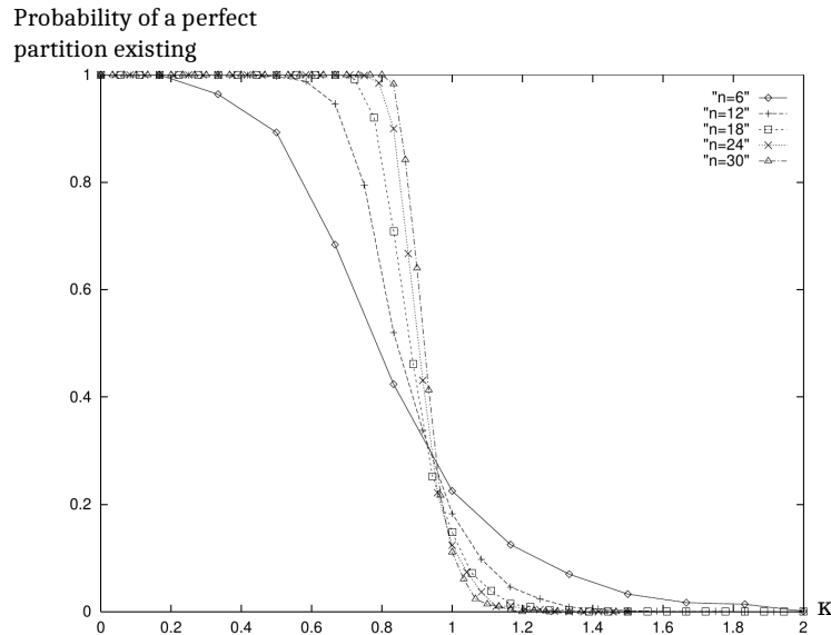
Figure 3.1.1 – Image from Gent and Walsh [1998] showing that the probability that a perfect partition exists drops for \kappa \approx 1 . This phenomenon is called a phase transition, and characterizes the hard instances of the number partitioning problem (the ones for which \kappa \approx 1 ).
