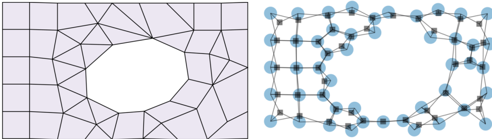
Figure 2.3.1 – A mesh and its corresponding hypergraph
