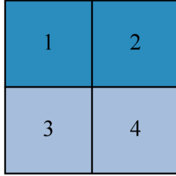
Figure 2.6.1 – A bipartition of a 4-cell mesh, which can be encoded with the vector [1, 1, 2, 2]
