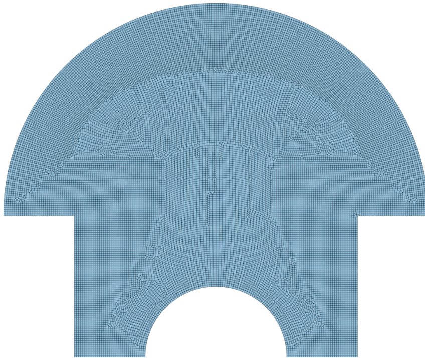
Figure 9.1.2 – The smallest mesh, Mushroom , of 22 800 cells
