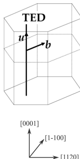
FIGURE 1.30 – Dislocation de type "coin" du SiC-4H[91].
