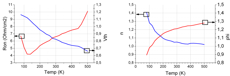
(a) Diode A, JBS Tungstene.
