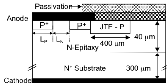
FIGURE 2.12 – Structure de la diode JBS retenue.
