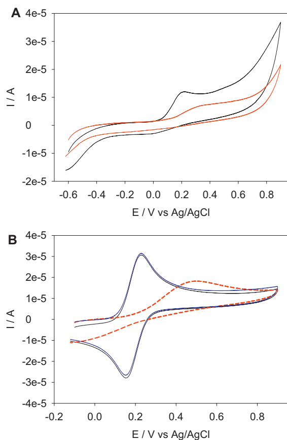
Fig. 3. (A) CV ( 100 \text{ mV s}^{-1} ) on a single carbon electrode put in contact with a one week aged dopamine solution ( 2 \text{ mg mL}^{-1} in 50 \text{ mM} Tris buffer at \text{pH}=8.5 ), after the first (.....) and the fourth scan (—). (B) CV ( 100 \text{ mV s}^{-1} ) of a pristine carbon electrode put in contact with a \text{NaCl-K}_4\text{Fe(CN)}_6 electrolyte (.....), the same electrode after 4 potential scans (—) in the presence of a one week aged dopamine solution, and of the same electrode after two polishing steps with 1 and 0.1 \mu\text{m} alumina powders (—).
