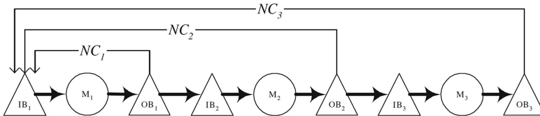
Figure II-XXVIII: Generic Kanban system (González-R et al., 2011)
