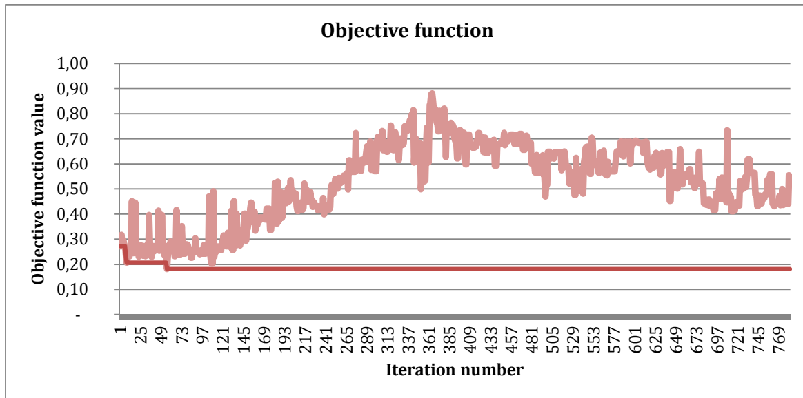
Figure IV-XIII: OTD and WC weighting objective function
