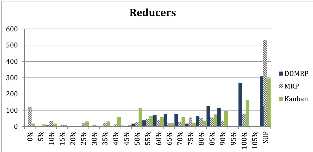
Figure III-XV: Reducer inventory distribution for high demand variability and visibility scenario
