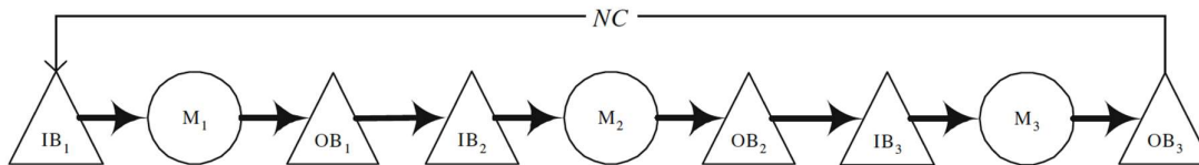
Figure II-XXIX: ConWIP system (González-R et al., 2011)
