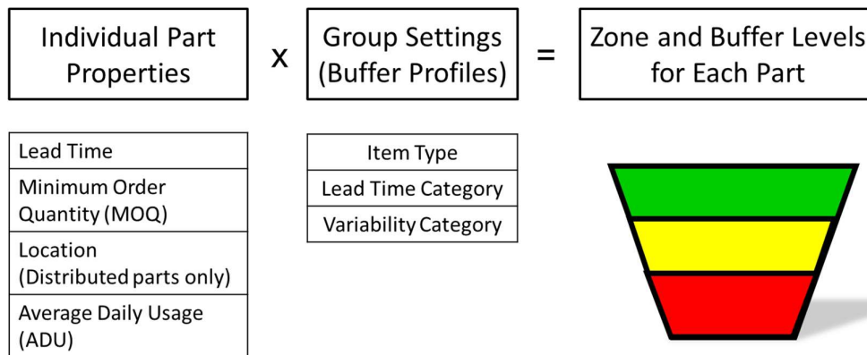
Figure II-VI: Parameters required to size DDMRP stock buffers (Ptak and Smith, 2016)
