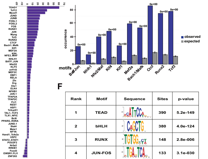
z score TFAD4_Day6_8156 peaks
