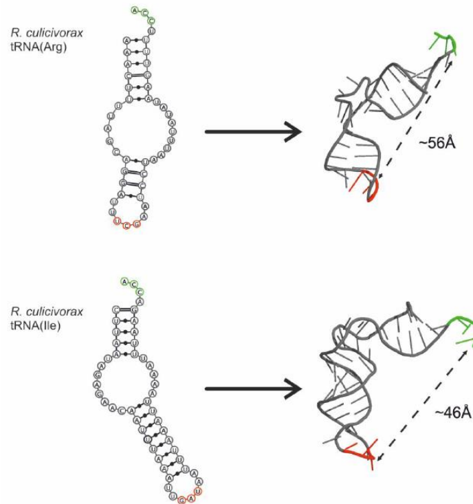
Figure 8: Structure prediction of mt tRNA Arg and mt tRNA Ile from R. culicivora .
