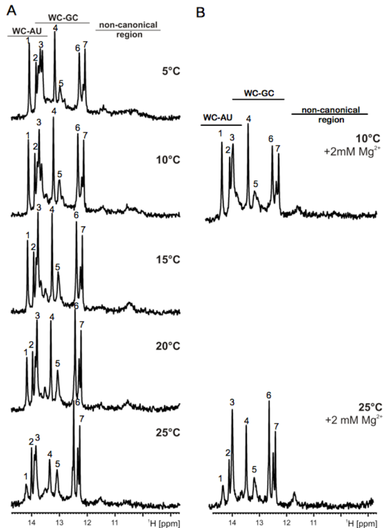
Figure 30: 1 H spectra of mt tRNA Arg measured by NMR spectroscopy.
