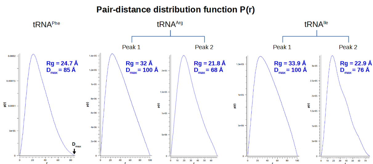
Figure 36: Pair-distance distribution functions of Scd tRNA Phe , Rcu tRNA Arg , and Rcu tRNA Ile . Pair-distance distribution functions, derived from SAXS curves indicating R_g and D_{\max} for yeast tRNA Phe , Rcu tRNA Arg from two populations (peak 1 and peak 2) and Rcu tRNA Ile from two populations (peak 1 and peak 2).
