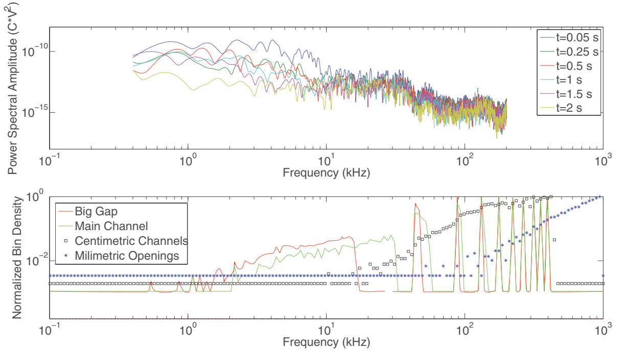
Figure A.1. Figure showing the frequency ranges where the different size effects are present. Top: Several power spectral distributions recorded during the experiment. Bottom: Curves represent the different size effects and the response of the plate modes.
