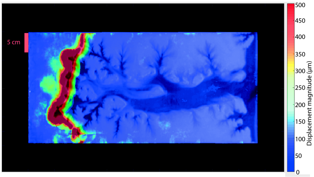
Figure 5.2: Incremental displacement map between the snapshots before and after an acoustic emission. The displacement magnitude map (for a time step of 8 ms between two images) is obtained by following the expression \|u\| = \sqrt{u_x^2 + u_y^2} where u_{x,y} shows displacements in x and y axes. See the section 5.3 for more details.
