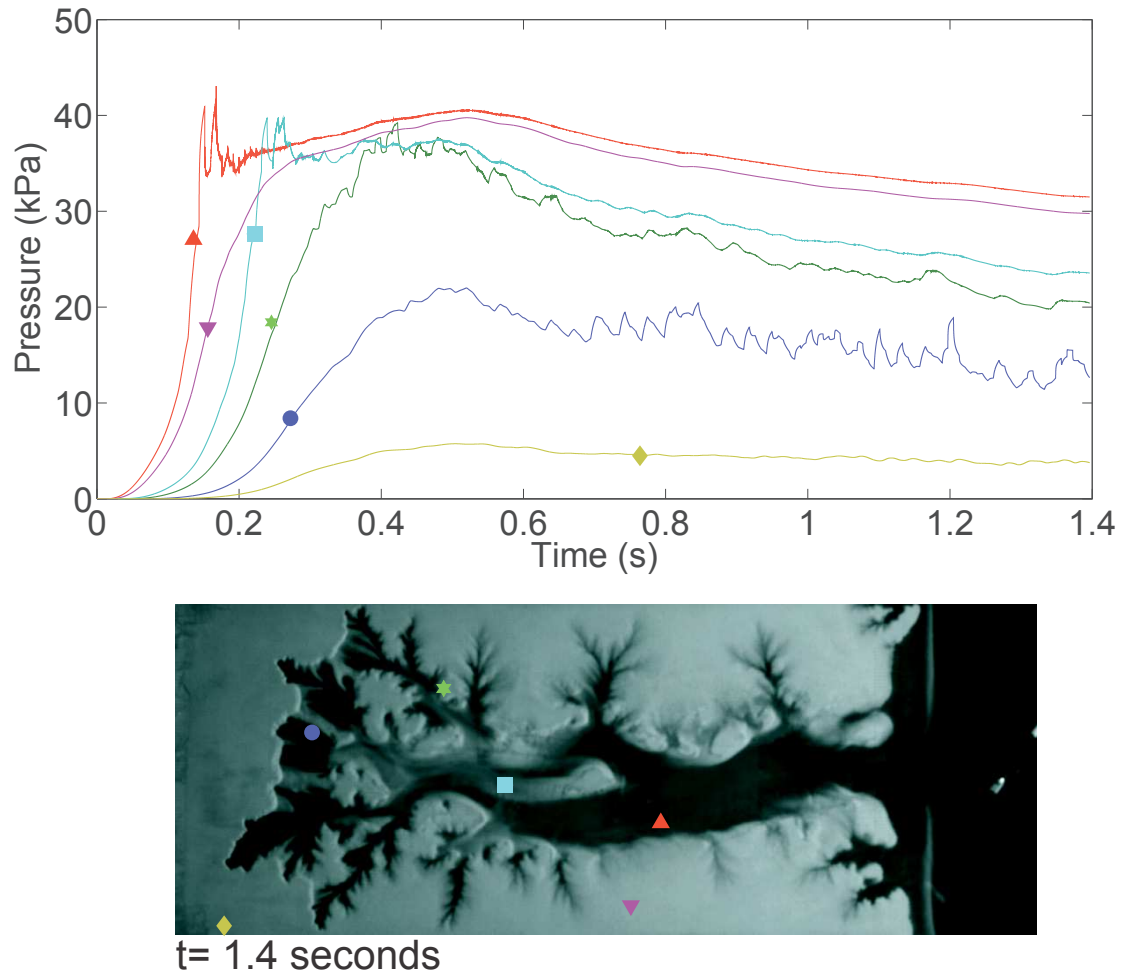
231 Figure 5. Pressures inside the Hele-Shaw cell, pressure evolution on different points marked on the cell are 232 presented
