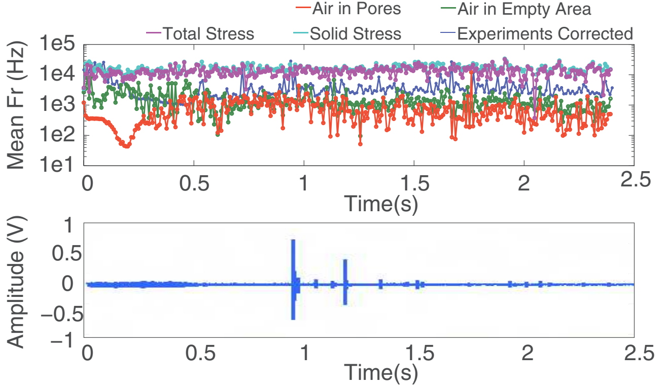
Figure 6. The comparison of the mean frequency evolution inside the cell. Top: Mean frequency vs time for different stress contributions (simulations) in comparison with the mean frequency vs time obtained from experimental data. Bottom: The signal experimentally recorded on the plate during the air injection experiment.
