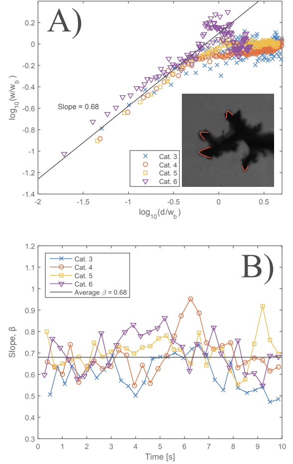
FIG. 8. A) The finger thickness w plotted in a log-log plot as function of the distance d from the finger tip. The data shown is the average of about 50 measurements in time for each experiment, averaged again for each category. The data is collapsed by the finger thickness at the base of the tips w_b found as the average finger thickness where w has reached a more or less constant level, which seems to be a typical length scale for the tip region. The finger thickness at the base of the tips is found as. The average slope at different times during several experiments is \beta = 0.68 , indicating a more rounded shape of the tips. In the inset: Snapshot of typical finger tips together with profiles corresponding to \beta = 0.68 (red lines). B) The slope \beta averaged per category as function of time during experiments. The plot shows that the slope for the tip profile fluctuates around \beta = 0.68 over time during the experiments, suggesting that the tips are more rounded than cusp-like at all times.
