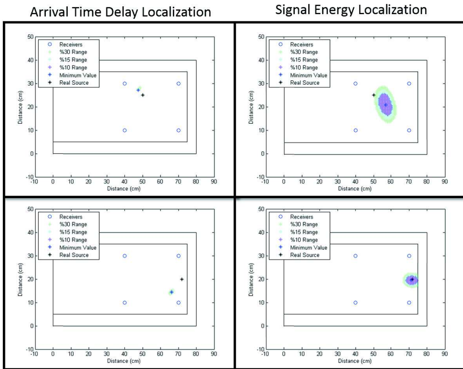
Figure 3: Validation of the Localization Methods using a Steel Ball. Figures on the left column shows localization result using the arrival time delay. Figures on the right column shows localization result using the signal energy.
