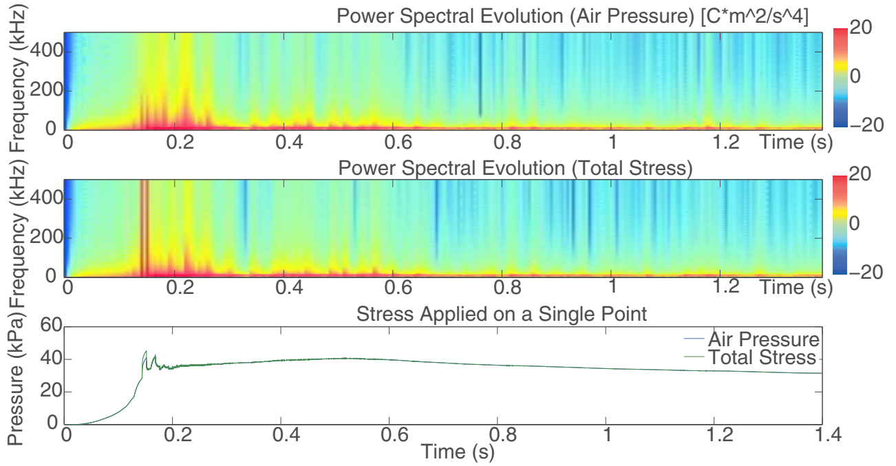
Figure 7. Power spectral evolution of the Lamb waves on the plate compared with the different types of loading.
