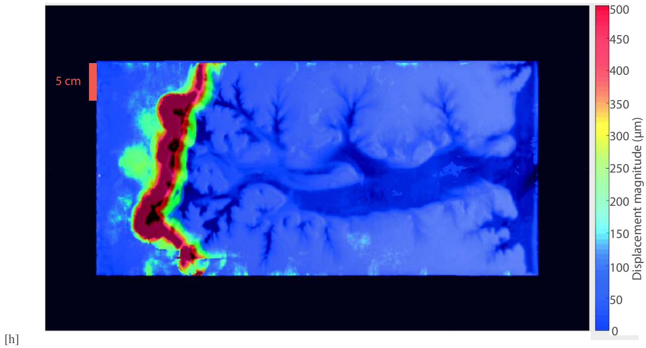
Figure 3. Displacement magnitude field obtained using the images at the start and at the end of an acoustic event. The red bar shows a distance of 5 cm. The colorbar shows the displacement occurred during a time step of 8 ms
