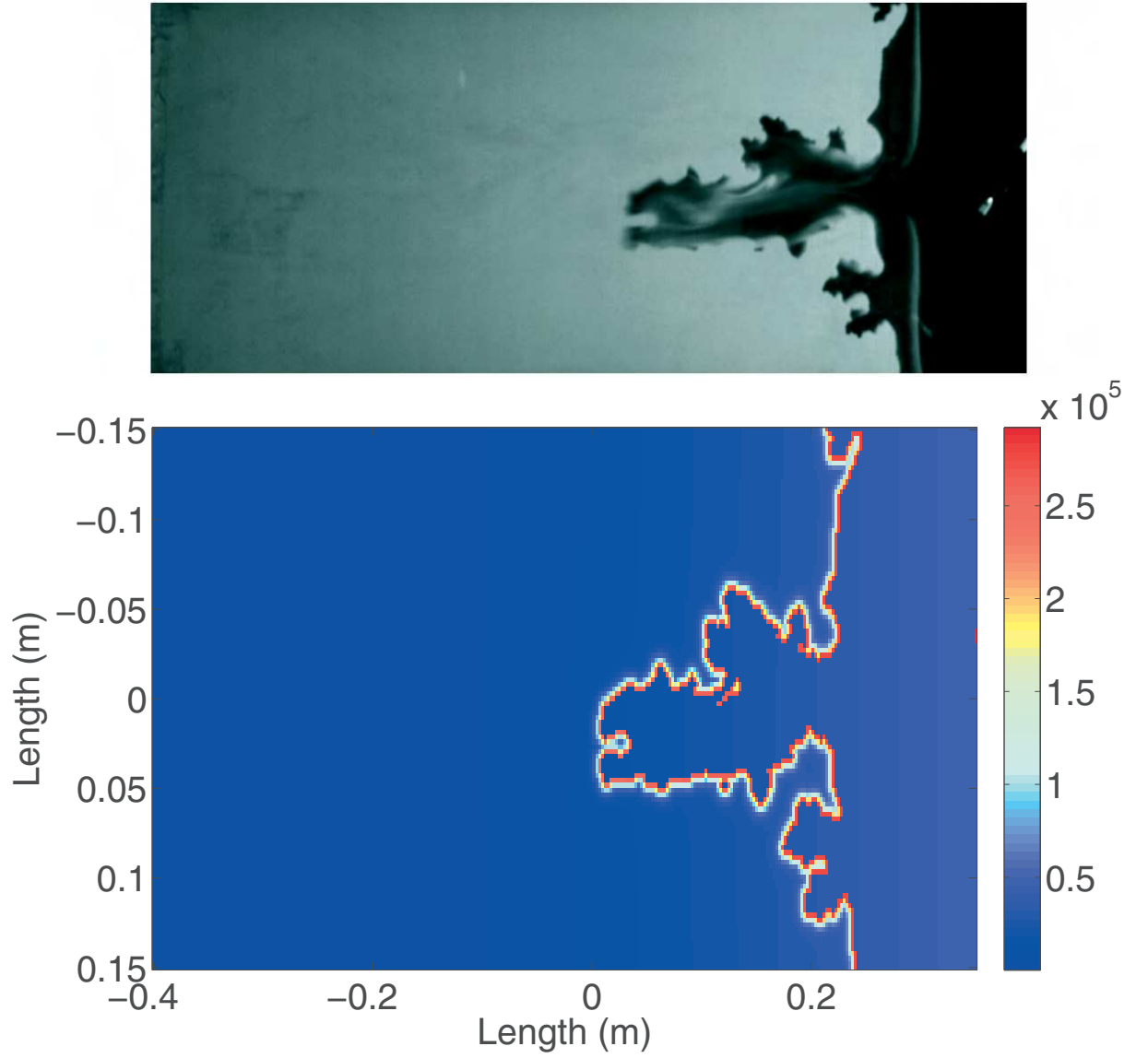
186 Figure 3. Hele-Shaw Cell during injection t = 0.16 s. Colorbar shows the pressure applied on the glass 187 plate in Pa.
