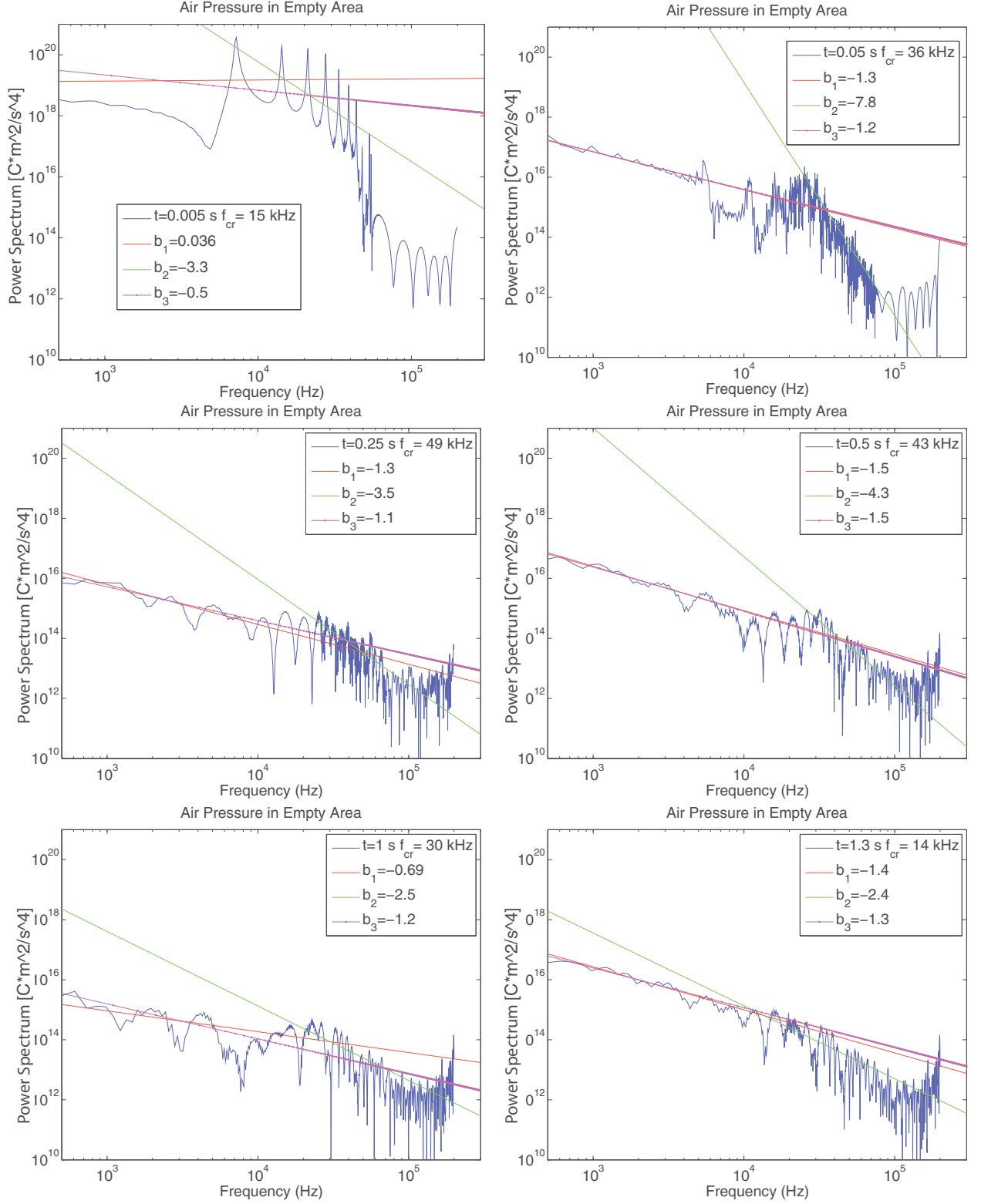
Figure 10. Power law evolution and comparison of power spectra due to the air pressure in empty channels
