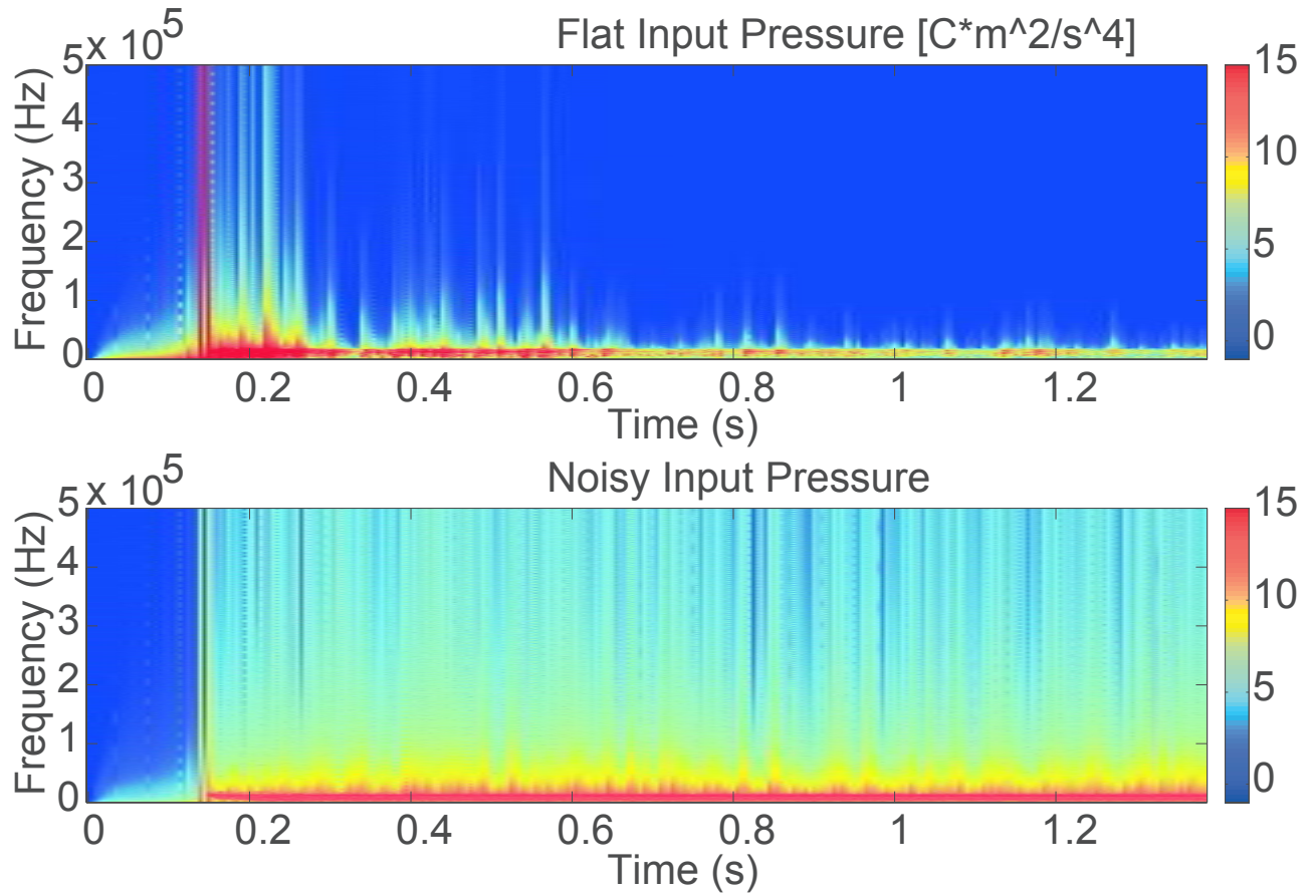
Figure 8. Comparison of two different spectrogram. Top: Spectrogram when the input pressure is flat. Bottom: Spectrogram when Gaussian noise is applied to the air input pressure.
