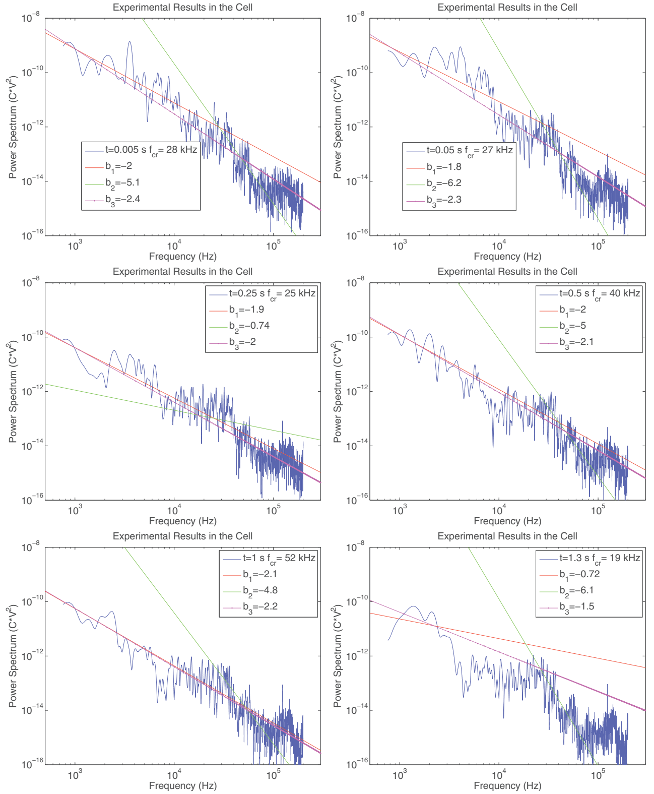
Figure 14. Power law evolution and comparison of experimental power spectra due to the total stress
