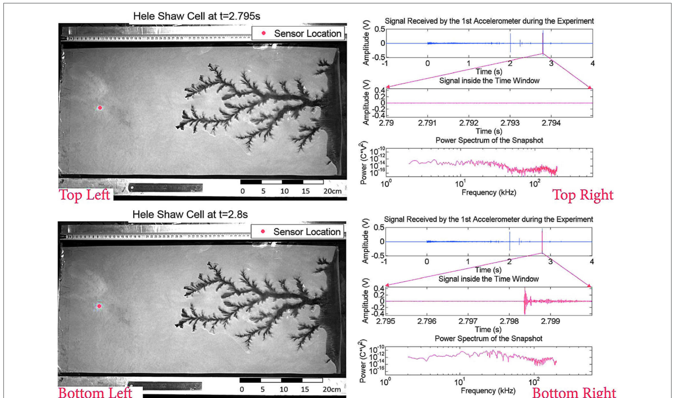
FIGURE 10 | Optical (Left) and acoustic (Right) experimental recordings just before (Top) and during (Bottom) an aftershock like event. The red dot on the left image illustrates the sensor location where the signal on the right is recorded. Top Right: Acoustic signal recorded throughout the entire experiment. The red strip (time window of 0.005 s) corresponds to the snapshot that the image (Left) and power spectrum (Right) occurred at.
