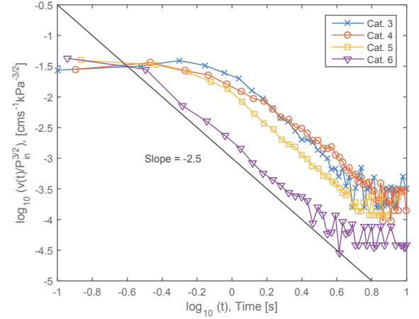
FIG. 10. Log-log plot of the finger tip velocity v(t) as function of time, averaged per category. The data is collapsed along the ordinate axis by dividing v(t) by P_{in}^{\frac{3}{2}} , where P_{in} = 64, 110, 134 and 213 kPa, for category 3, 4, 5 and 6 respectively. The initial constant plateau correspond to the period with linear growth over time, which then crosses-over to a declining slope close to -2.5 (dashed line) for all the categories. The slopes show that the decay in growth velocity follows a power law equation with time.
