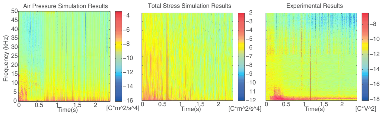
Figure 9. Power spectral distribution of the signals in different time steps. The contributions of different types of sources inside the Hele-Shaw Cell are indicated on the plot.
