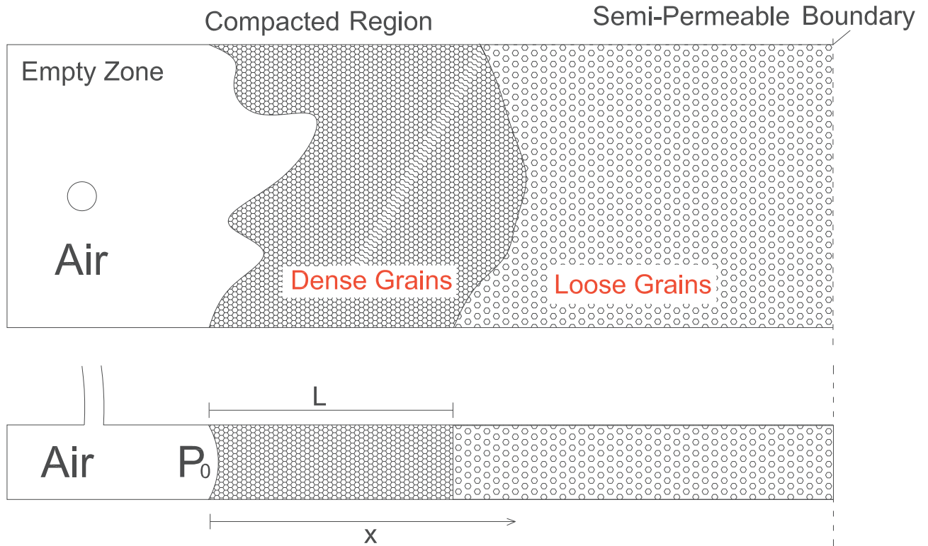
Figure 1. Compaction zone in the Hele-Shaw cell. As the air pushes grains, compacted zone with a length L occurs. Following this zone exponential decrease along the length x on the density of the grains (down to the undeformed phase) is presented.
