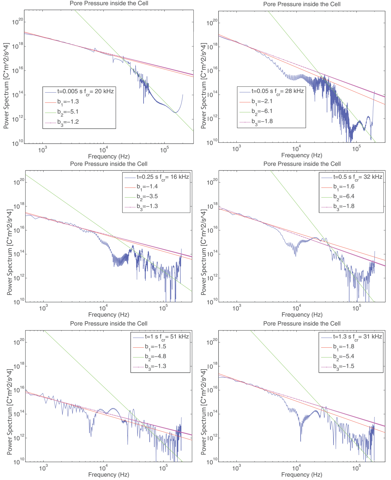
Figure 11. Power law evolution and comparison of power spectra due to the air pressure in pores
