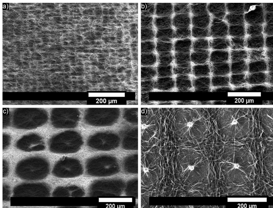
Figure 16 : Effect of the distance L between conducting 20\text{ }\mu\text{m} -in-diameter block and height H=60\text{ }\mu\text{m} : (a) downside view of the scaffold showing microgrids with block separation L=0.33H=20\text{ }\mu\text{m} after peeling from the collector, (b) downside view (after peeling the scaffold from the collector) of the scaffold with L=1.67H=100\text{ }\mu\text{m} , (c) downside view with L=3.67H=220\text{ }\mu\text{m} , (d) topside view of the collector after fiber deposition with L=3.67H=220\text{ }\mu\text{m} . Scale bars= 200\text{ }\mu\text{m} . Reprinted with permission from [90].
