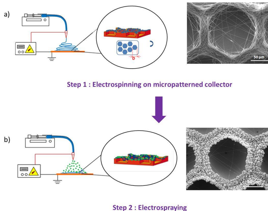
Figure 50: The two step processes: a) Electrospinning onto a micropatterned collector; b) Electro spraying onto the thin layer of nanofibers deposited onto a micropatterned collector
