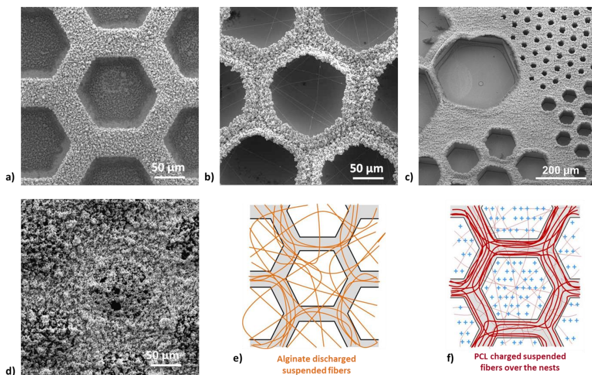
Figure 51: a) SEM image of a hydroxyapatite electrospray deposition onto a honeycomb micropatterned collector without electrospun fibers; b) SEM images of bi-layer electrospun/electrospray PCL/HA membrane onto honeycomb micropatterned collector; c) Same conditions as c) but at another scale showing different honeycomb pattern sizes; d) SEM images of a bi-layer electrospun/electrospray Al/HA membrane onto a honeycomb micropatterned collector
