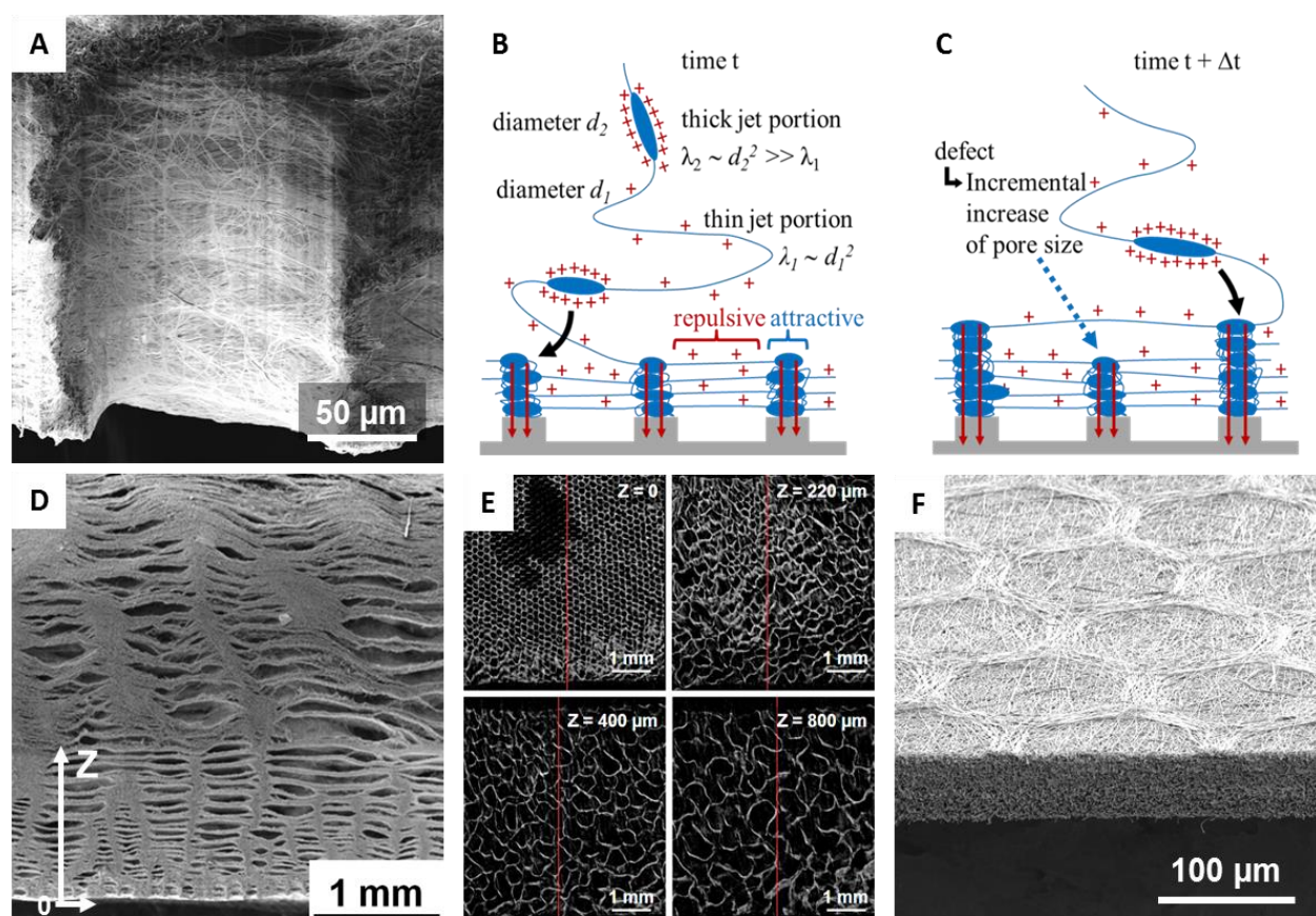
Figure 44: A) SEM image of a porous column with controlled pore size ( D = 160 \mu\text{m} ) in a PCL scaffold. B) Proposed mechanism for the construction of porous columns with controlled pore size C) Proposed mechanism for the merging of two columns. D) SEM image of the cross-section of a PCL scaffold (1 hour, D = 160 \mu\text{m} ). E) MicroCT images showing 4 slices at different Z values of a thick PCL honeycomb structure. F) SEM image of a thin PLA honeycomb structure (1 hour, D = 160 \mu\text{m} ). Videos of 3D micro-CT pictures can also be viewed in the Supplementary Data.
