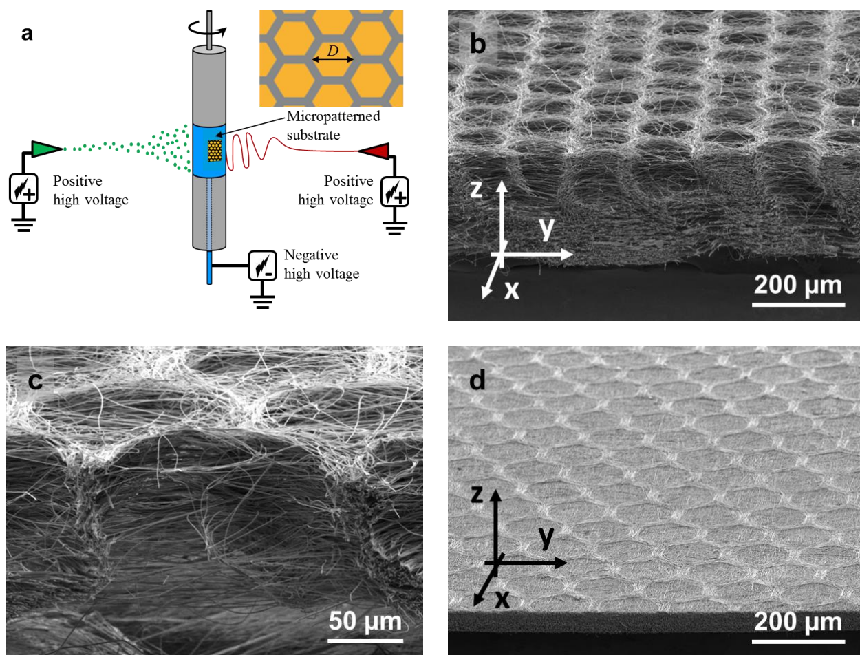
Figure 64: (a) Schematic of the process. The diameter D of the honeycombs was 40 \mu\text{m} , 80 \mu\text{m} , 160 \mu\text{m} or 360 \mu\text{m} . The width and the height of honeycomb walls were respectively 20 \mu\text{m} and 60 \mu\text{m} . (b) 3D columnar structures obtained for D = 160 \mu\text{m} after 1 hour of production. (c) 3D columnar structure obtained after 15 minutes of production. (d) Fibrous structure obtained with the same operating conditions and time of production than for (b) but without electrospaying. No internal 3D microstructure can be achieved in this case.
