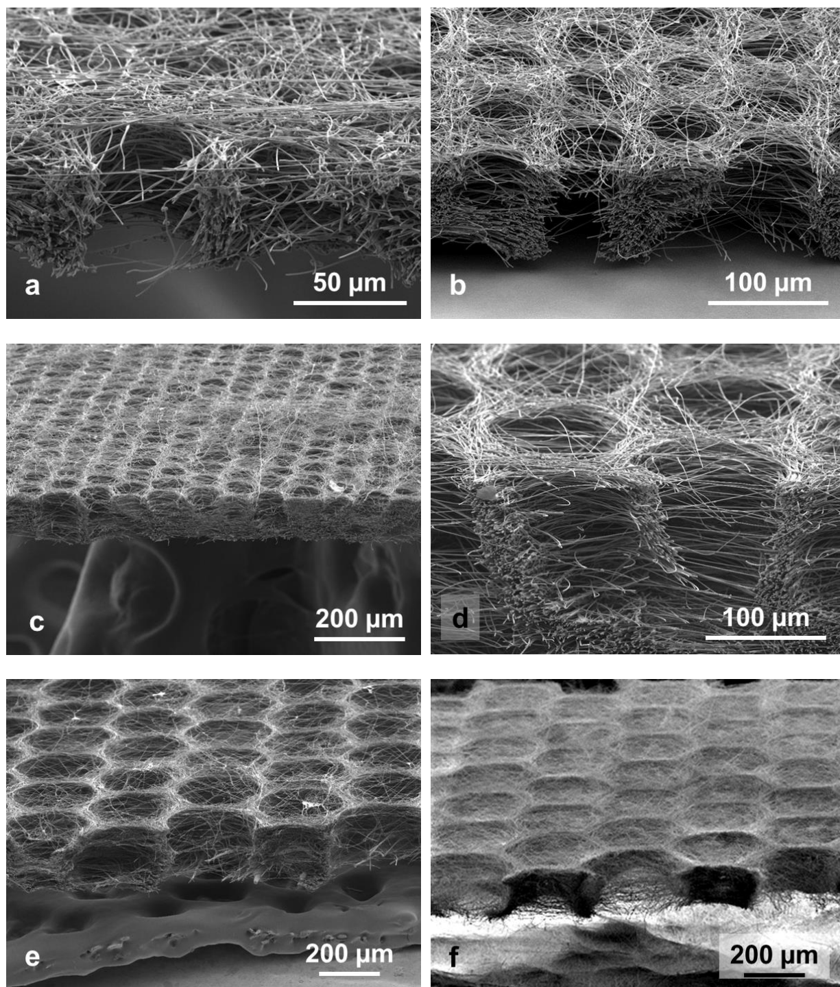
Figure 68: SEM pictures of various 3D constructs with electrospun PLA nanofibers and electrosprayed PEO microparticles showing their cross-section and the surface which was in contact with the collector. (a) D = 40 \mu\text{m} , (b and c) D = 80 \mu\text{m} and (d) D = 160 \mu\text{m} . (e and f) D = 360 \mu\text{m} .
