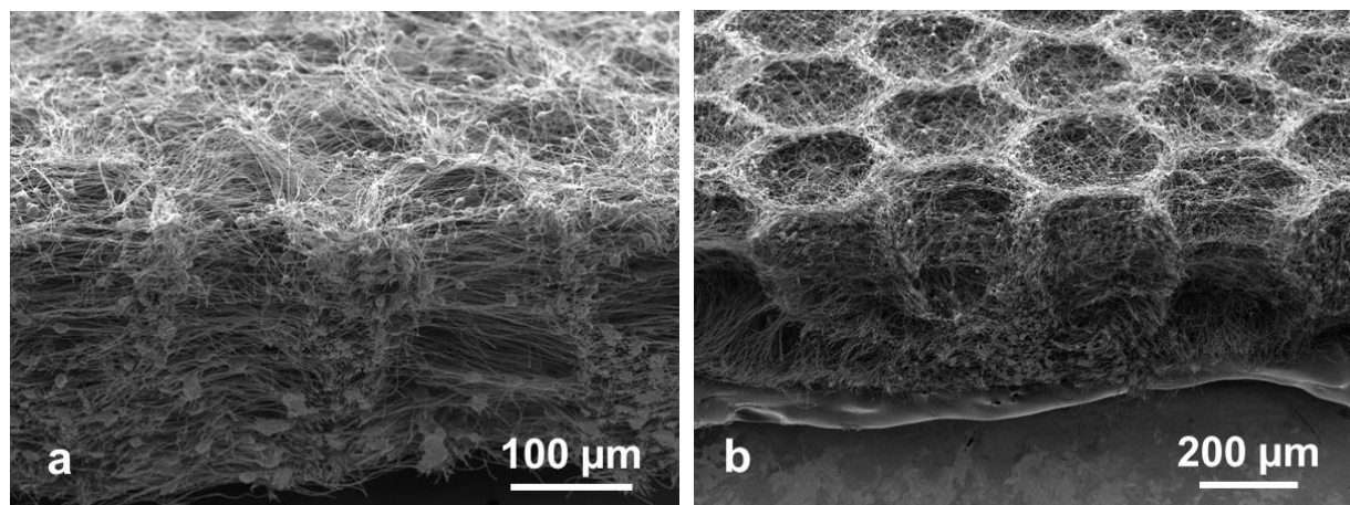
Figure 69: SEM pictures of 3D constructs with electrospun PLA nanofibers and electrosprayed PCL microparticles showing their cross-section and the surface which was in contact with the collector. (a) D = 160 \mu\text{m} , (b) D = 360 \mu\text{m} .
