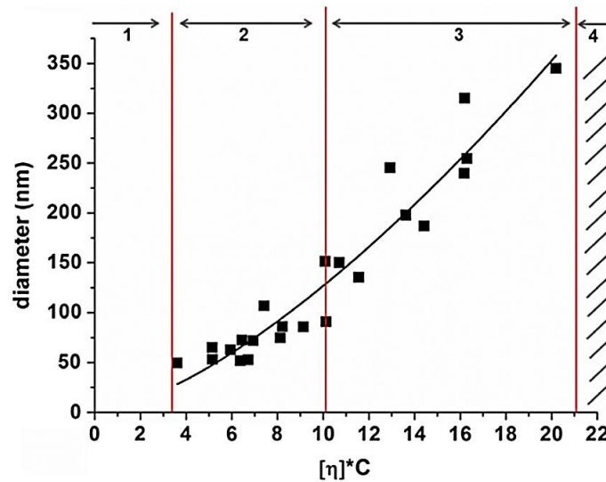
Figure 7: Variation of fibers average diameter with [\eta]*C (■): zone 1: electro spraying, zone 2: beaded electro spun fibers, zone 3: bead-free electro spun fibers and zone 4: no electrospinning.
