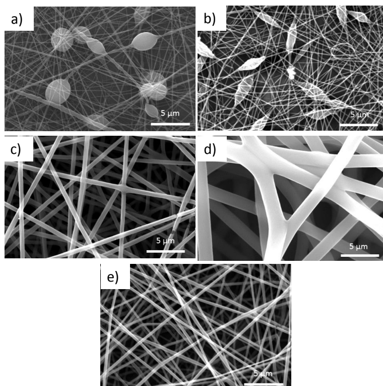
Figure 31: SEM images of different PLA solutions: a) 7% PLA in 70/30 (V/V) DCM/DMF; b) 8% PLA in 70/30 (V/V) DCM/DMF; c) 8% PLA in 50/50 (V/V) DCM/DMF; d) 10% PLA in 70/30 (V/V) DCM/DMF; e) 8.2 % PLA in 50/50 (V/V) DCM/DMF
