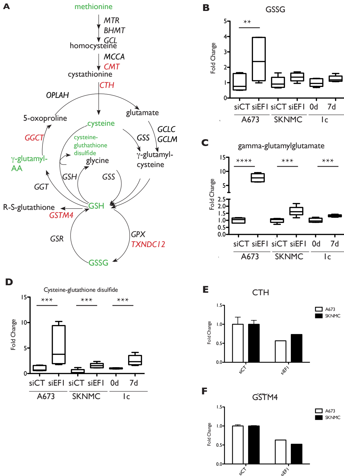
Figure 6: The glutathione pathway. A) Silencing of EF1 expression in Ewing' sarcoma cells appears to be associated with increased glutathione synthesis and turnover/recycling. B) Elevated levels of GSSG, glutathione degradation/turn-over products such as C) gamma-glutamylglutamate and such as the biochemical marker of oxidative stress D) cysteine-glutathione-disulfide. E) EWS-FLI1 upregulates the expression of enzyme CTH and F) GSTM4.
