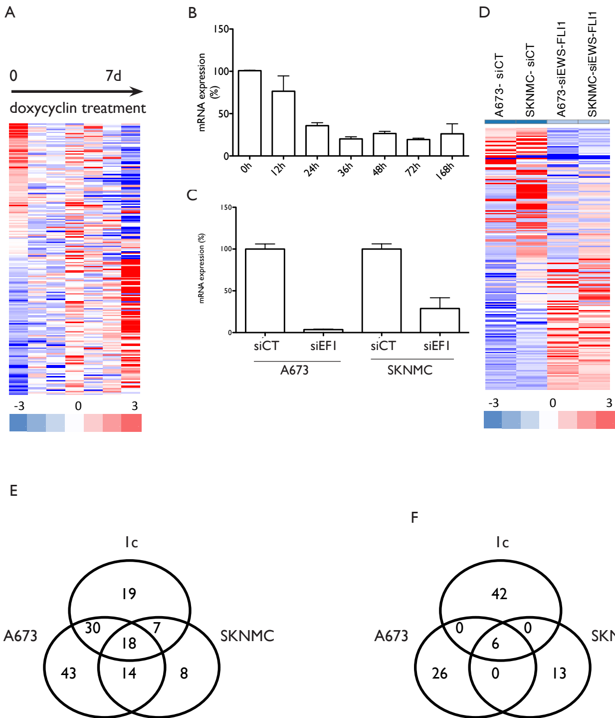
Figure 1. Metabolite profile of Ewing' sarcoma cell lines, inhibited by EWS-FLI1. A) Heat map showing 254 metabolites in lysates from five replicates from EWS-FLI1 doxycyclin inducible cell line 1C in a time-series experiment for 7 days. A shift of metabolites was observed upon EWS-FLI1 inhibition that became more profound in later time points. B, C) Relative expression of EWS-FLI1 in the 1C time series B) and the A673 and SKNMC inhibition C). D) Heat map showing 433 metabolites in lysates from five replicates from the Ewing' sarcoma cell lines A673 and SKNMC inhibited by siRNA for EWS-FLI1. E, F) Venn diagram comparing the 218 common metabolites in 3 different cell lines upon EWS-FLI1 inhibition. The venn diagrams indicate the number of metabolites that are significantly ( P < 0.05 ) upregulated E) or downregulated F). The overlap shows the common metabolites in all three cell lines. The highest common metabolites in the three cell lines are part of the kynurenine pathway, the glucose pathway, the cysteine glutathione pathway, the fatty acid synthesis pathway and the N-glycosylation pathway.
