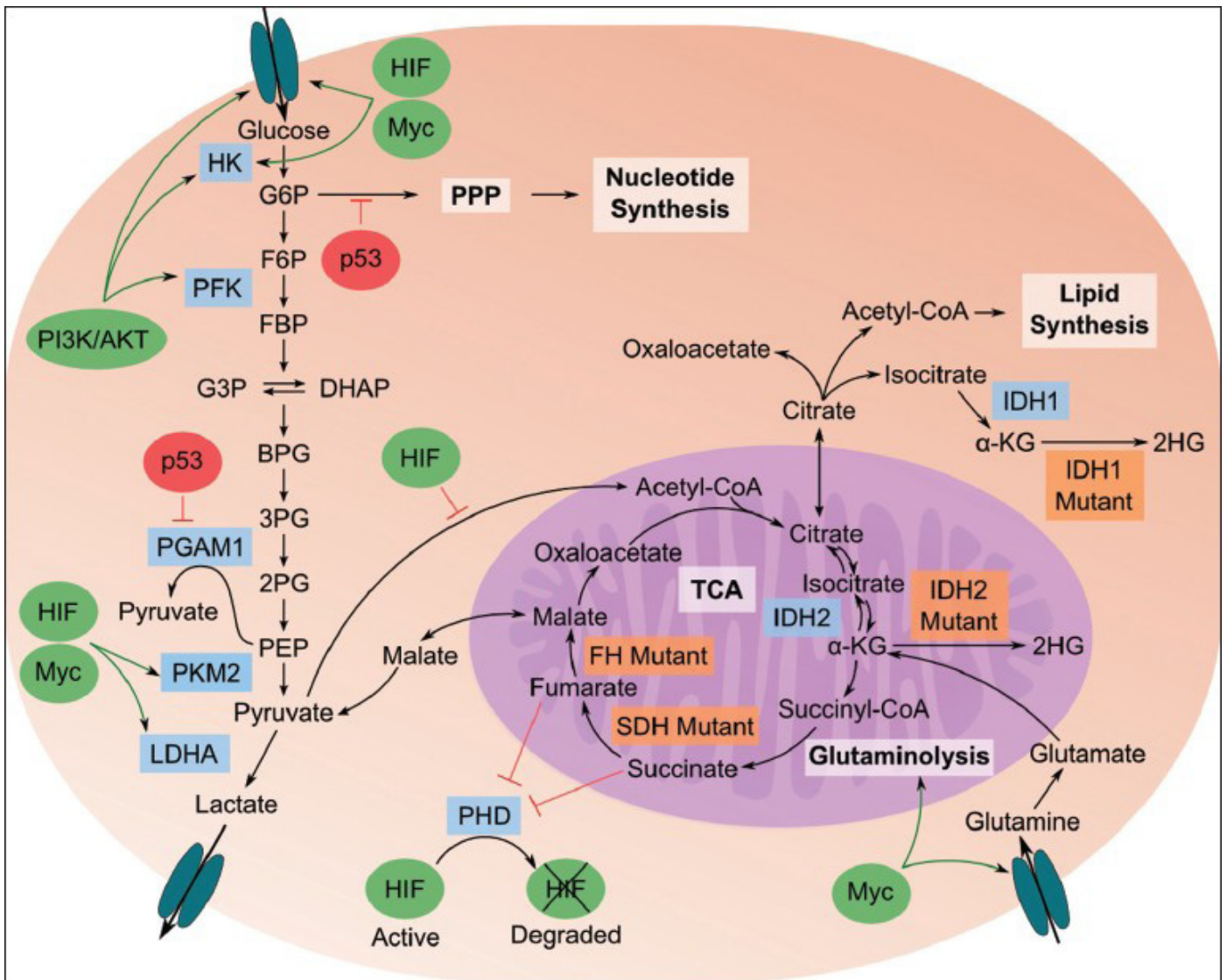
Figure 5: Tumor metabolism: Relationships between metabolites and genes in cancer cells. Glycolysis breaks down glucose into pyruvate, which is then turned to lactate, as flux through TCA cycle is down regulated in cancer cells. Pathways branching off of glycolysis, such as the pentose phosphate pathway, generate biochemical building blocks to sustain the high proliferative rate of cancer cells. Blue boxes are enzymes important in the metabolic transformation to support the cancerous phenotype; orange boxes are enzymes that are mutated in cancer cells. Green ovals are oncogenes that are up-regulated in cancer; red ovals are tumor suppressors that are down-regulated in cancer. Figure adapted from Vermeersch et al, Carcinog, 2013,
