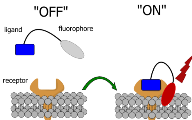
Figure 24. Principle of the turn-on detection of GPCRs.
