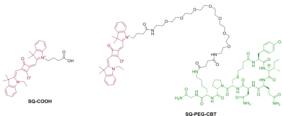
Figure 34. SQ-COOH and the target carbocyanine derivative SQ-PEG-CBT.
