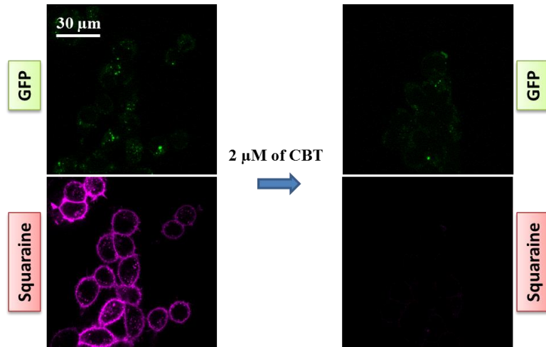
Figure 38. Confocal images of wtOTR cells with 10 nM of SQ-PEG-CBT before and after the addition of 2 μM of CBT.
