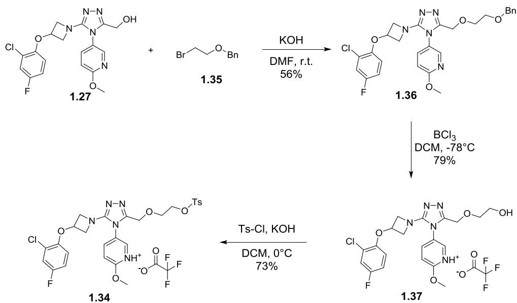
Scheme 8. Synthesis of the precursor 1.34 for 18 F labelling.
