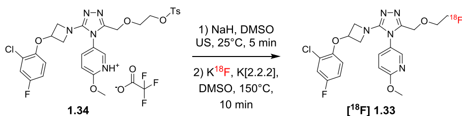
Scheme 10. Radiolabelling of 1.34 with 18 F.
