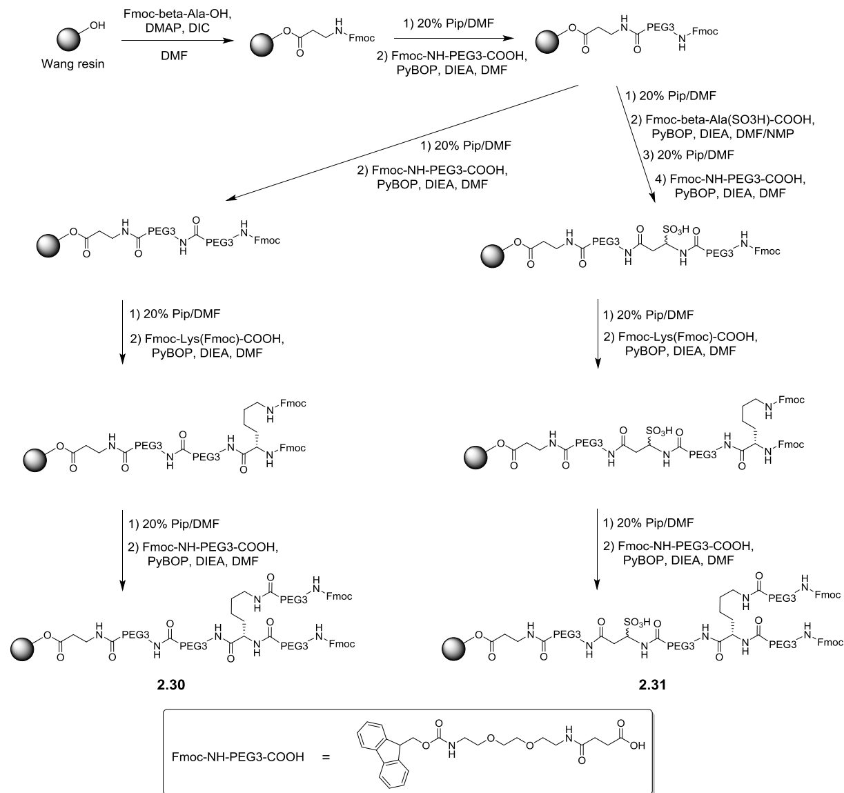
Scheme 20. Synthesis of branched chains 2.30 and 2.31 .
