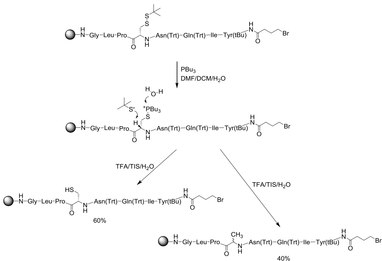
Scheme 2. Cleavage of the S -tert-butylsulfanyl protection group.
