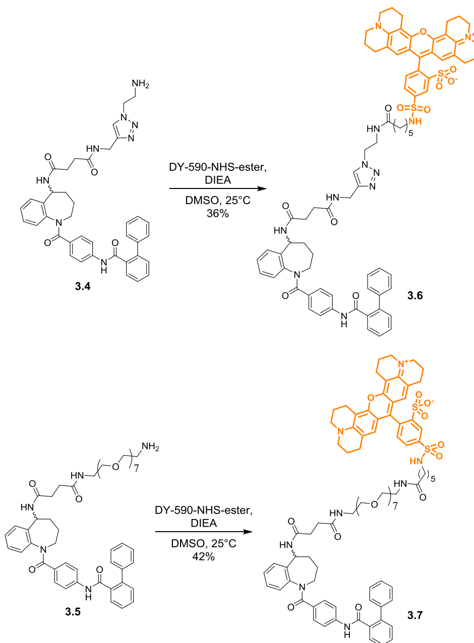
Scheme 24. Synthesis of DY-590 ® -labeled V 2 R ligands 3.6 and 3.7 .
