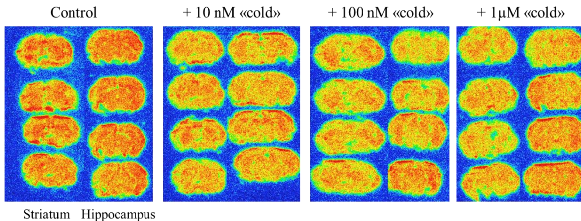
Figure 13. In vitro autoradiograms of rat brain sections incubated with [ 11 C]PF-3274167 and after competition with cold PF-3274167.
