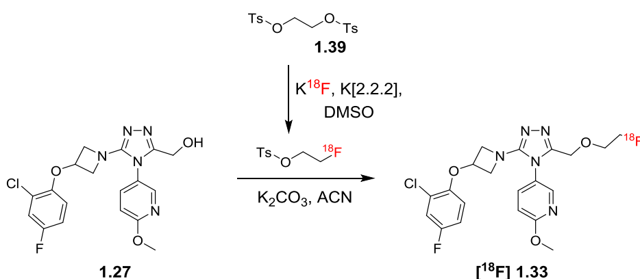
Scheme 11. Two-step labelling procedure for the introduction of 18 F.
