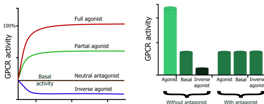
Figure 2. Schematic representation of the action of different ligands on a GPCR.
