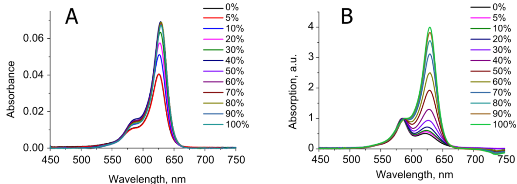
Figure 45. Absorption spectra of 200 nM 2.26 (A) and 2.27 (B) in increasing concentrations of MeOH in water.
