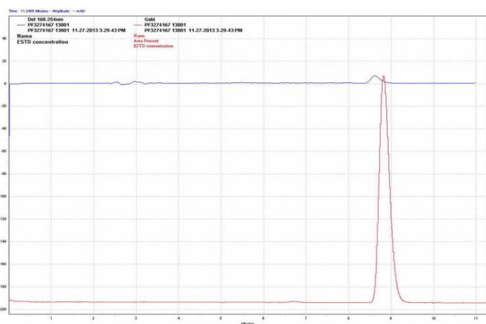
Figure 12. Radiolabelling of 1.27 and the quality chromatogram of final [ 11 C]PF-3274167 (UV absorbance at 254 nm in blue and radioactivity in red)
