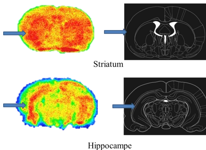
Figure 15. In vitro autoradiograms of rat brain sections incubated with [ 18 F] 1.33 .
