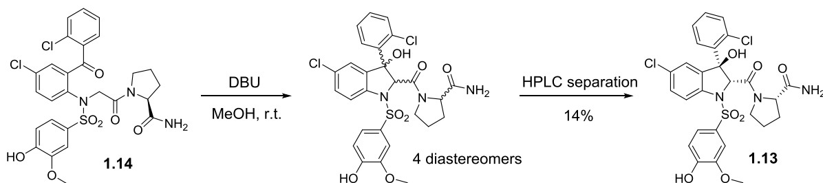
Scheme 6. Intramolecular cyclisation of 1.14 .
