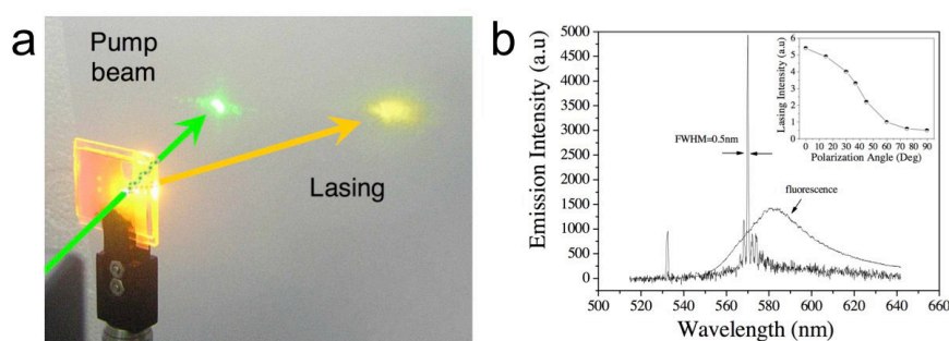
Fig. 7. a. Macroscopic view of lasing experiment. b. Fluorescence and lasing spectra from pyromethene dye-doped nematic liquid crystals. Discrete sharp peaks emerge from the residual spontaneous emission for pump energy of about 1.2 \mu\text{J}/\text{pulse} . The inset shows the dependence of the lasing intensity on the angle \theta between the linearly polarized light and the local nematic director orientation. Reprinted from Ref. 112 with
