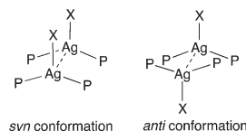
Scheme 7 Respective conformations of the ligands around the silver cations.
