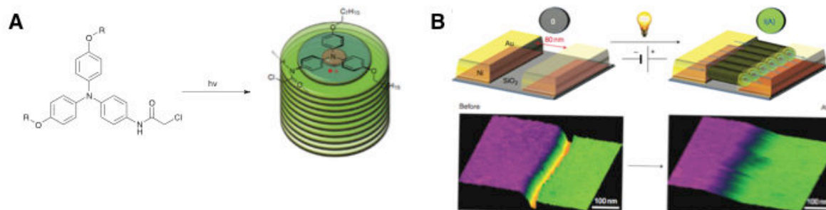
Figure 1 | Self-assembling triarylaminines reported by our group in 2010 1 (a). Assembly of the triarylaminines between two lithographically defined electrodes 2 (b).
