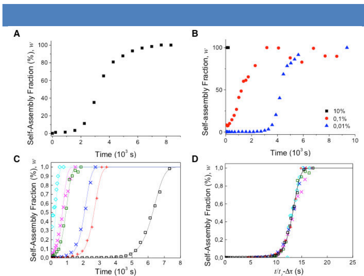
Figure 38 | Self-assembly kinetics as followed by NMR. Light-induced self-assembly after a 1s light pulse (a). self-assembly induced by seeding with preassembled molecules (b). Self-assembly induced by chemical oxidation fit with a master equation (c). Fit of the self-assembly kinetics with the master theory curve (d).
