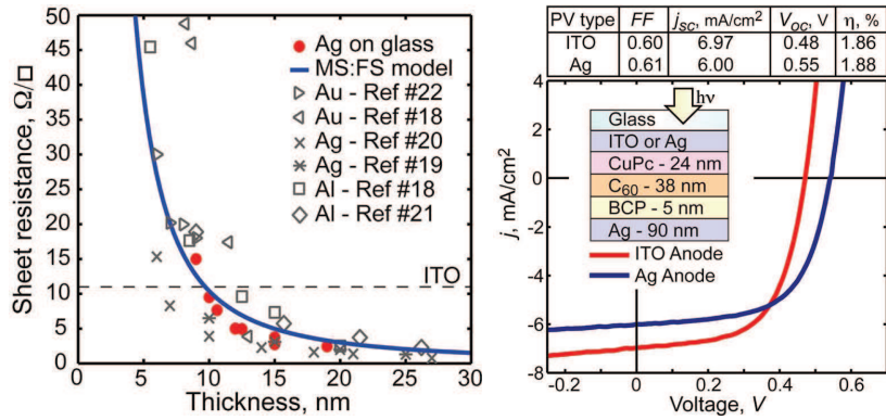
Fig. 1.5: Sheet resistance versus film thickness for thin Ag, Al and Au films compared to the sheet resistance of ITO (left) and IV characteristics of OPV devices under 106\text{mW}\cdot\text{cm}^{-1} illumination with 9\text{nm} Ag and 150\text{nm} ITO anodes [39]
