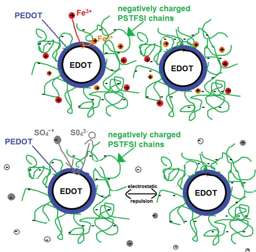
Fig. 2.38: Illustration of the decrease of the colloidal stability of PEDOT:PSTFSI due to the high concentration of Fe^{3+}/Fe^{2+} ions
