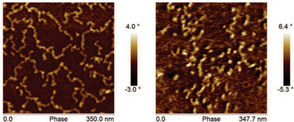
Fig. 6.8: AFM phase images of PSTFSI, M_W \approx 300\text{kDa} (left) and PMaTFSI, M_W \approx 80\text{kDa} (right) on a mica surface
