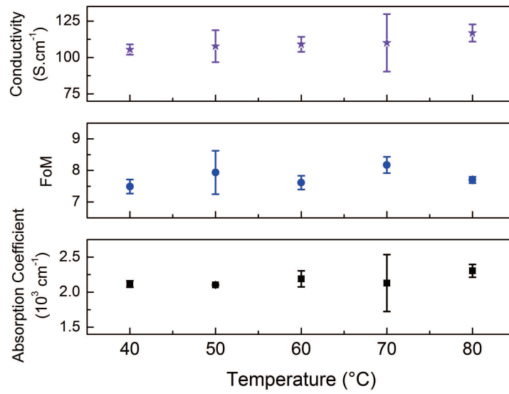
Fig. 3.18: Opto-electronic properties of PEDOT:PSTFSI films deposited by doctor blading at different temperatures with a constant blade speed of 10\text{mm}\cdot\text{s}^{-1}
