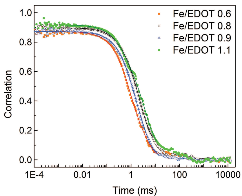
Fig. A.11: Correlation function of DLS measurements of PEDOT:PSTFSI dispersions synthesized with different concentrations of Fe(Tos)_3
