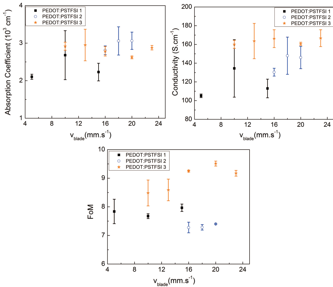
Fig. 3.16: Opto-electronic properties of PEDOT:PSTFSI films deposited by doctor blading at 70^\circ\text{C} with different blade speeds
