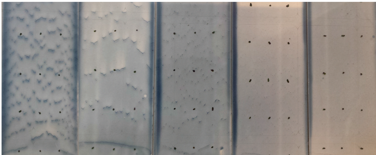
Fig. 3.17: PEDOT:PSTFSI films cast by doctor blading from a PEDOT rich dispersion with increasing blading speed from right to left
