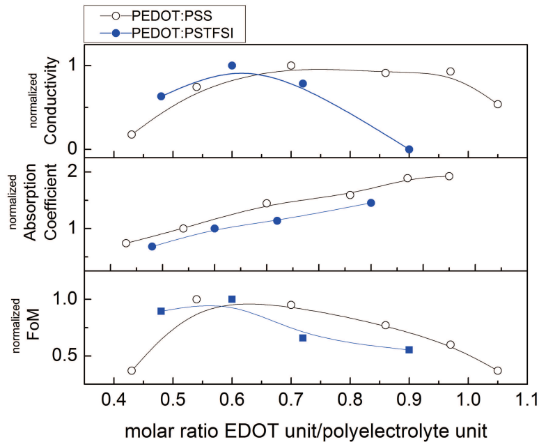
Fig. 2.22: Conductivity, absorption coefficient and FOM of PEDOT:PSS ( M_W(\text{PSS}) \approx 200\text{kDa} ) and PEDOT:PSTFSI ( M_W(\text{PSTFSIK}) \approx 300\text{kDa} ) as a function of the molar ratio EDOT/polyelectrolyte repeating unit, synthesized at 10^\circ\text{C} and magnetic stirring at 625\text{rpm}
