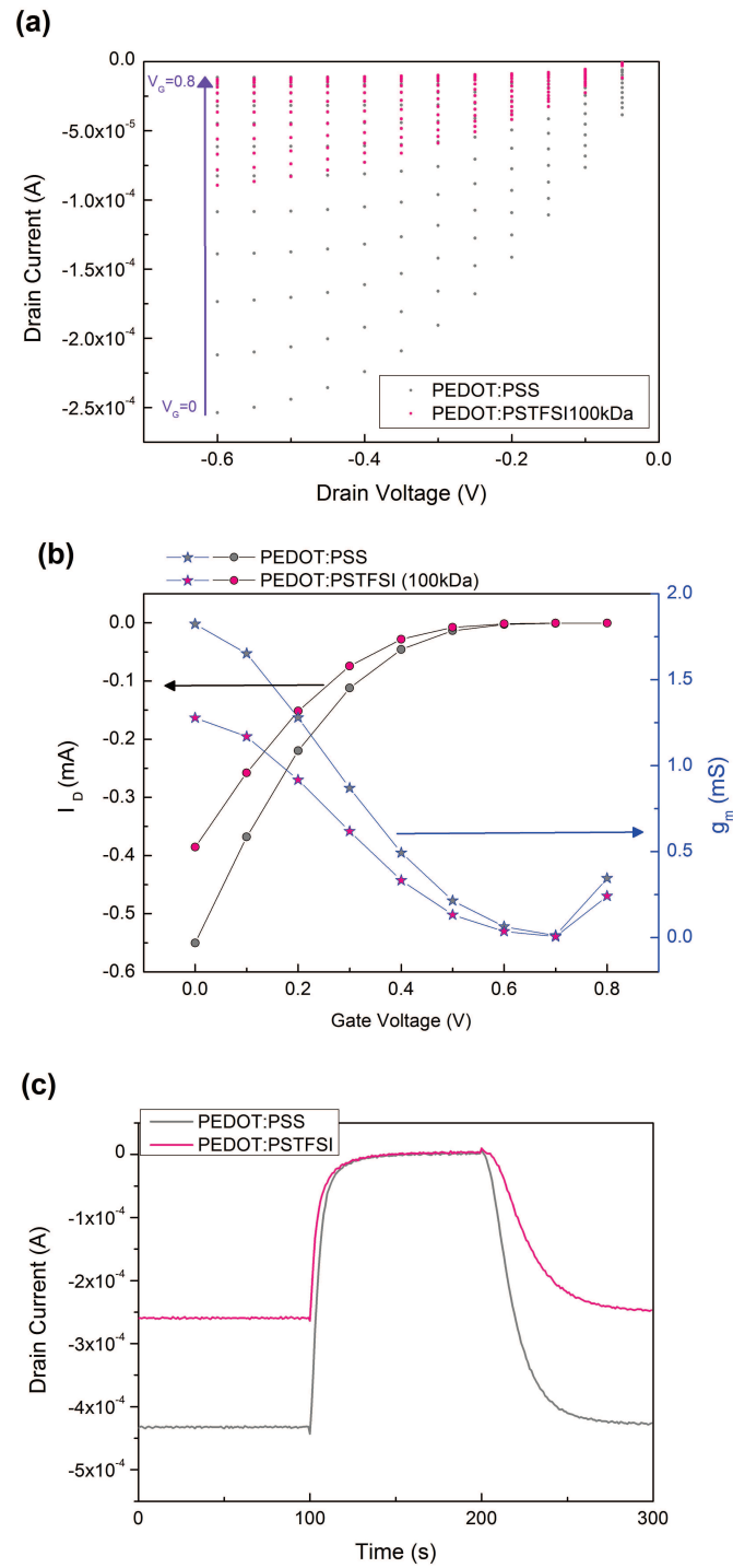
Fig. 5.7: a) I_D-V_D curve, b) I_D-V_G transfer characteristics, transconductance ( V_D=-0.8V ) and c) temporal response of the drain current of OECTs with a PEDOT:PSS or a PEDOT:PSTFSI ( M_W(PSTFSI)=100kDa ) electrode
