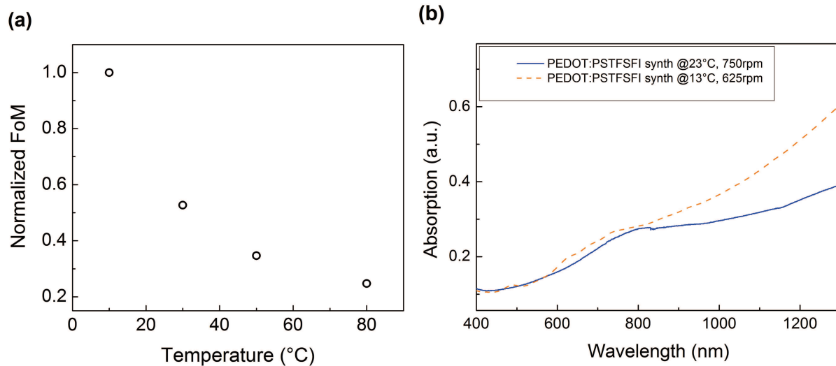
Fig. 2.49: a) Dependency of the FoM on the polymerization temperature and b) UV/Vis spectra of PEDOT:PSTFSI synthesized at 13°C and at 23°C
