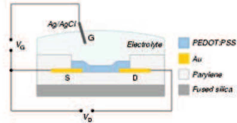
Fig. 5.6: Scheme of an OECT [15]
