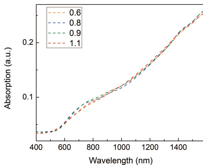
Fig. 2.42: UV/Vis spectra of PEDOT:PSTFSI synthesized with (NH 4 ) 2 S 2 O 8 and Fe(tosylate) 3 with Fe 3+ to EDOT ratios of 0.6 to 1.1, at 10°C, PSTFSIK 100kDa
