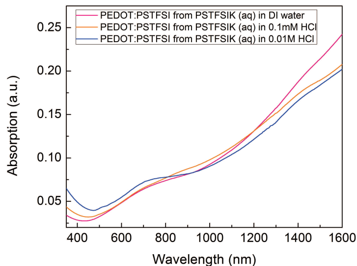
Fig. 2.26: UV/Vis spectra of PEDOT:PSTFSI films synthesized from PSTFSIK solutions with different concentrations of HCl; M_W(\text{PSTFSIK}) \approx 250\text{kDa} , PSTFSIK solution at 9\text{g.l}^{-1} , equivalent to 0.025\text{mol.l}^{-1} STFSIK units
