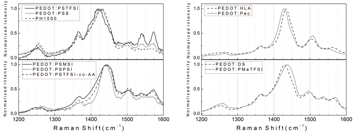
Fig. 6.5: Raman spectra of PEDOT:polyelectrolyte dispersions, excitation wavelength 532nm
