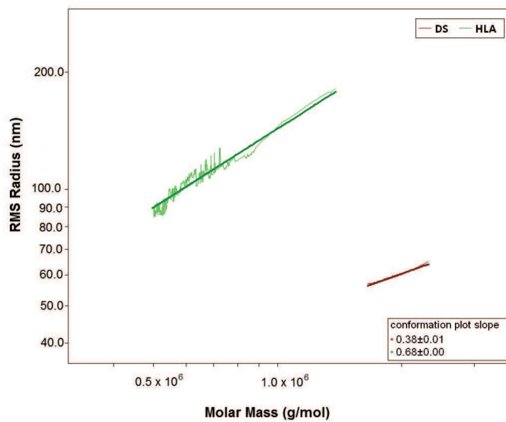
Fig. D.2: Conformation plot of dextran sulfate and hyaluronic acid, determined by size exclusion chromatography
