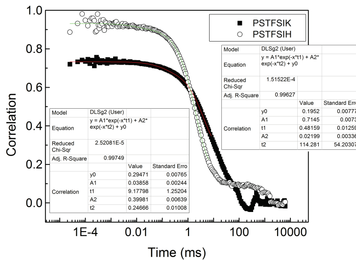
Fig. 2.8: DLS correlation function of aqueous PSTFSIK and PSTFSIH solutions, M_W \approx 350kDa
