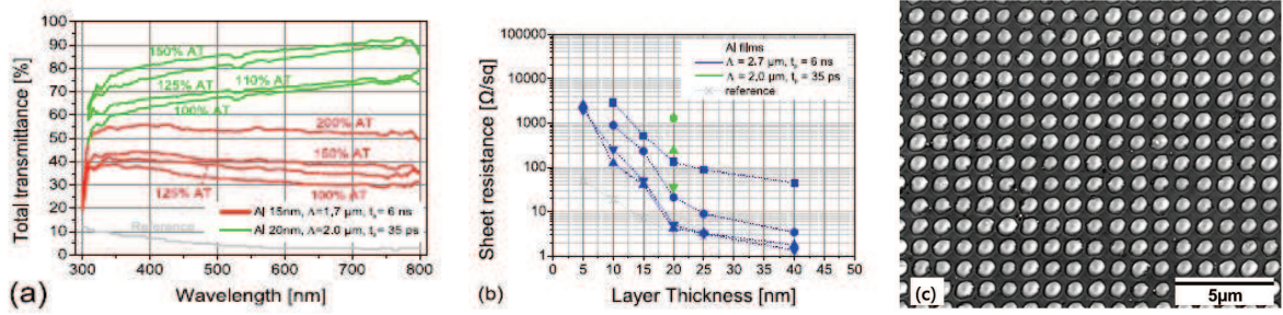
Fig. 1.8: a) Transmittance in the optical range, b) sheet resistance as a function of the film thickness and c) SEM image of a laser patterned Al film with a spatial pattern period of \Lambda=1.7\ \mu\text{m} [47]
