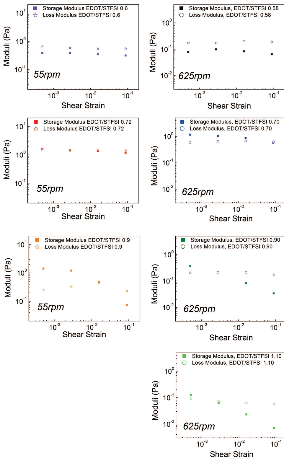
Fig. A.6: Storage and Loss Moduli as a function of shear strain at 10\text{rad}\cdot\text{s}^{-1} of PEDOT:PSTFSI with different EDOT to STFSI ratios and stirring at 55rpm and at 625rpm
