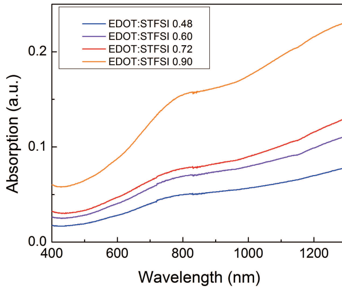
Fig. 2.14: UV/Vis absorption spectra of PEDOT:PSTFSI as a function of the molar EDOT to STFSI ratio, synthesis at 10° C 55rpm under N 2 , M W (PSTFSIK)≈250kDa
